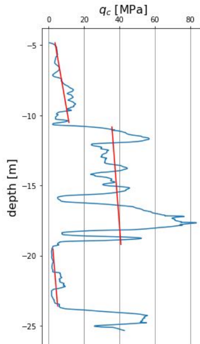
Figure 6.10: CPT DKP-9 including trendlines
