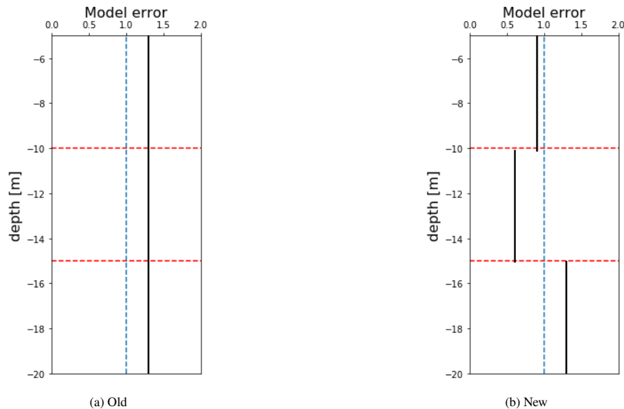
Figure B.1: Model error
