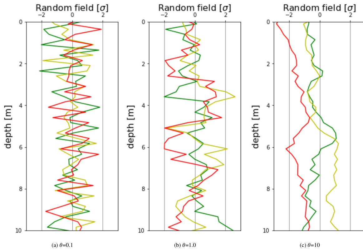
Figure A.1: Normalised random fields
