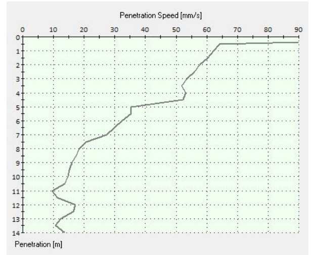
Figure 1.3: Example of v_p -z-curve
