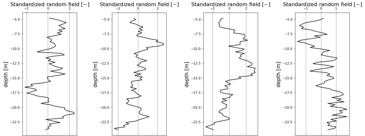
Figure B.2: Random field examples
