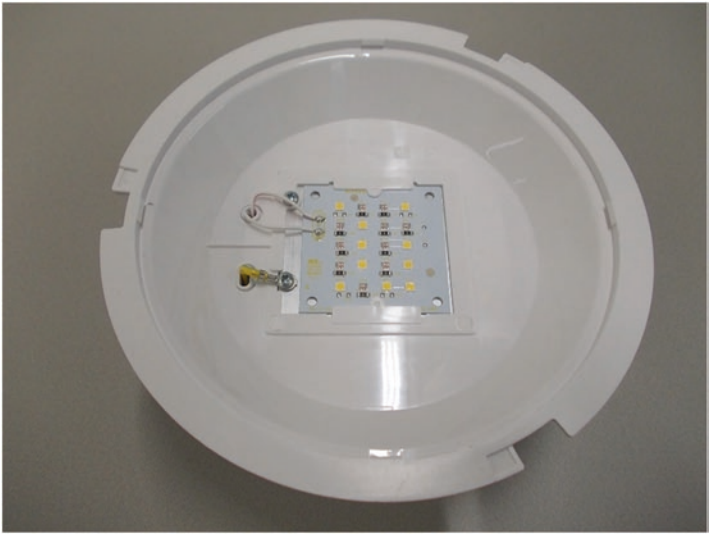
Fig. 7.19 Photo of carrier product with the diffusive flat exit window taken out
