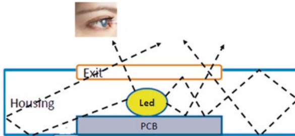
Fig. 7.17 Schematic diagram of light paths representing the view factor approach
