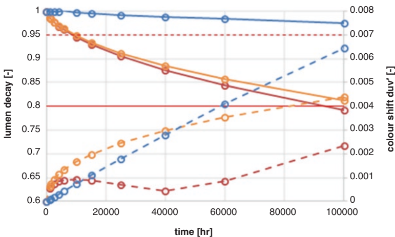
Fig. 7.23 Calculated uv' color shift (dotted line) and lumen decay (solid line) as function of (aging) time; LEDs 100 °C, PCB 90 °C, reflector & exit window 80 °C. Red: all parts aging; Orange: only LED aging; Blue all but LED aging
