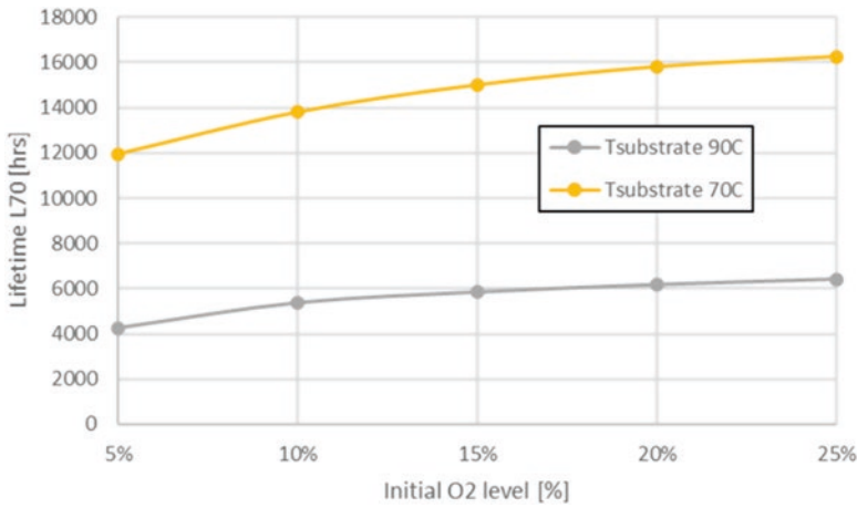
Fig. 7.15 Lifetime as a function of temperature and initial O 2 level
