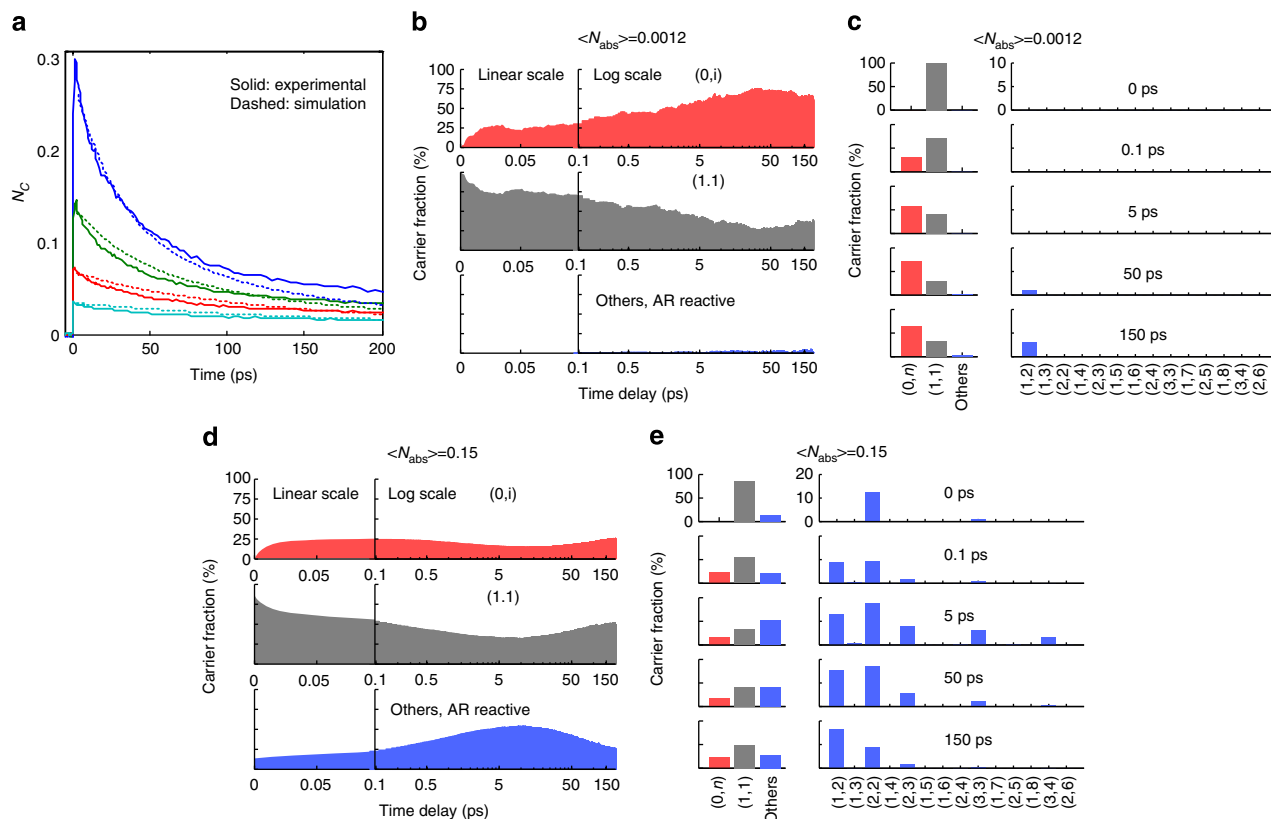
Figure 2 | Monte Carlo simulations of AR in QD solids. (a) Simulated (dashed line) and experimental (solid line) carrier decay traces with initial excitation density \langle N_{abs} \rangle from 0.15 to 0.019. N_c = 2 \langle N_{abs} \rangle is the total charge carrier density (electrons plus holes). (b,d) Charge carrier combinations (0,i; red shaded area), (1,1; grey shaded area) and others (AR reactive; blue shaded area) with (b) \langle N_{abs} \rangle = 0.0012 and (d) \langle N_{abs} \rangle = 0.15 on a lin-log timescale (the first 100 fs are on a linear timescale; subsequently a logarithmic scale is used). (c,e) Histograms of the MCDs for five delay times with (c) \langle N_{abs} \rangle = 0.0012 and (e) \langle N_{abs} \rangle = 0.15 . The same colour coding is used as in (b) and (d).
