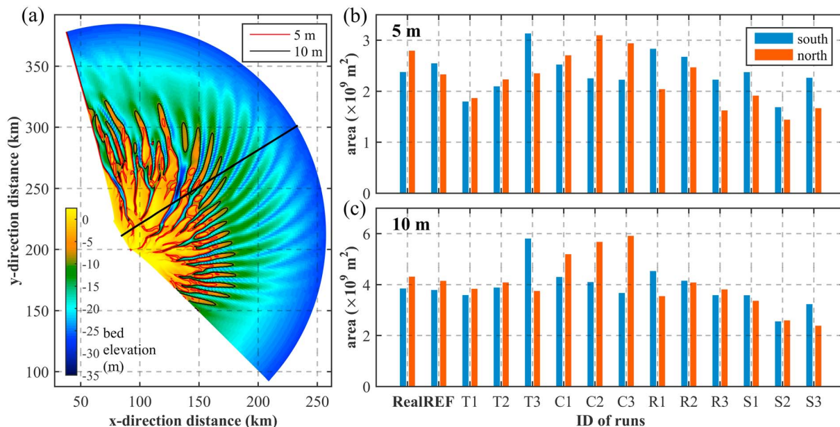
Figure 10. Comparison of the sand ridge areas between the real radial sand ridges and the numerical runs. (a) illustrates the method of calculating the areas of the southern and the northern sand ridges. The computational domain is divided into southern and northern halves from the middle radial line (see the black bold line). (b) and (c) illustrate the planar areas enclosed by the 5- and 10-m contour lines, respectively.
