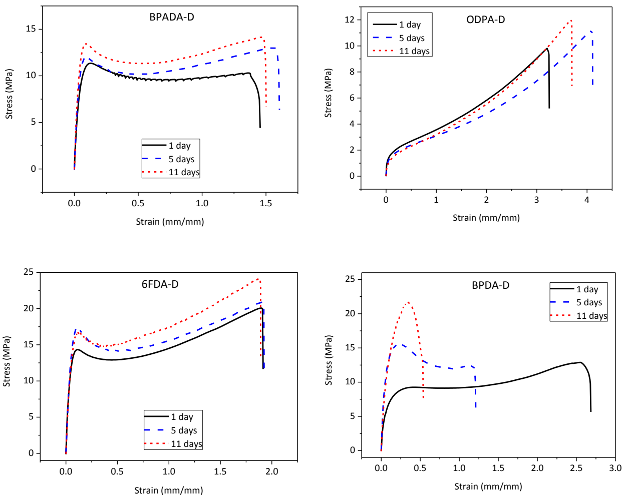
Figure 8. Effect of annealing time on the stress-strain behavior of the four PIs. T_{ann} = T(\tan \delta_{MAX}) = T_g .
