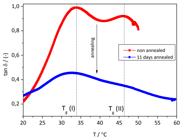
Figure 7. Rheological T-sweep curves. Effect of annealing on the glass transition relaxation behavior of the BPADA-D polymer. Red curve represents the non-annealed polymer and the blue curve shows the polymer annealed for 11 days at T_{ann}=T(\tan \delta_{MAX})=T_g .
