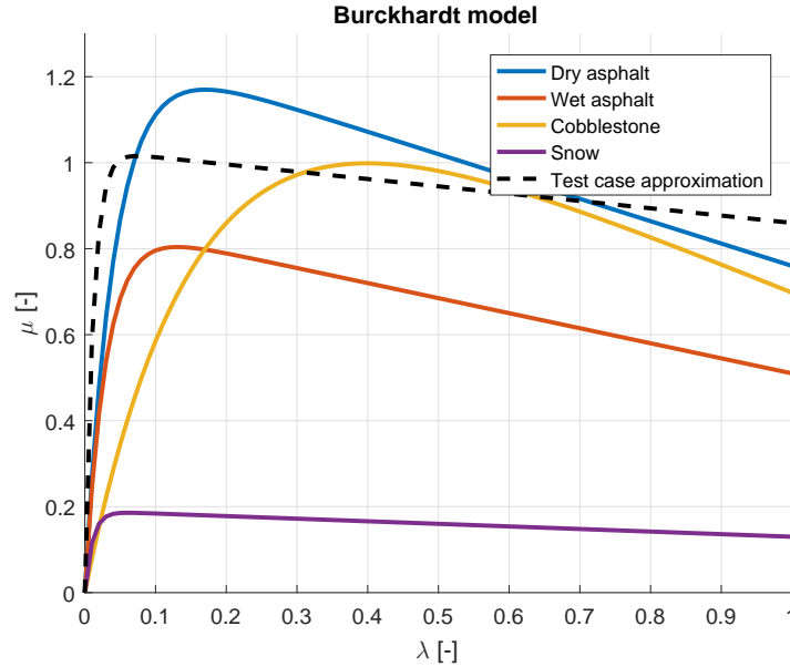
Figure 4-1: Burckhardt model
