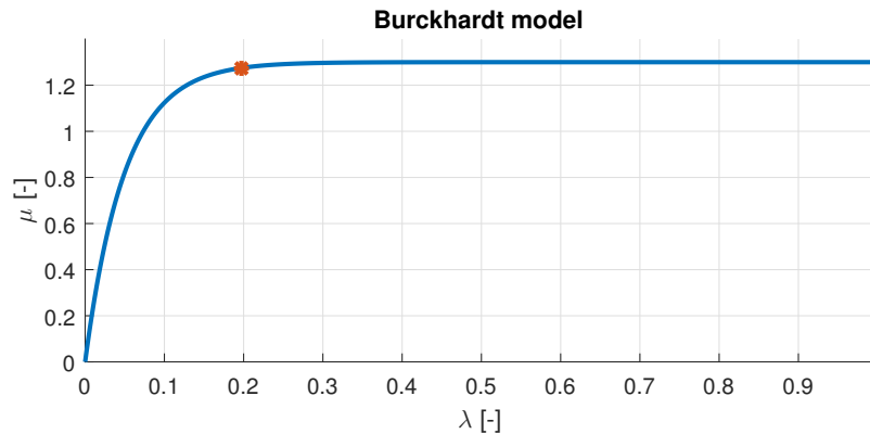
Figure 3-2: Friction coefficient curve without a peak
