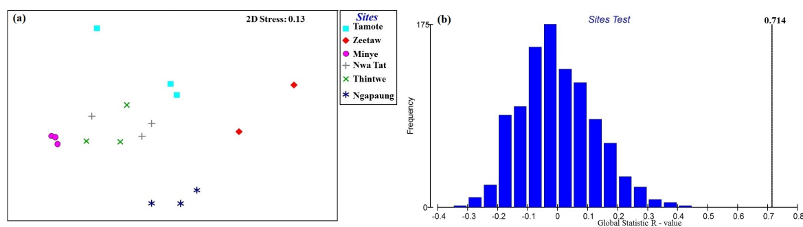
Figure 5. (a): Dimensionless MDS ordination plot of morpho-species contributions among six channels based on the Bray–Curtis similarity matrix of square root transformation. (b): ANOSIM plot for morpho-species contribution similarity among six channels.
