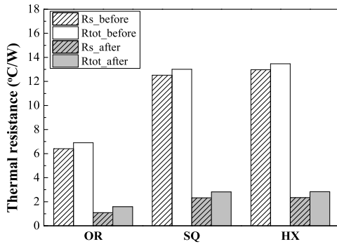
FIGURE 10. Total and spreading thermal resistance of three types of MC LED module before and after optimization.
