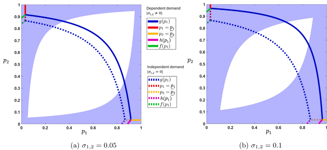
Fig. 6. Change of optimal policy regions for F = 100, D = 100, c_1 = 20, c_2 = 20 with dependent demand. The shaded area represents the infeasible combinations of p_1 and p_2 for the given \sigma_{1,2} value. In the presence of demand dependency, (x_1^*, x_2^*) = (0, 0) below the solid blue line, and (x_1^*, x_2^*) = (1, 1) above the solid blue line.
