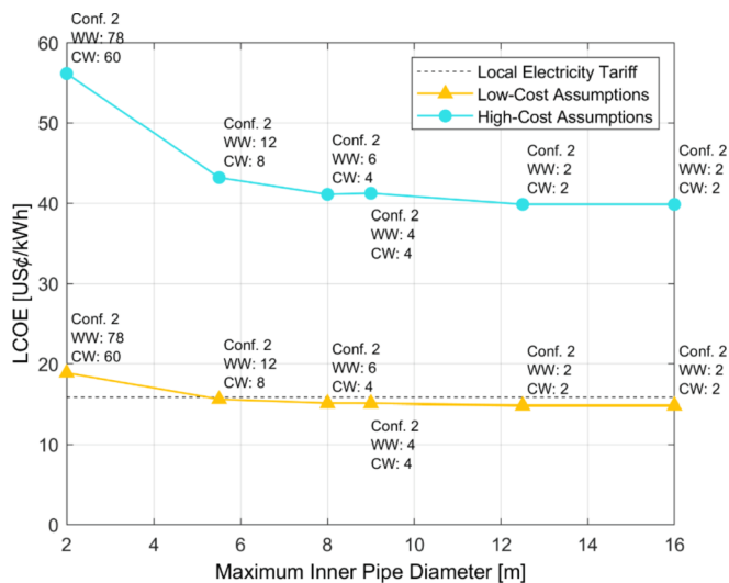
Fig. 7. Impact of maximum seawater pipe diameter on the LCOE at 136 MW gross . Labels show temperature configurations and the number of required pipes.
