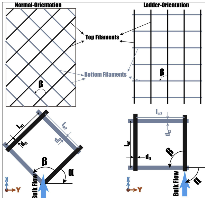
Fig. 1. Schematic view of spacers with flow attack angle of 45^\circ (normal orientation) and 90^\circ (ladder orientation). The flow attack angle is denoted with \alpha and the hydrodynamic angle with \beta . The relative distance between axes of two consecutive spacer filaments is defined as the ratio of filament length ( l_m = l_{m1} = l_{m2} ) to the channel height ( H_{CH} ). Spacers used in this article have the same filament mesh in flow direction ( l_{m1} ) and perpendicular to the flow ( l_{m2} ). The XY-plane is defined as the 2D space that represents the direction of flow in X- and Y-direction. X denotes the main direction of the flow (x-component of flow), and Y denotes the flow direction perpendicular to the main flow and perpendicular to the channel height (Z).
