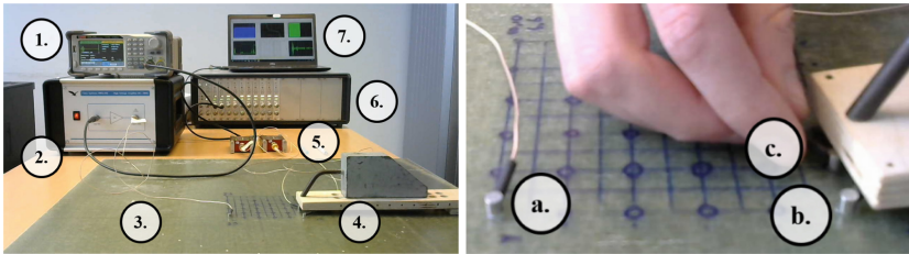
Fig. 4. Experimental setup: The left figure shows a general overview and the right figure is a close-up. Numbers 1–7 relate to the Siglent SDG10251 waveform generator, Falco WMA-300 amplifier, test specimen, measurement sensor fixture, Vallen AEP5H preamplifiers, Vallen AMSY-6 data acquisition system and measurement laptop, respectively. Letters a-c denote the actuator, reference sensor and measurement sensor. All transducers are of the VS600-Z1 type.
