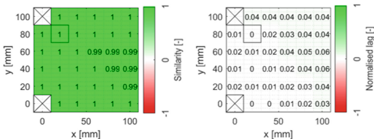
Fig. 6. Comparison between simulated response in out-of-plane direction v [mm] at location (20,80)mm and reconstructions from measurements at other locations towards this location. The left figure shows the Similarity index between the measurement and the reconstructions. The right figure shows the lag relative to a period in the signal ( 1/(40\text{ kHz}) ).
