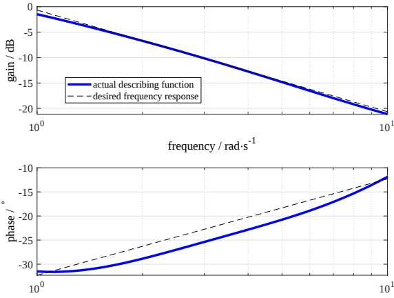
Fig. 6 Describing function of (32) when \gamma_1 \approx 0.8 , \gamma_2 \approx -0.6331 , corresponding to a gain slope of -20 dB/decade and a phase slope of 20^\circ /decade.
