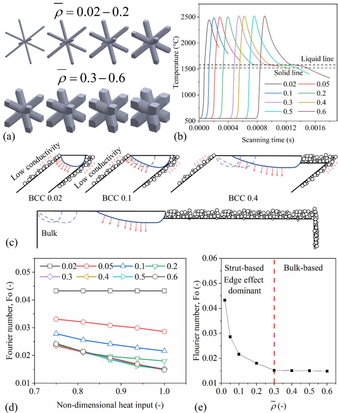
Figure 9. Edge effect in L-PBF of NiTi BCC architected materials: (a) CAD model of unit cells, (b) temperature history at the central point of the strut, (c) schematic diagram of edge effect, (d) the effect of non-dimensional heat input on the Fourier number, and (e) The effect of relative density of Fourier number for the parameters used in the current study.
