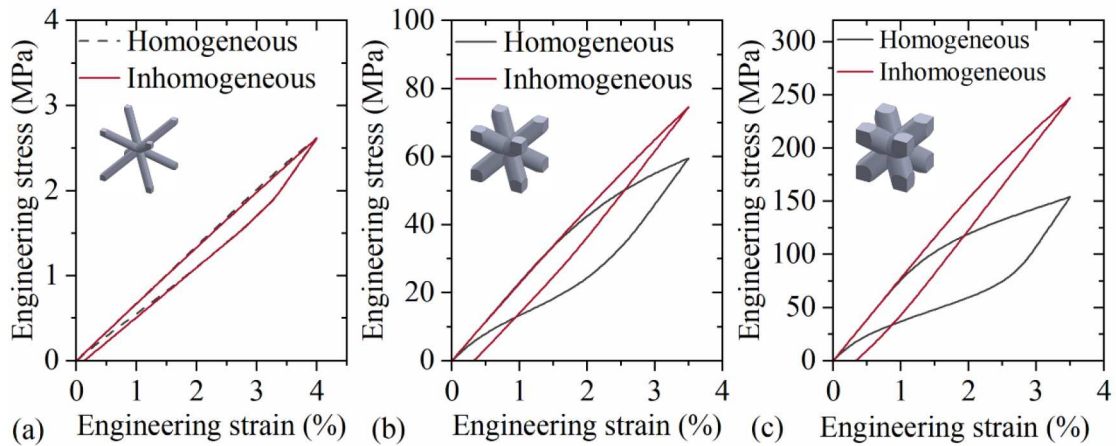
Figure 11. Engineering stress-strain response of NiTi architected materials with inhomogeneous and homogeneous martensitic transformation temperatures: (a) BCC 0.1, (b) BCC 0.4, and (c) BCC 0.6.
