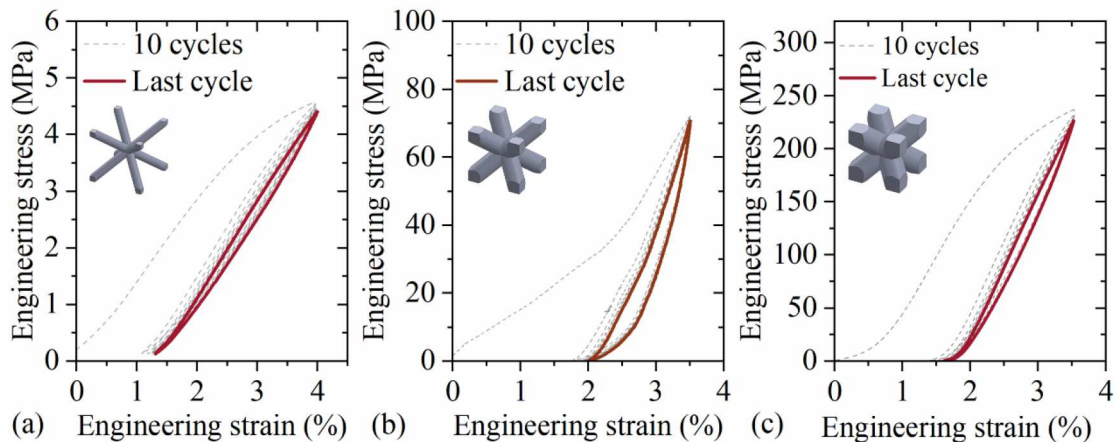
Figure 14. Cyclic compression tests on fabricated BCC architected materials at 54°C: (a) BCC 0.1, (b) BCC 0.4, and (c) BCC 0.6 samples.
