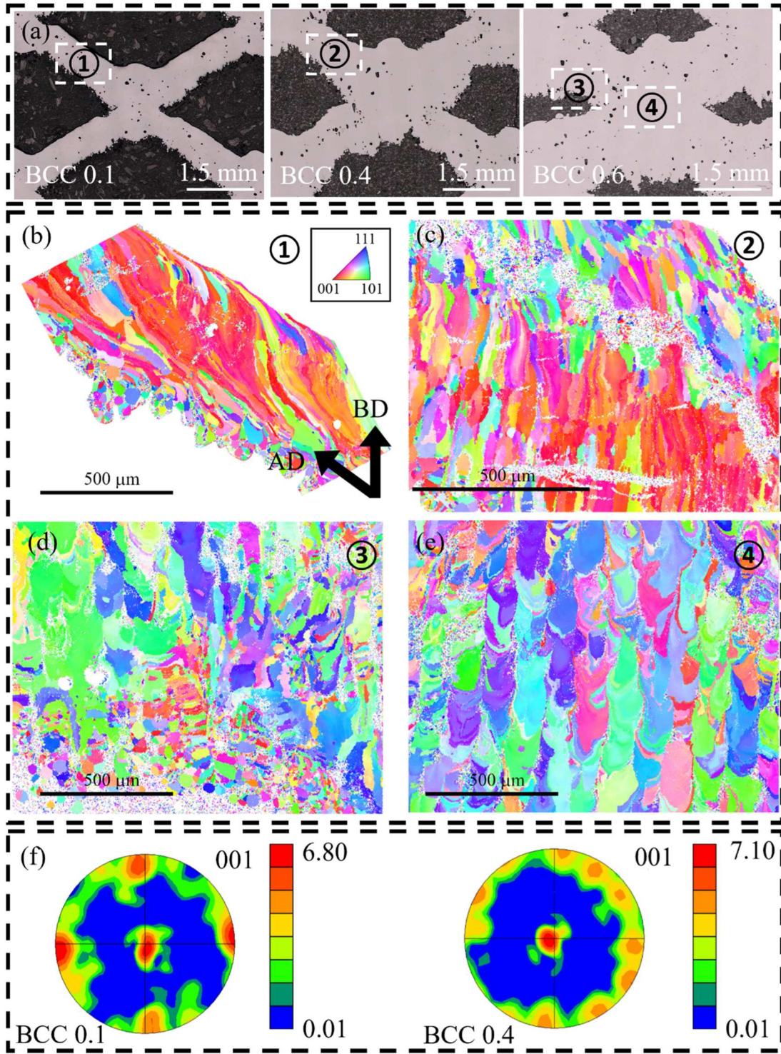
Figure 5. (a) Selected areas of BCC samples with relative densities of 0.1, 0.4, and 0.6. (b) Inverse Pole Figure (IPF) of the macroscopic cross-section for the BCC 0.1 sample. (c) IPF of the strut for the BCC 0.4 sample. (d, e) IPF of the macroscopic cross-section of the strut and node for the BCC 0.6 sample. (f) Corresponding Pole Figure (PF) for the BCC 0.1 and 0.4 samples.
