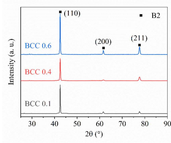
Figure 4. XRD patterns of BCC 0.1, 0.4 and 0.6 NiTi samples at room temperature.
