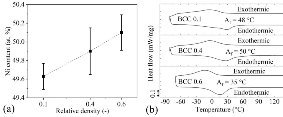
Figure 6. Ni content from (a) EDS and (b) DSC results of the BCC architected materials with relative densities of 0.1, 0.4 and 0.6.
