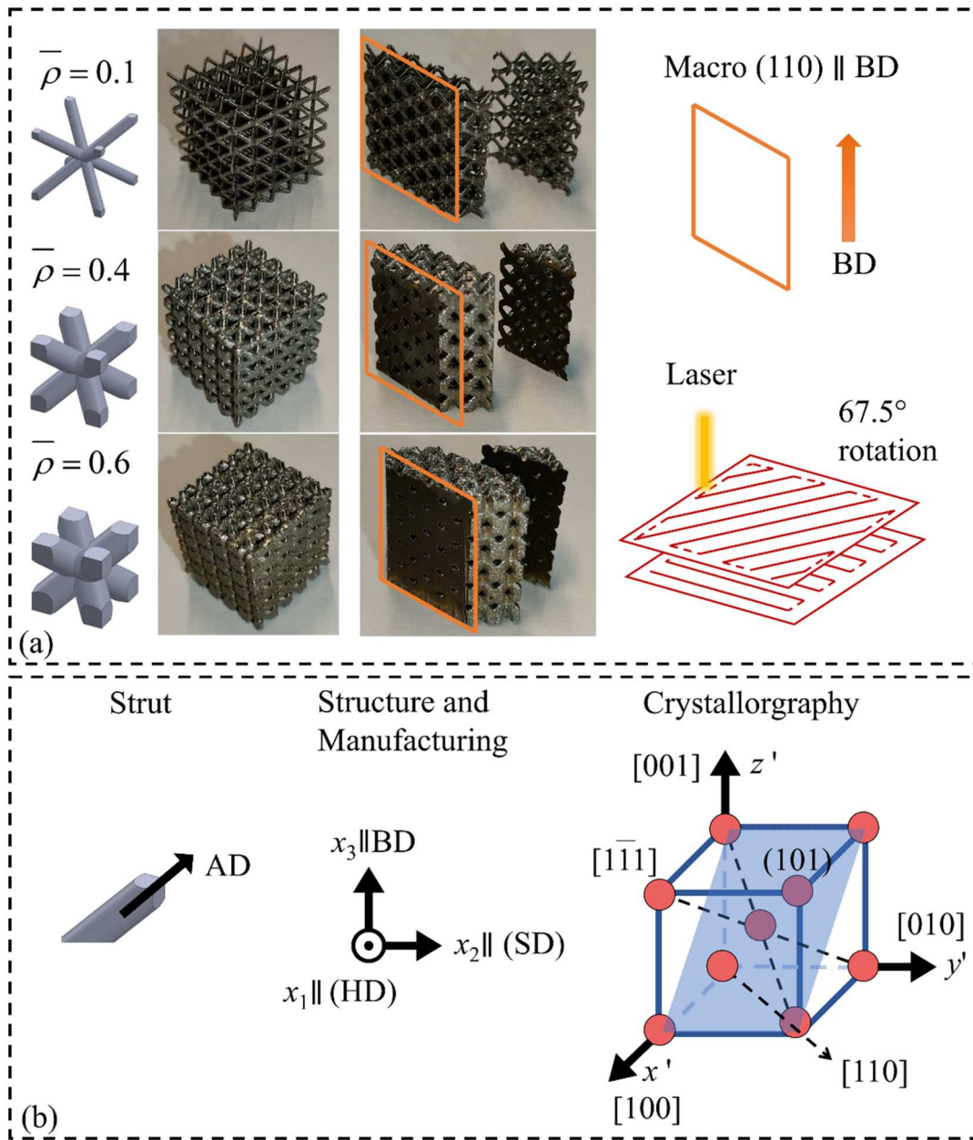
Figure 1. (a) Schematic diagram of macroscopic (110) cutting plane of as-fabricated samples (b) coordinate systems used in the current study.
