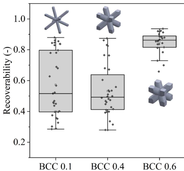
Figure 7. Recoverability in the instrumented indentation of BCC 0.1, 0.4 and 0.6 samples, including statistical mean, median and range.
