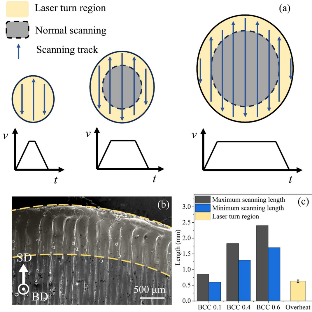
Figure 10. Representation of the laser turn region: (a) schematic diagram (b) SEM picture, and (c) the comparison of scanning length and length of laser turn region.
