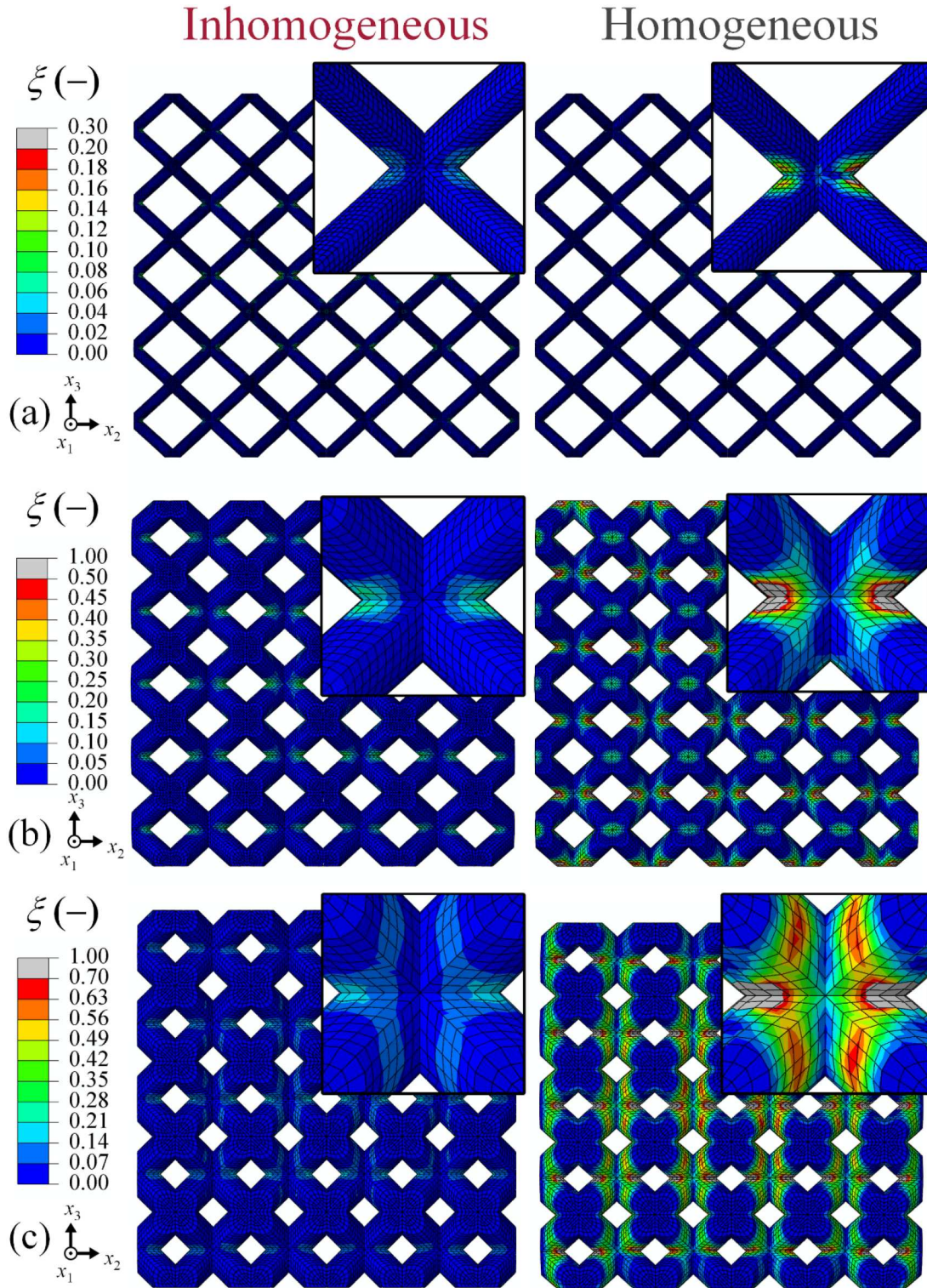
Figure 13. Contour plots of martensitic volume fraction resulting from the inhomogeneous and homogeneous martensitic transformation temperatures in (a) BCC 0.1, (b) BCC 0.4 and (c) BCC 0.6 samples under maximum loading.
