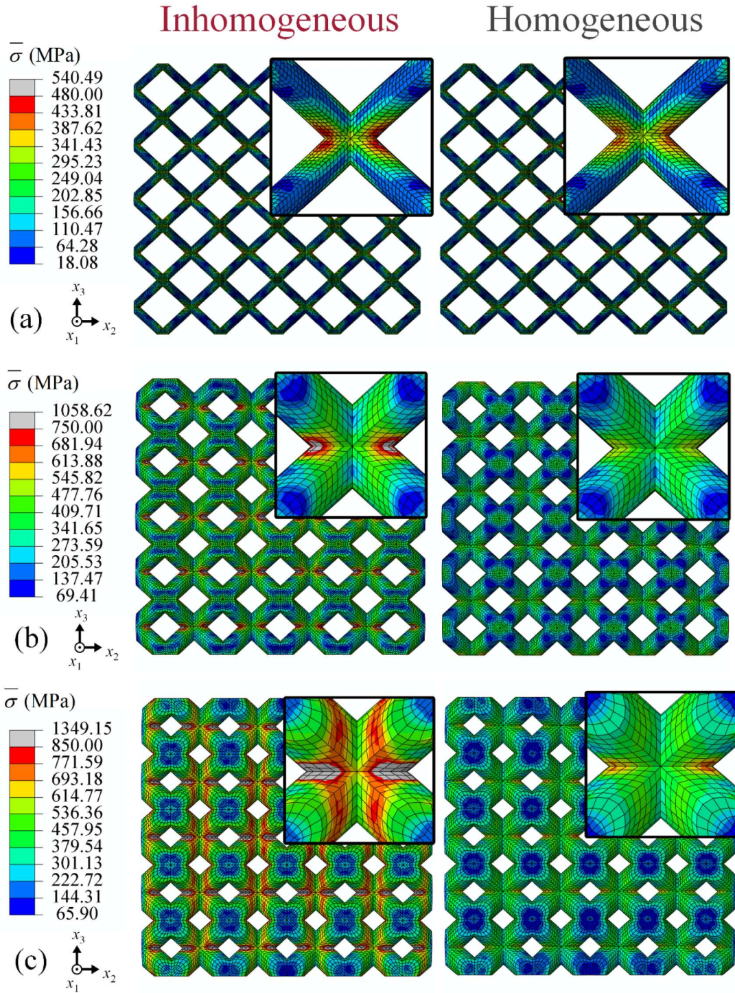
Figure 12. Contour plots of equivalent (von Mises) stress resulting from the inhomogeneous and homogeneous martensitic transformation temperatures in (a) BCC 0.1, (b) BCC 0.4, and (c) BCC 0.6 samples under maximum loading.
