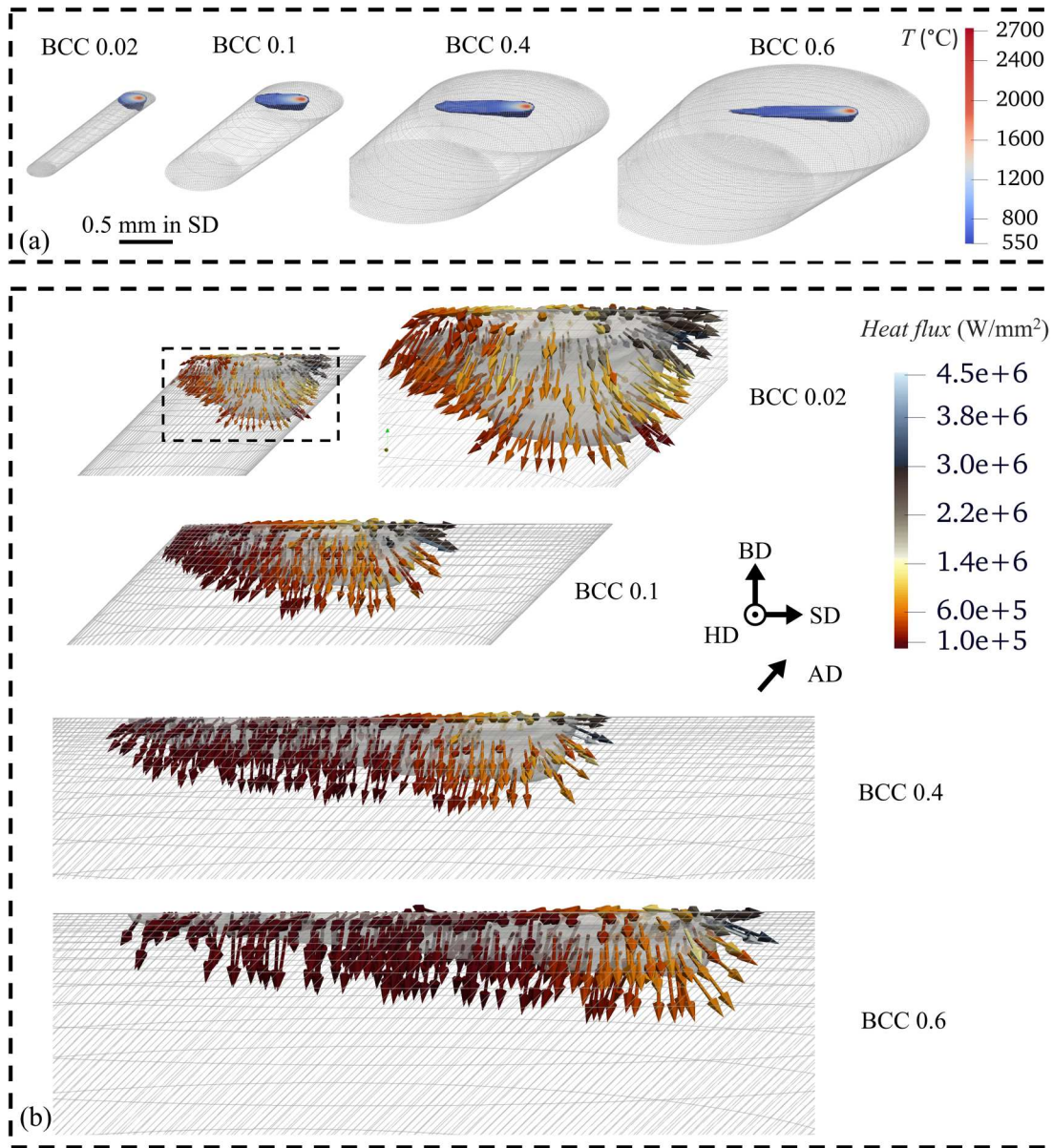
Figure 3. (a) Melt pool profile and (b) heat flow at the solid-liquid zone of melt pool during L-PBF of BCC architected materials with the relative density of 0.02 (an extreme case), 0.1, 0.4, and 0.6.
