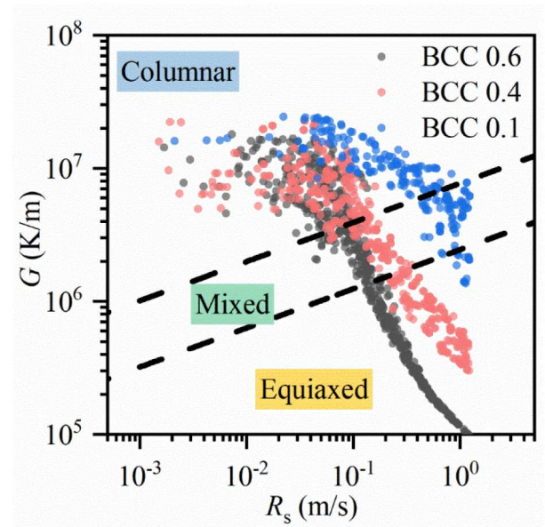
Figure 8. (a) Columnar to equiaxed transition of L-PBF NiTi, where G is the temperature gradient and R_s is the solidification rate.
