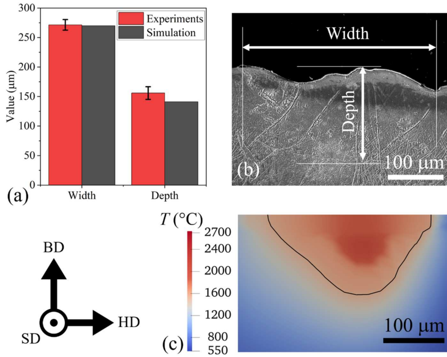
Figure 2. (a) Validation of thermal simulation by comparing the width and depth of the melt pool, (b) experimental melt pool profile, and (c) corresponding melt pool profile from thermal simulation.
