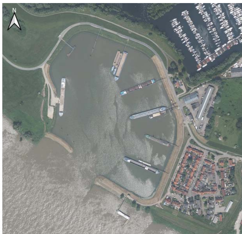
Figure 5.37: Lobith (NL), overnight harbour with floating landing stages (aerial imagery by the National Georegister (NGR) is licenced under CC BY 4.0).
