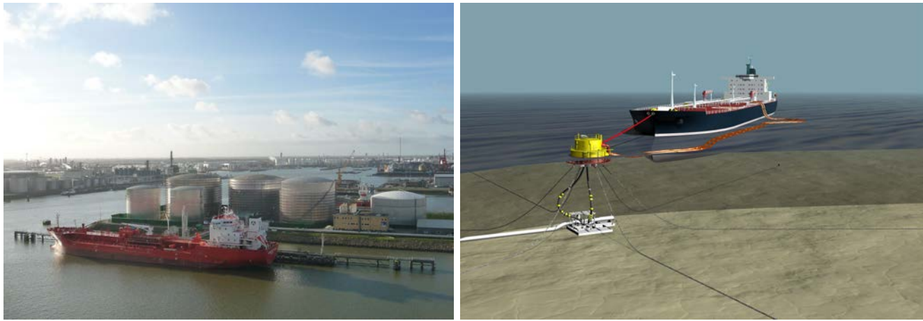
Figure 5.5: Tanker mooring arrangements; left: T-jetty mooring in Botlek, Rotterdam, the Netherlands (by BoH is licenced under CC BY-SA 3.0); right: single point buoy mooring (Functional SPM (Turret Buoy) by BluewaterPR is licenced under CC BY-SA 4.0).
