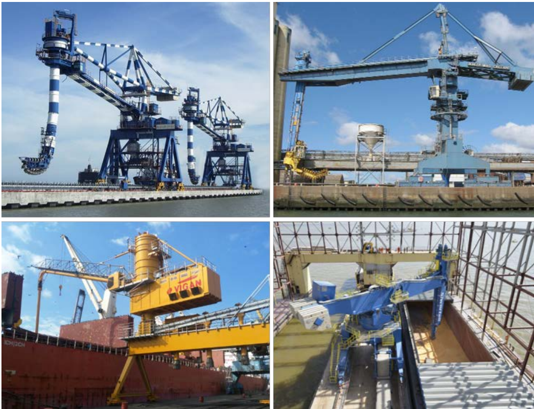
Figure 5.22: Continuous unloaders; top left: bucket elevator type; top right: chain type; bottom left: pneumatic type; bottom right: screw type (images by PIANC, 2019b , are licenced under CC BY-NC-SA 4.0, Port-de-commerce-de-Lorient by Pline is licenced under CC BY SA 3.0).
