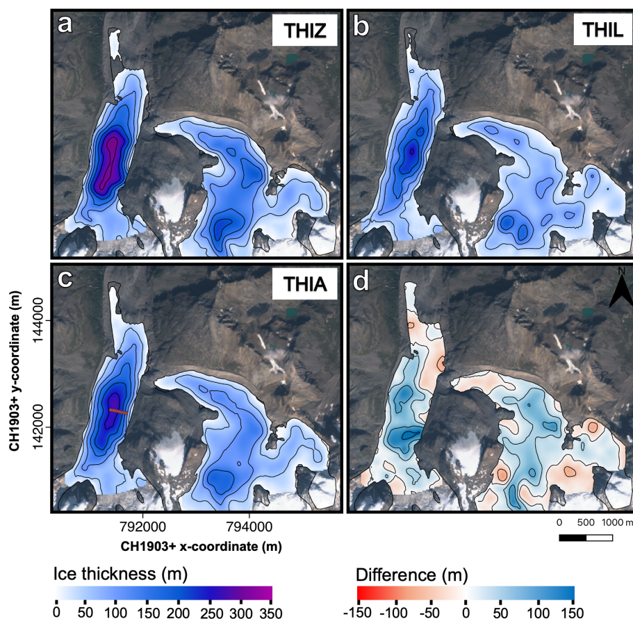
Figure 3. Ice thickness distribution of the ablation area of the Morteratsch–Pers glacier complex in 2020. (a) THIZ (ice thickness distribution of Zekollari et al., 2013), (b) THIL (ice thickness distribution of Langhammer et al., 2019) and (c) THIA (average ice thickness distribution). The difference between THIZ and THIL is shown in panel (d). Contour lines represent 50 m intervals. Note that at the front of Vadret da Morteratsch and locally at the front of Vadret Pers, the glacier outline is larger than the ice thickness dataset. The current surface elevation of these areas is lower than the bedrock elevation inferred from THIL and THIZ. The locations of the ice thickness measurements of 2020 are added in panel (c) with red circles. The background image is a Sentinel-2 true colour composite satellite image from 13 September 2020.
