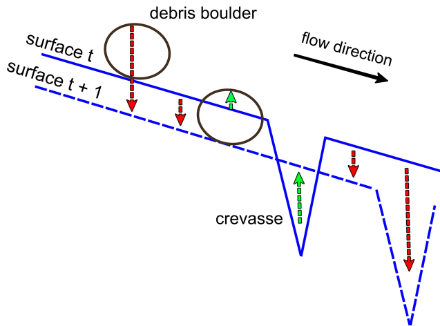
Figure 4. The advection of surface topography (such as debris boulders and crevasses) can alter surface elevation changes between time step t and t + 1 (red: negative \partial h / \partial t ; green: positive \partial h / \partial t ). The net effect on the surface elevation depends on the amount of lowering and the vertical extent of the moving features on the glacier surface.
