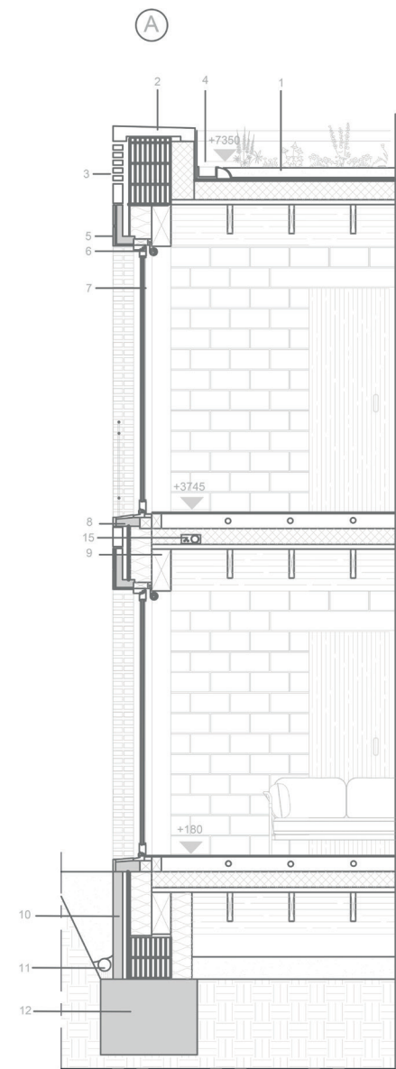
Detailing
