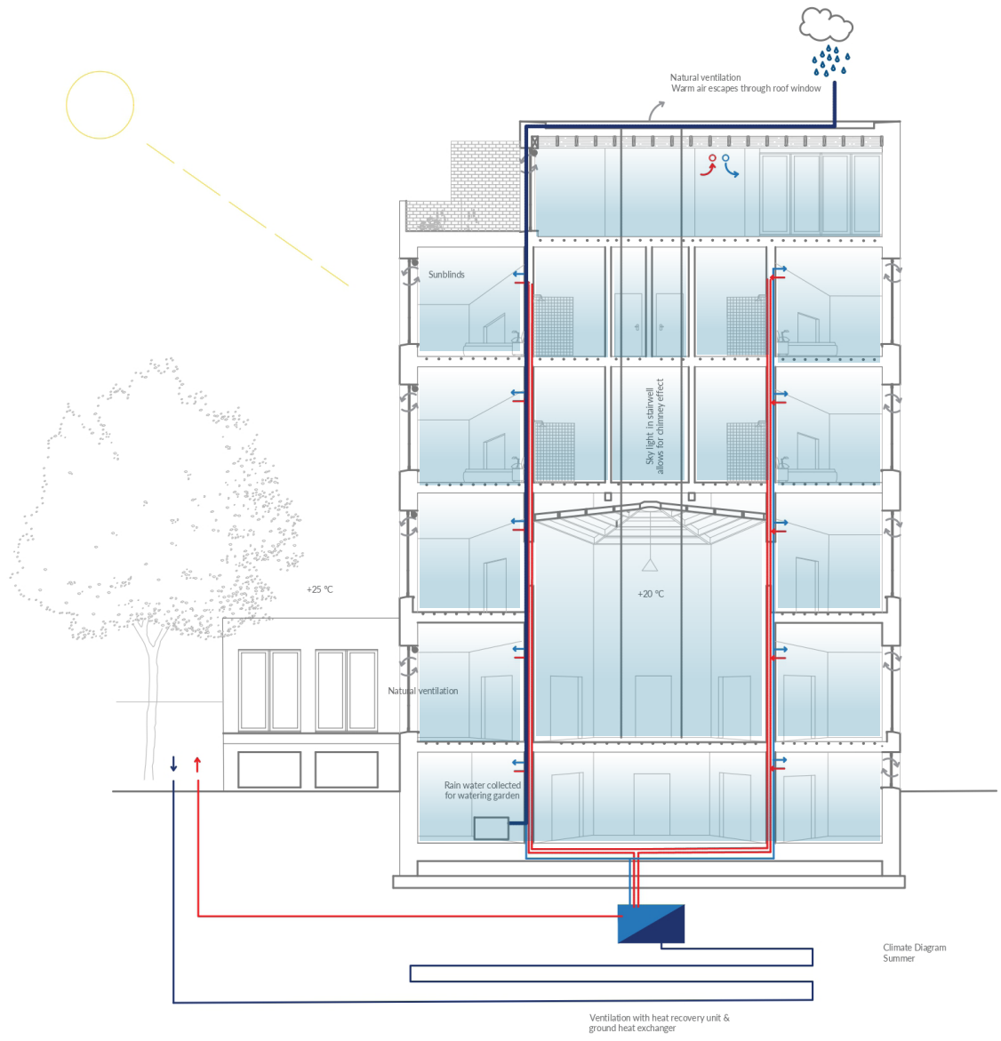
Climate scheme Summer
