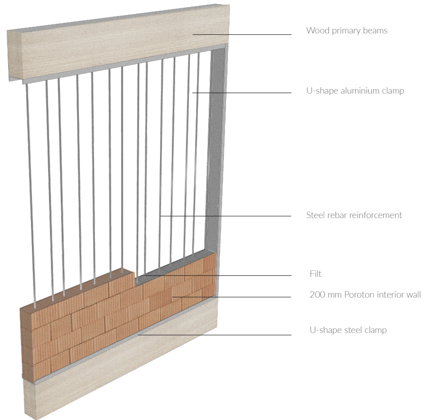
Structural principle
