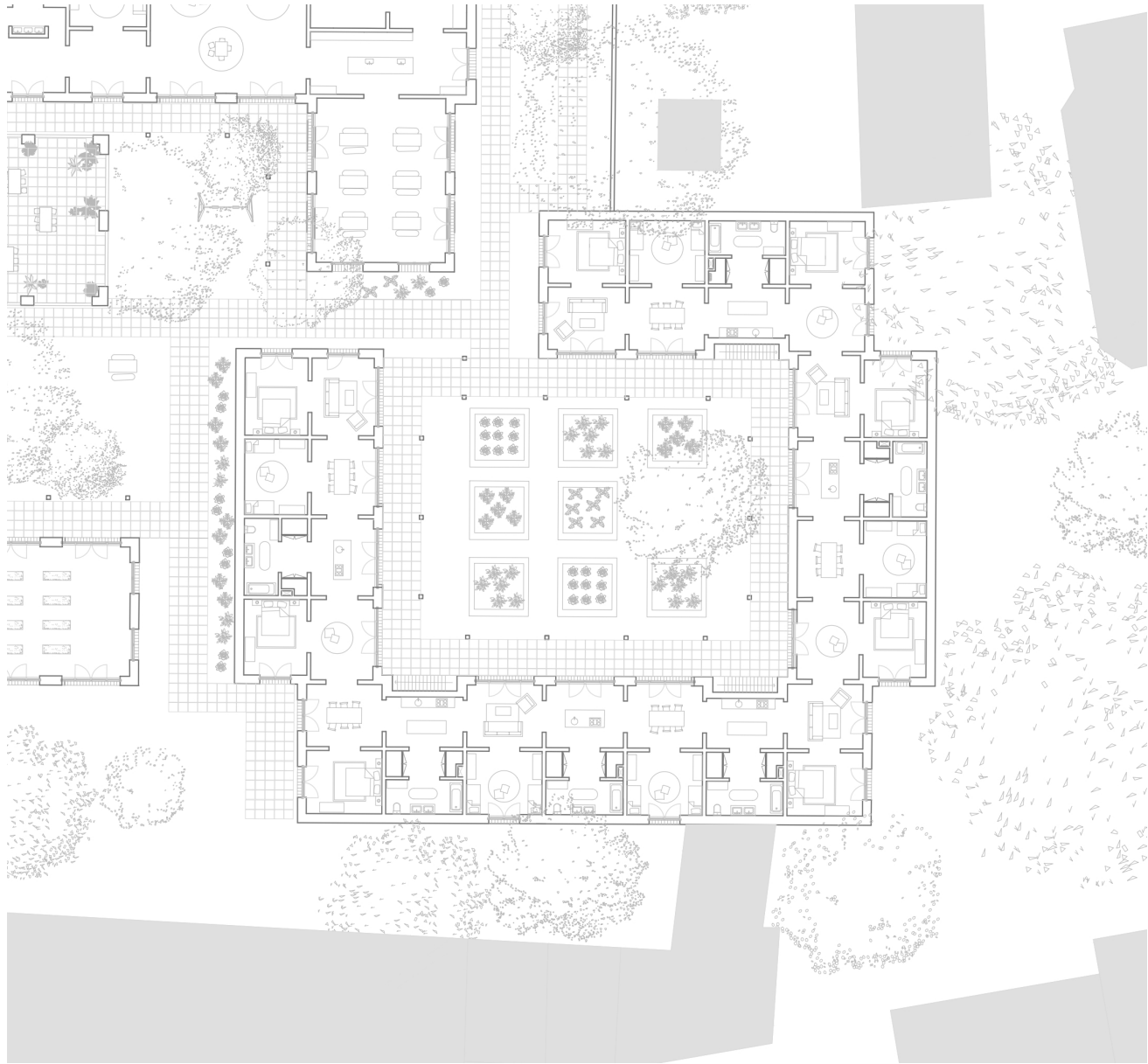
Groundfloor plan residences
