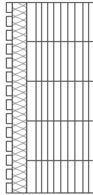
Poroton with stone strips R_c = 3,7
