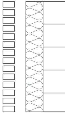
Traditional cavity wall R_c = 3,7
