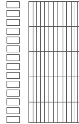
Poroton uninsulated cavity wall R_c = 3,5
