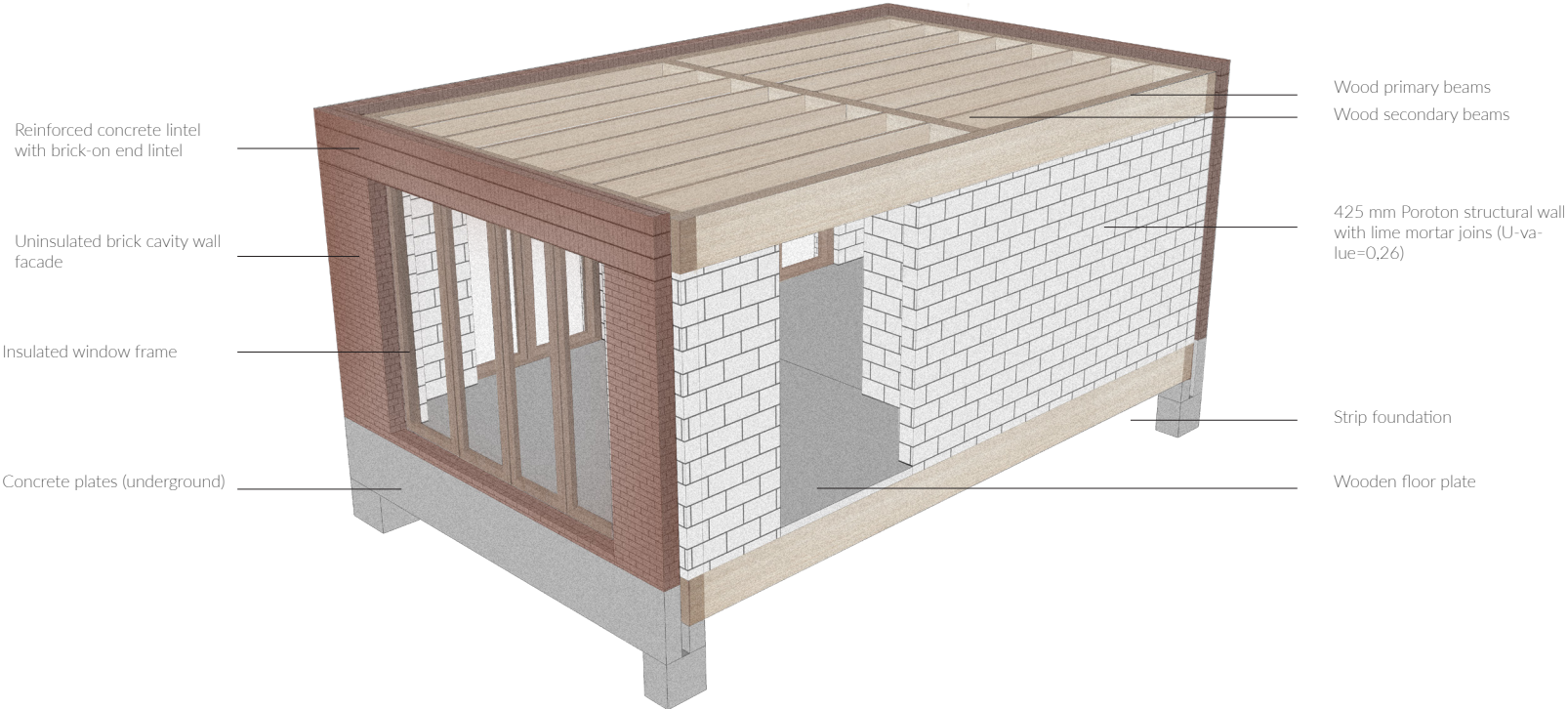
Structural principle
