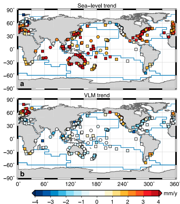
FIG. 2. Linear trends at individual tide-gauge locations. (a) Trend in relative sea level over available data within 1958–2014. The local barotropic effects of wind and pressure were removed using the regression model before computing the trend. (b) Linear trends in VLM. The blue line depicts the boundaries of the ocean basins. Note that, given the availability of observations, the period over which the trends are computed differs between stations.
