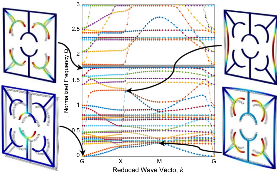
Fig. 7.24 Dispersion curves and mode shapes of the diagonal structure for printing speed 20mm/s. Dispersion curves and mode shapes of the diagonal structure with the 4D printing speed at 20mm/s after the heating–cooling process.
