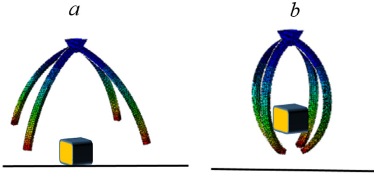
Fig. 7.11 The gripper deformed configuration. The FE Abaqus simulation of the gripper at printing speed: (A) 20 and (B) 40mm/s. No permission required.
