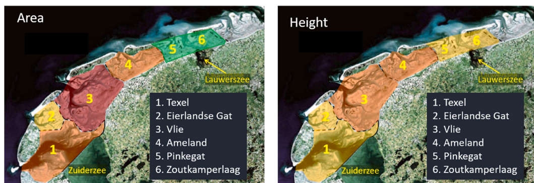
Fig. 9. Graphical illustration of the results for the SLR-17 scenario, with the changes in area on the left and changes in average flat height to the right. The colours indicate how large the losses are, with the largest losses in red (>40% by 2100), the intermediate losses in orange (20%–40%) and yellow (10%–20%) and smallest losses in green (<10%). (For interpretation of the references to colour in this figure legend, the reader is referred to the Web version of this article.)
