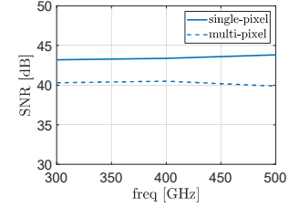
Fig. 2. SNR using the QO setup for the single- and multi-pixel detectors
