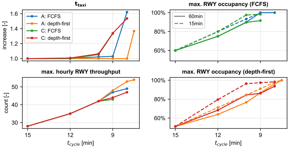
Figure 5.9: KPIs w.r.t. t_{\text{cycle}} for continuous schedules of test cases A and C, comparing the high-level variants FCFS and depth-first
