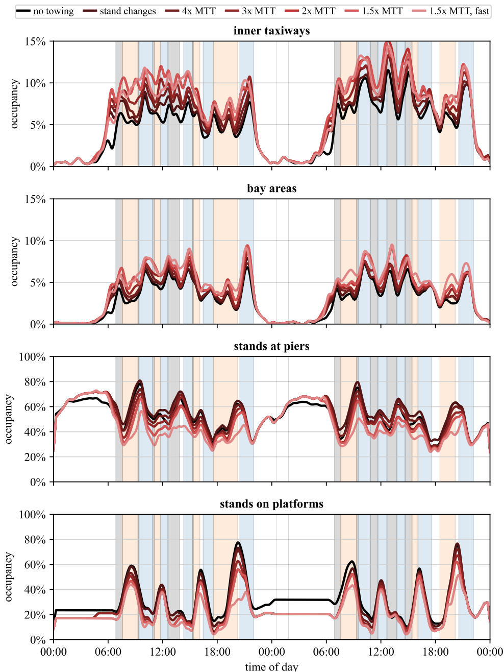
Figure 8.20: Comparison of occupancy rates in different areas of the airport across the simulated towing operations from Table 8.7
