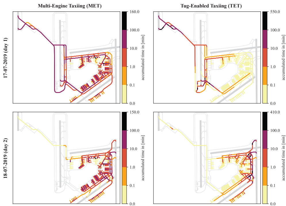
Figure 7.7: Emission hotspots depicted through accumulated engine on time per layout location for departing aircraft for each day and each taxiing mode of operation
