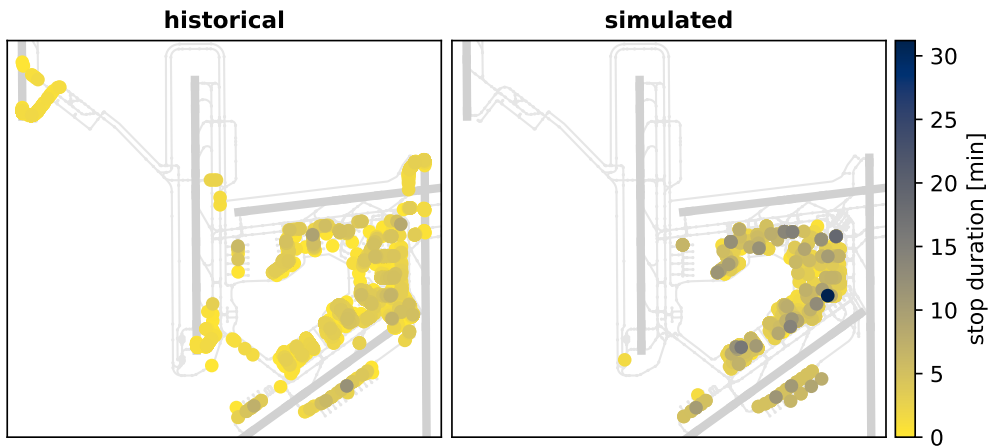
Figure 8.15: Outbound holding: stop locations and waiting durations >10 s of historical and simulated departing flights
