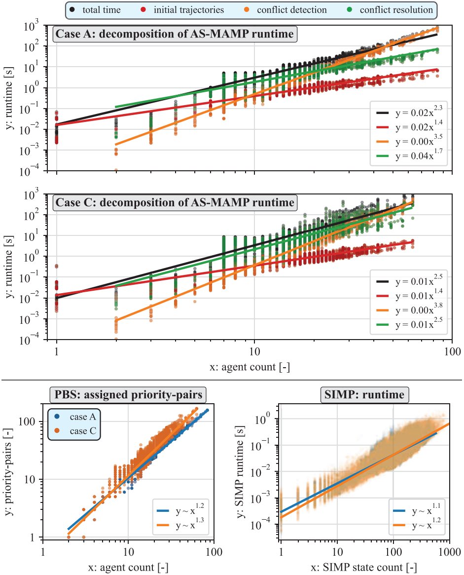
Figure 5.4: AS-MAMP computational performance based on 200 simulations per test cases A and C, resulting in total in 3 854 planning rounds with approx. 695 k SIMP-calls
