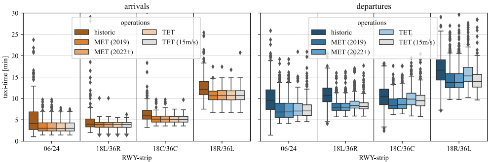
Figure 7.5: Box-and-whisker plot of historical and simulated taxi times for arrivals and departures per runway-strip
