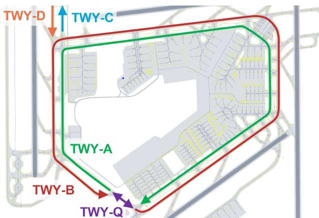
Figure 9.4: Standard taxiway flow directions as part of ATC procedures at Amsterdam Airport Schiphol
