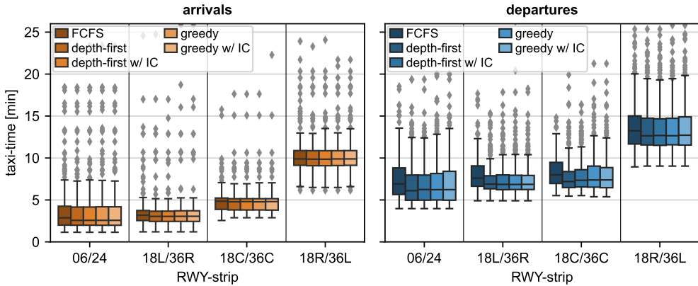
Figure 5.5: Box-and-whisker plots per runway for both inbound and outbound flights, showing the taxi time distributions of simulations of multi-engine taxiing (MET) operations using either FCFS or PBS variants as high-level in AS-MAMP
