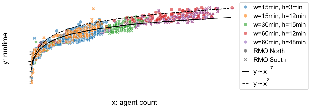
Figure 6.12: Runtimes of planning rounds over the number of agents; the solid and dashed black lines indicate polynomial time complexities of \mathcal{O}(x^{1.7}) and \mathcal{O}(x^2) , respectively
