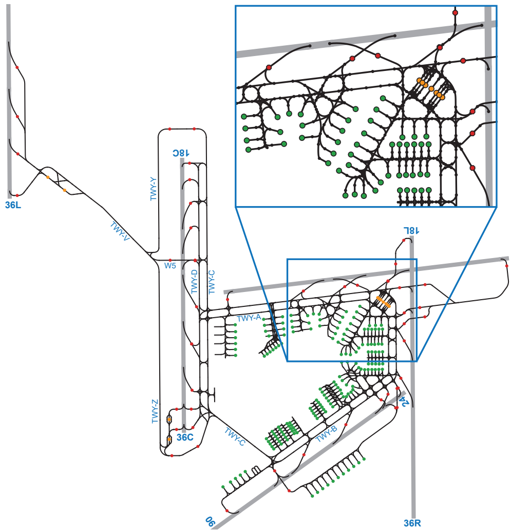
Figure 6.2: Graph of layout of Amsterdam Airport Schiphol with edges for runways (grey) or taxiways (black), and vertices for taxiway intersections (black), stopbars (red), holding points (orange), or gates (green)
