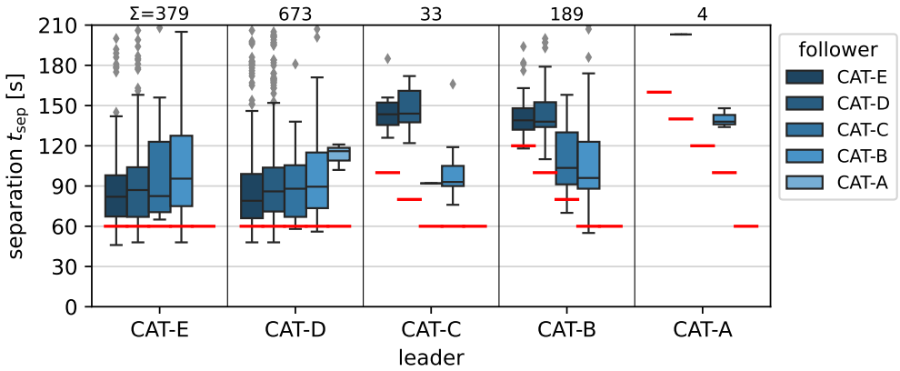
Figure 8.21: Temporal separation of consecutive takeoffs in historical data, grouped by RECATEU categories [133]; the minimum separation times for the respective RECATEU combinations of consecutive takeoffs is indicated by the red lines
