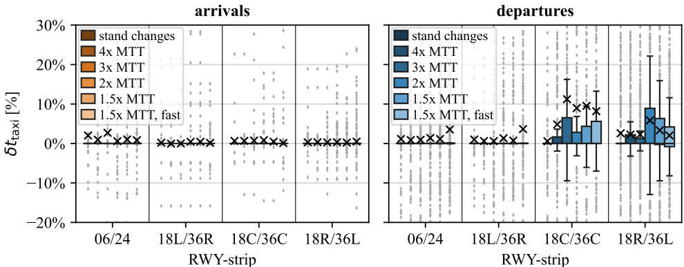
Figure 8.19: Normalised taxi time differences \delta t_{\text{taxi}} in relation to simulation 'no towing'; black cross denotes the mean value
