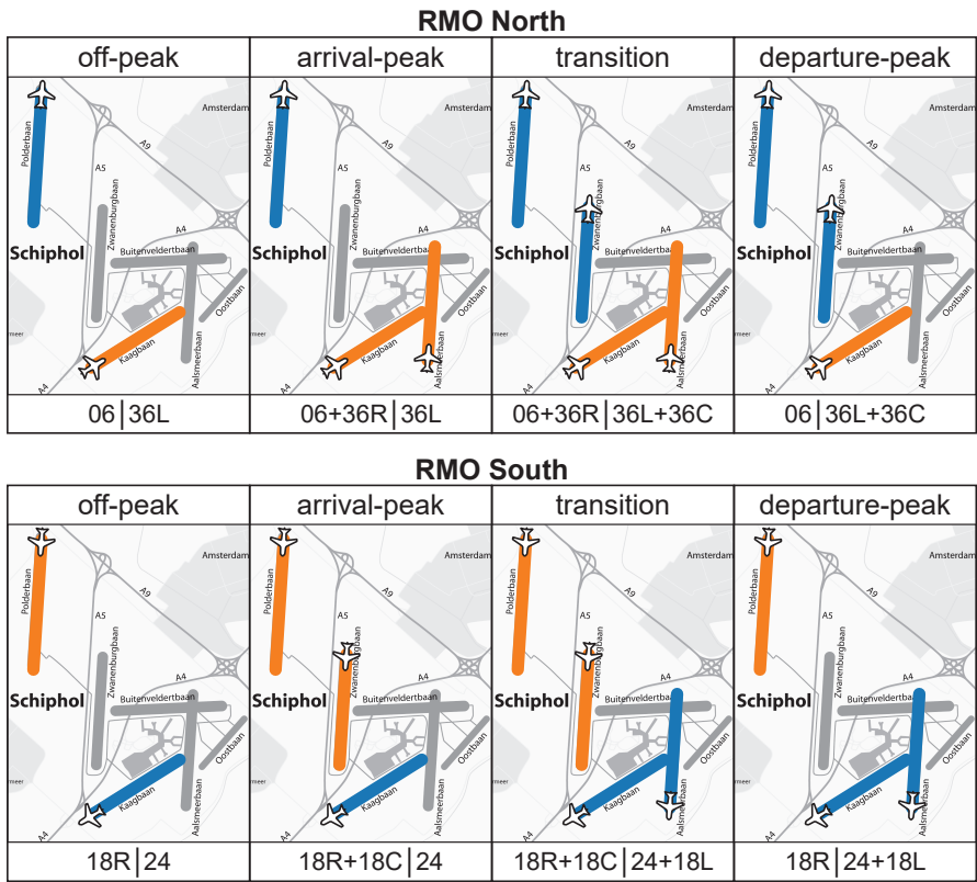
Figure 6.7: Runway modes of operation (RMO) at Schiphol: different phases of RMO North (top) and RMO South (bottom) with active runways for arrivals (orange) and departures (blue); background map adapted from [154]
