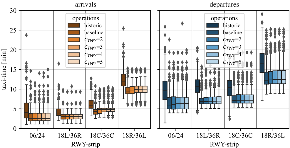
Figure 9.6: Comparison of taxi times per runway strip between historical operations and simulations with varying values of the cost factor c_{TWY}
