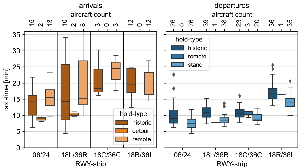
Figure 6.14: Box-and-whisker plot of historical and simulated taxi times dependent on the hold-type of arrivals and departures per runway-strip; simulation with w_p = 20 min and h_p = 10 min. The hold-type 'remote' denotes holding at one of the remote holding locations, 'detour' marks trajectories that go via one of these holding points. The hold-type 'stand' denotes explicit holding time at the stand, in contrast to implicit holding at the stand as emergent property to resolve conflicts during path planning
