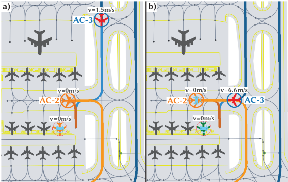
Figure 9.7: Fast-forward animations of a) the original trajectories for which the stand entry is blocked for AC-3, and b) the adapted routes when AC-2 uses a longer pushback path allowing AC-3 to enter the stand
