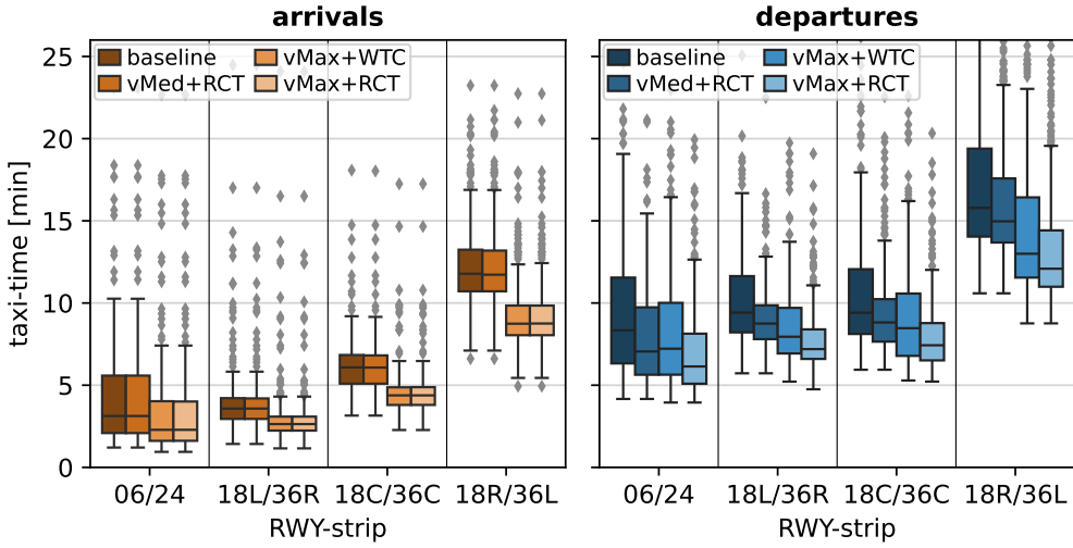
Figure 8.22: Box-and-whisker plots of taxi time distributions for arriving and departing flights per runway-strip
