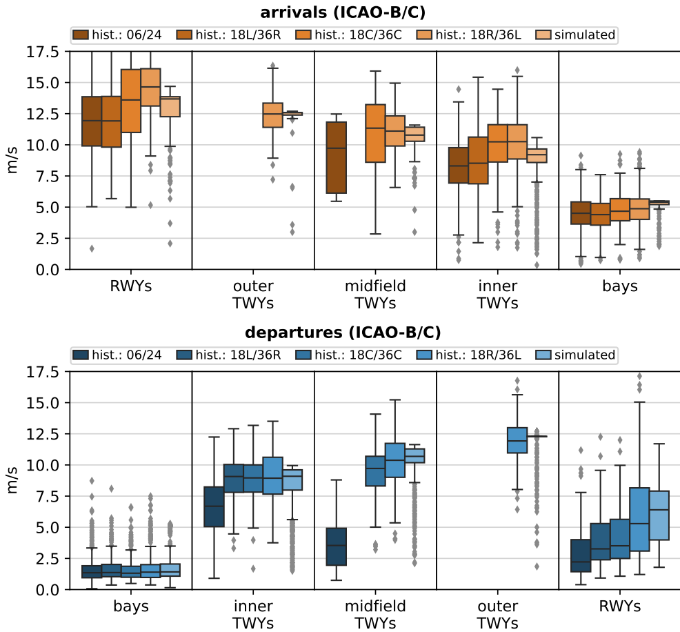
Figure 8.13: Comparison of average taxi speeds across the different taxiway areas from Figure 8.3 for both arriving (top) and departing flights (bottom)
