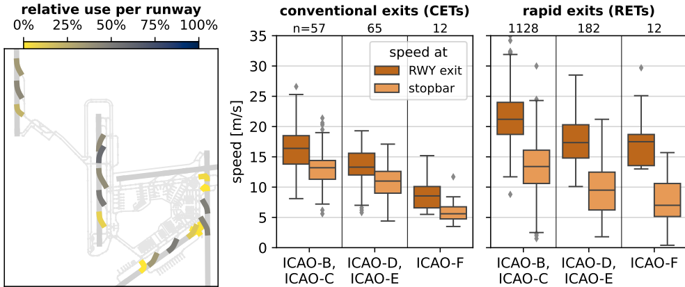
Figure 8.6: Historical landing speeds per aircraft type and type of runway exit
