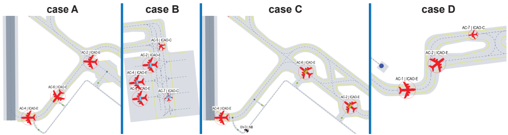
Figure 5.2: Simulation snapshots illustrating the bottleneck of each test case on the synthetic layout
