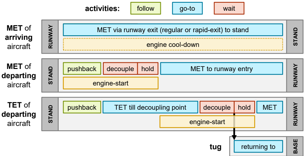
Figure 7.3: Activity sequence for arriving and departing aircraft; while engine-start (orange box) of departing aircraft is accounted for, engine cool-down (dotted orange box) is neglected
