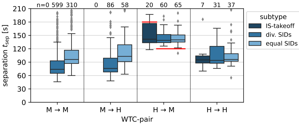
Figure 8.8: Temporal separation of historical takeoffs grouped by ICAO wake turbulence categories (WTC) [176]. Each WTC-pair is subdivided into intersection (IS) takeoffs, as well as following diverging or equal standard instrument departure (SID) routes. Red lines indicate the respective minimum separation times.
