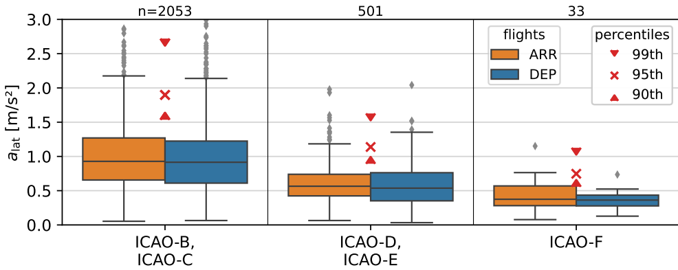
Figure 8.5: Distributions per aircraft type of historical lateral accelerations in curved taxiway segments for both arriving and departing flights
