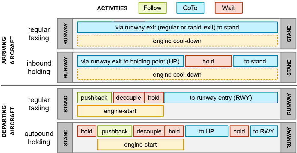
Figure 6.3: Activity sequences for regular taxiing of arriving and departing aircraft as well as inbound and outbound holding; while engine-start (orange box) of departing aircraft is accounted for, engine cool-down (dotted orange box) is neglected
