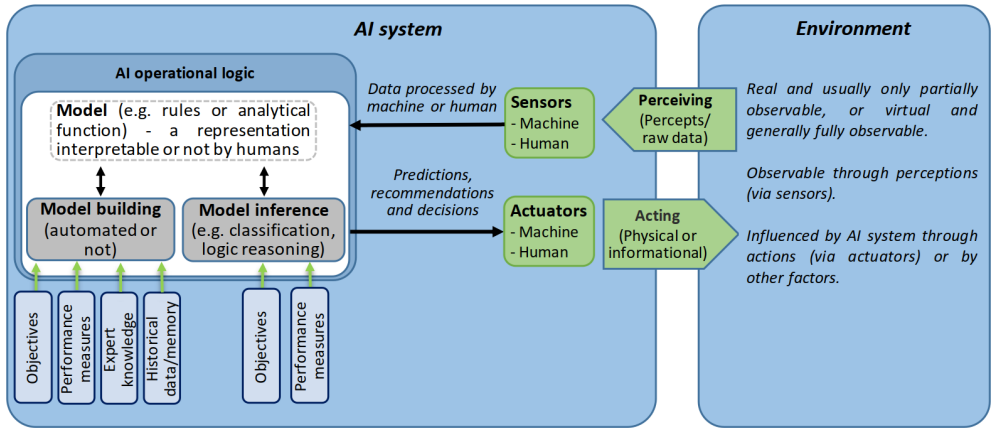
Figure 1.5: Schematic overview of an AI system and its elements, as defined by the AI Group of Experts at the OECD (AIGO); adapted from [19], Figure 1.4, p. 23
