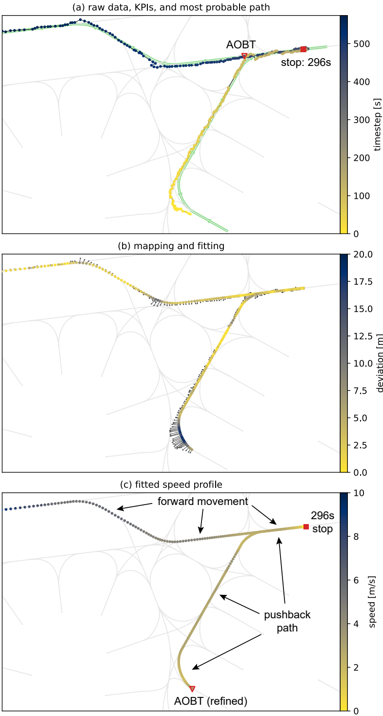
Figure 8.1: Illustration of methodology for evaluating historical track data
