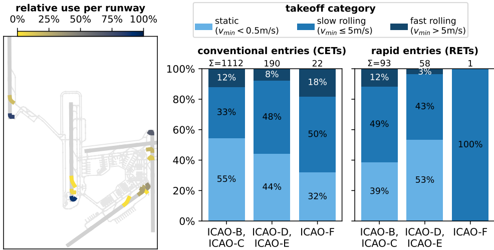
Figure 8.7: Share of takeoff categories of historical flights per aircraft type and type of runway entry
