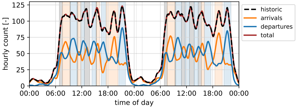
Figure 8.10: Hourly ground movements over the simulated 48 h. Shades denote the runway configuration phase: off-peak (white), arrival-peak (orange), transition (grey), and departure-peak (blue).
