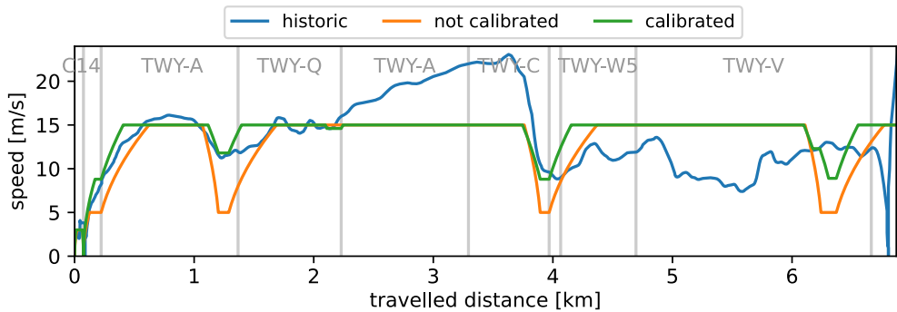
Figure 6.6: Exemplary historical, un-calibrated, and calibrated speed profiles of a departing flight travelling from stand C14 to runway 36L
