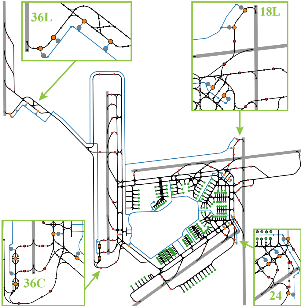
Figure 7.2: Graph of layout of Amsterdam Airport Schiphol with edges for runways (grey), taxiways (black), or service roads (blue), and vertices for gates (green), taxiway intersections (black), tug decoupling (orange) and all-clear points (grey), or stopbars (red)
