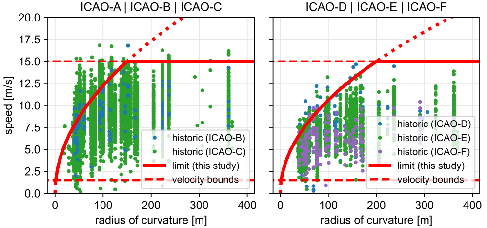
Figure 6.5: Calibration of curve speed with historical track data; the red dotted lines mark the speed limits computed using Equation (6.1)
