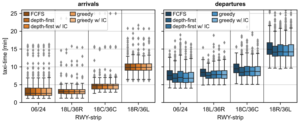
Figure 5.6: Box-and-whisker plots per runway for both inbound and outbound flights, showing the taxi time distributions of simulations of tug-enabled taxiing (TET) operations using either FCFS or PBS variants as high-level in AS-MAMP
