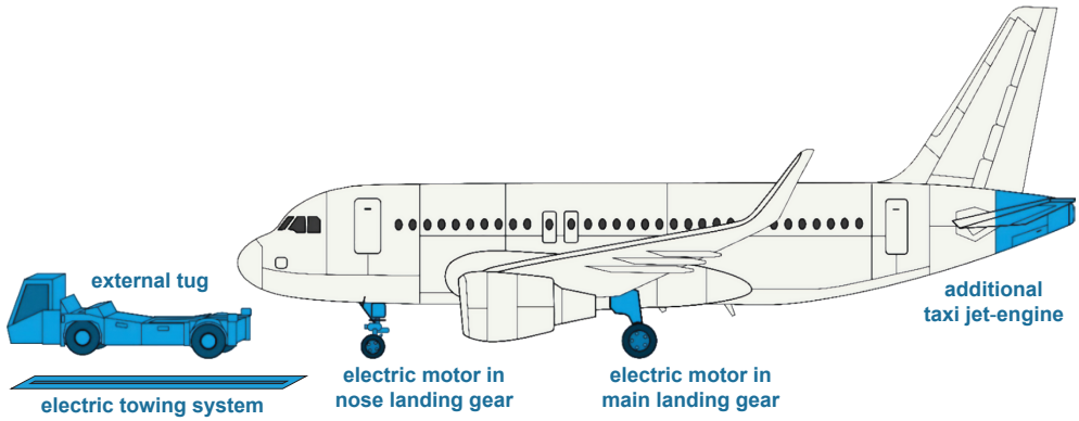
Figure 1.2: Overview of different engine-off taxiing concepts; based on [11]
