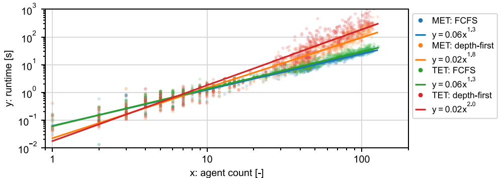
Figure 5.8: Computational runtimes of planning rounds of simulations of multi-engine taxiing (MET) and tug-enabled taxiing (TET) operations using either FCFS or depth-first search as high-level in AS-MAMP
