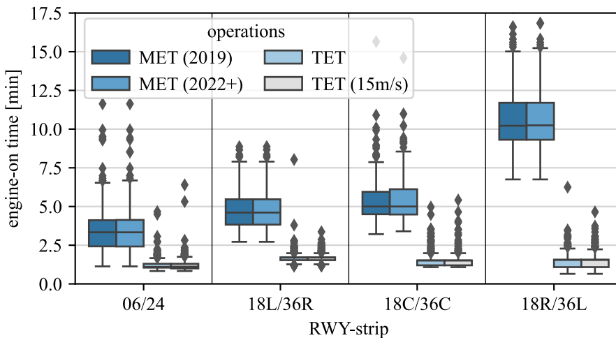
Figure 7.8: Box-and-whisker plot of engine-on times of departing flights per runway-strip
