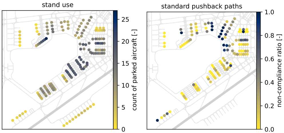
Figure 8.9: Historical stand use (left) and non-compliance rate to standard pushback path per stand (right)
