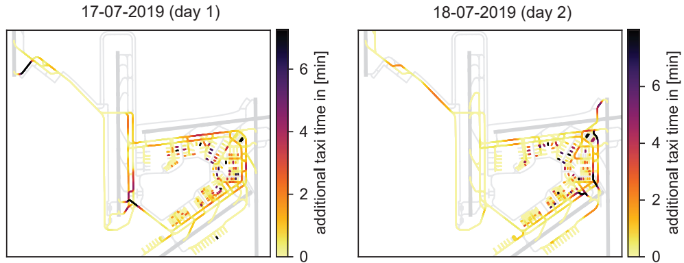
Figure 6.13: Additional taxi time per layout location on each of the two days, simulated with w_p = 20 min, h_p = 10 min
