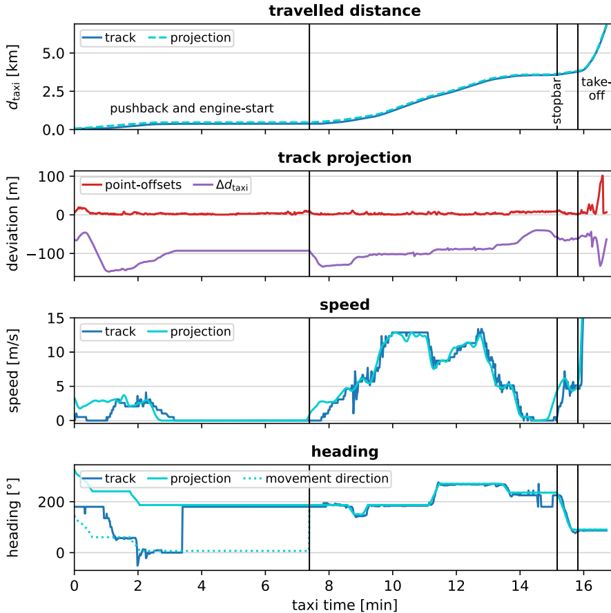
Figure 8.2: Projection KPIs of exemplary track of departing flight shown in Figure 8.1
