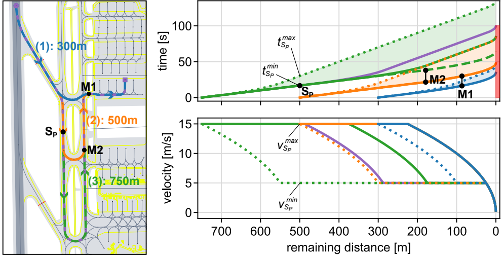
Figure 4.2: Exemplary trajectories through layout (left) and state space (right) to a stand that is occupied till t = 100 s resulting in a long goal constraint (red shade at 0 m)
