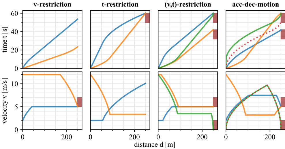
Figure 4.3: Exemplary motions visualised per column both in (d, t) -graph (top) and (d, v) -graph (bottom); the speed and time restrictions for the different examples are marked by red shades
