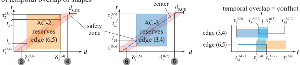
Figure 4.5: Graph reservations and exemplary conflicts (illustrated in top part), with path-reservations on edges along an agent's path (middle part) and neighbourhood-reservations on all other edges that are swept by an agent's shape (bottom part)
