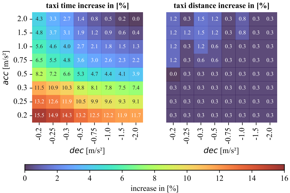
Figure 5.3: Sensitivity analysis of case A depicting how acceleration \text{acc} and deceleration \text{dec} influence the taxi time and distance, shown as increase in [%] w.r.t. the lowest sum over all flights.
