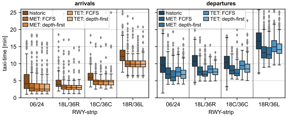
Figure 5.7: Box-and-whisker plots per runway for both inbound and outbound flights, showing the taxi time distributions of historical data, as well as simulations of multi-engine taxiing (MET) and tug-enabled taxiing (TET) operations using either FCFS or depth-first search as high-level in AS-MAMP
