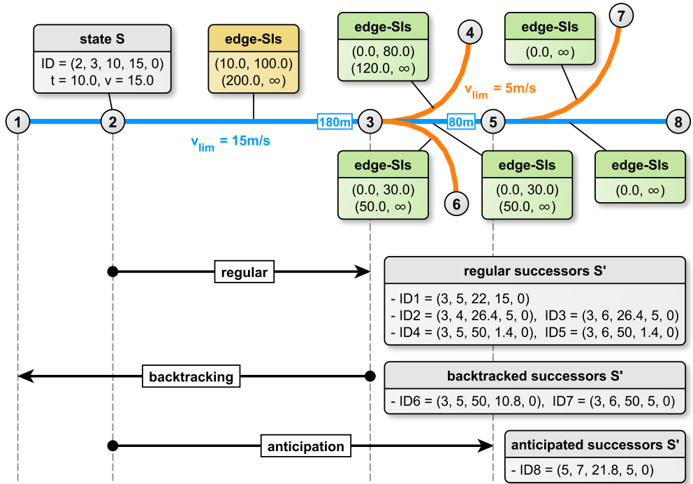
Figure 4.6: Example of successor generation: from state S on edge (2,3), different successors are created on edges (3,4), (3,5), (3,6), and (5,7) due to speed limits at straight segments (blue lines, v_{lim} = v_{max} ), curved segments (orange lines, v_{lim} = v_{turn} ), as well as safe intervals (SIs) on edge (2,3) (shaded in yellow) and for entering the upcoming edges (shaded in green); all resulting successors S' are displayed
