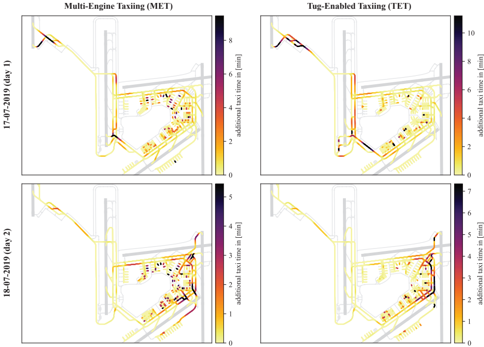
Figure 7.6: Delay hotspots depicted through additional taxi time per layout location for each day and each taxiing mode of operation
