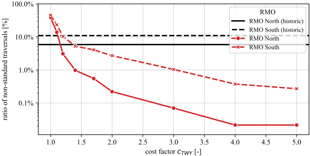
Figure 9.5: Ratio of non-standard taxiway traversals w.r.t. all traversals for two operational days under varying runway modes of operation (RMO). Black lines indicate ratios of the historical operations, red lines those of the simulated operations for varying values of the cost factor c_{TWY} .
