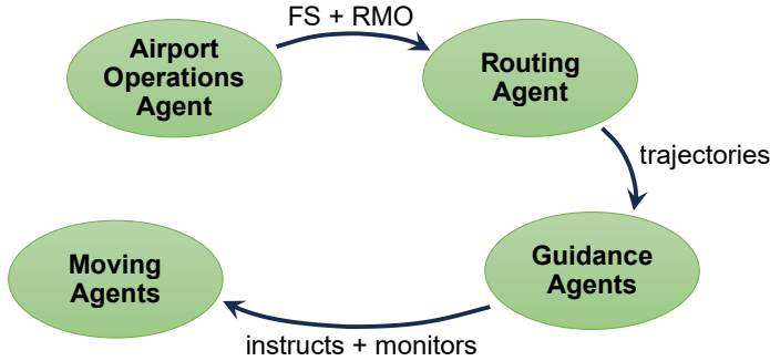
Figure 7.1: Overview of multi-agent system for automated multi-engine and tug-enabled taxiing operations
