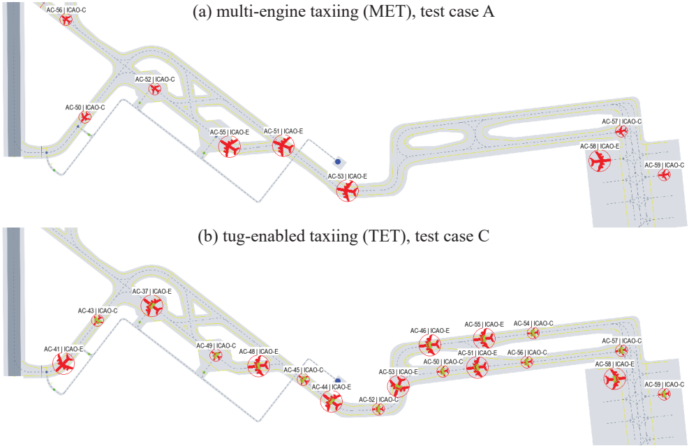
Figure 5.10: Simulation snapshots at \approx 60 min into continuous schedule with t_{\text{cycle}} = 7.5 min and depth-first search
