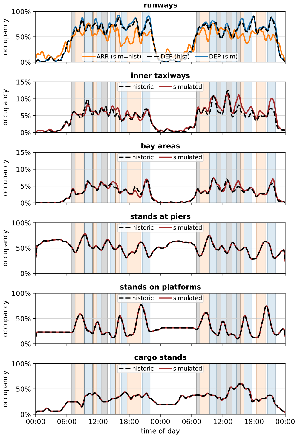
Figure 8.16: Comparison of occupancy rates in different areas of the airport between historical and simulated operations
