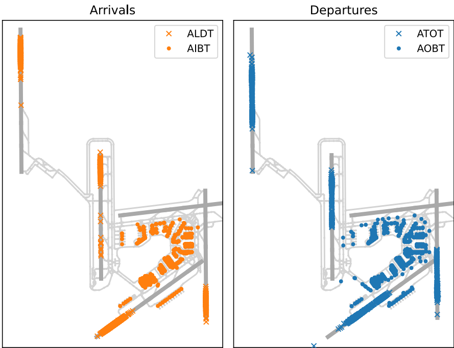
Figure 6.9: Aircraft positions at historical A-CDM milestones for inbound (left) and outbound flights (right)
