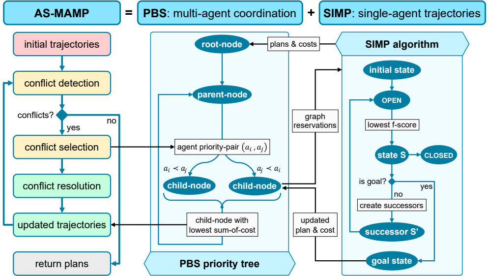
Figure 4.1: Overview of the Multi-Agent Motion Planning on Airport Surfaces (AS-MAMP) algorithm; the representation of the SIMP algorithm is simplified, see the pseudocode in Algorithms 3 and 4 for details
