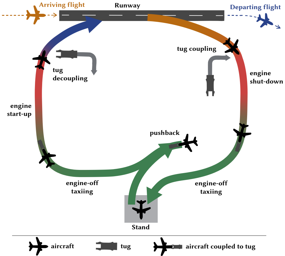
Figure 1.3: Schematic overview of how the TaxiBot concept serves as engine-off technique during inbound and outbound taxiing; based on [12]
