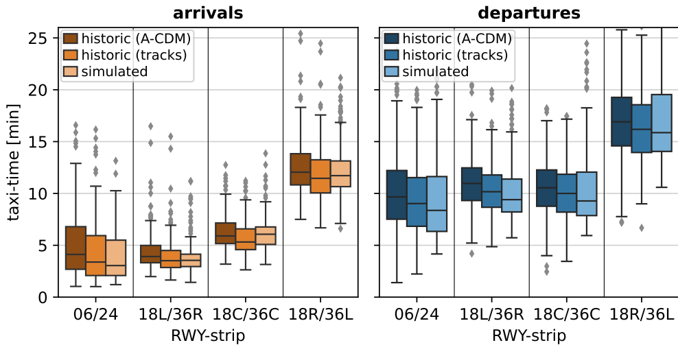
Figure 8.11: Box-and-whisker plots of taxi time distributions of historical A-CDM milestones, historical tracks, and simulated operations for arriving and departing flights per runway-strip
