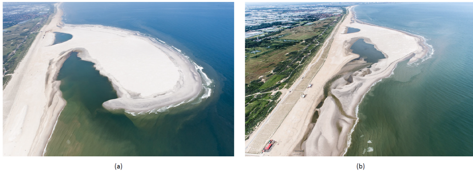
Figure 4.1.: Aerial photos of the SE, taken from the North, in a) July 2011 (shortly after construction) and b) July 2022 (after the first year). Source: Rijkswaterstaat and van Houdt (2012)
