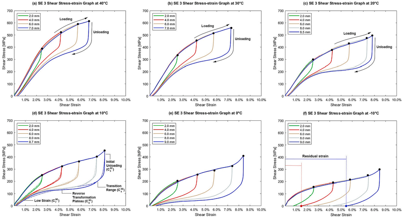
Fig. 5. Superelastic tests in different temperatures. For each experiment, 4–5 loading–unloading cycles are conducted with the displacement-control method. Subgraphs (a)–(c) indicate the SE loading and unloading process with arrows. In subgraph (d), the coloured dash-dotted curves are the fits (for the unloading curves) established in section 5.3.2. Every unloading curve is divided into four segments: initial unloading part, transition range, reverse transformation plateau and low strain. Each segment of the unloading curve has a coefficient (corresponding to Eq. (9)) which affects its shape.
