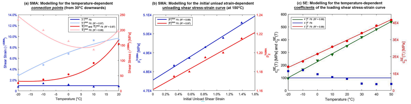
Fig. 6. (a) Modelling for the temperature-dependent connection points (from 30 °C downwards). The data points correspond to (\gamma_i^{SMA}, \tau_i^{SMA}) of the fitting functions in Fig. 4(a) of the manuscript. The full lines are the fitting models (Eqs. (3) and (4)). (b) Modelling for the initial unload strain-dependent of the unloading shear stress-strain curve (at 150 °C). The data points are the fitting parameters (Eq. (5)) of the SMA unloading model (dash-dotted lines in Fig. 4(b)). The full lines are the models which characterize the relationship between p_1^{hSMA} , p_2^{hSMA} and the initial unload shear strain (Eq. (6)). (c) Modelling for the temperature-dependent coefficients of the SE loading shear stress-strain curve. To simplify, c_2^{SE} is modelled as a constant. The data points correspond to the fitting parameters of the coloured dash-dotted lines in Fig. 4(c). The full lines are the fitting functions of the data points.
