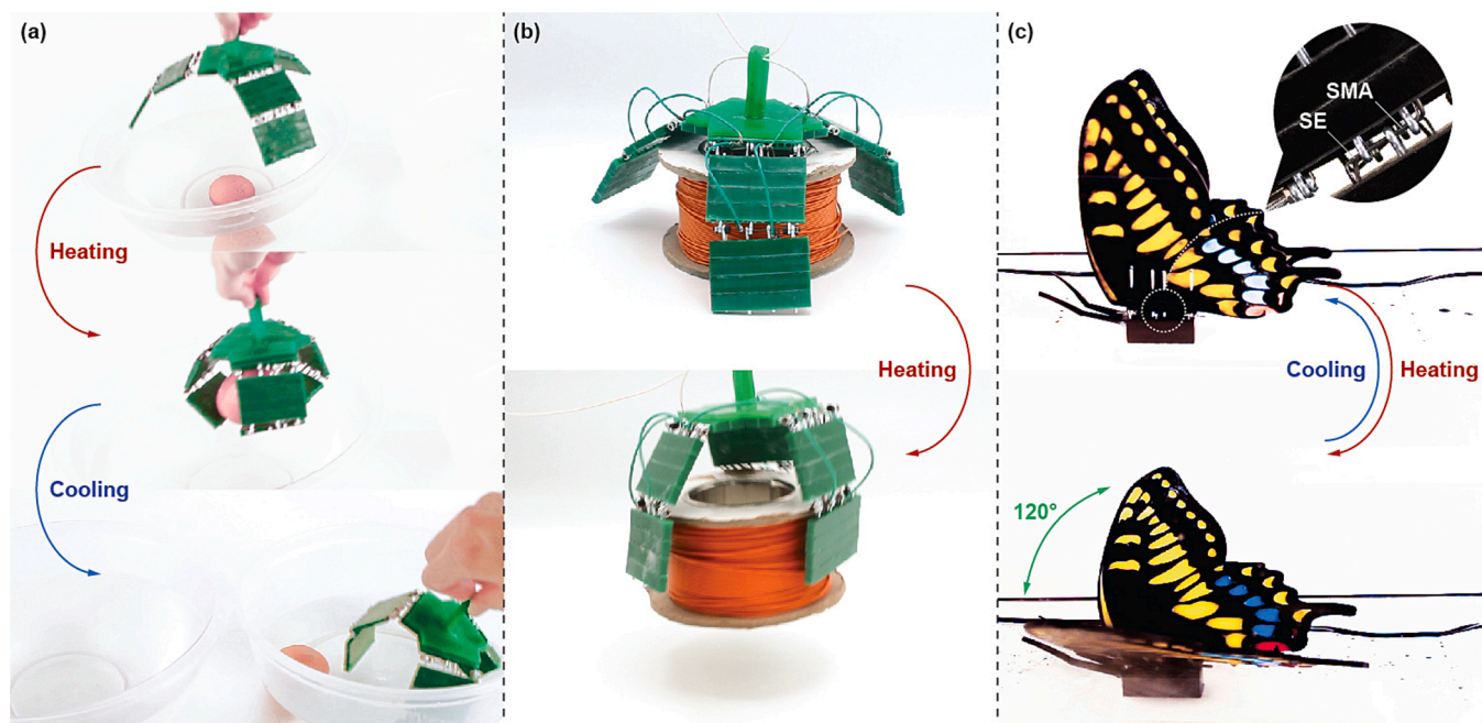
Fig. 12. Application examples. (a) and (b) A gripper constructed by 6 reversible torsion hinge actuators. It is able to grab up an egg when actuated in hot water, and release in cold water. It can also lift up a 0.6 kg wire bundle easily. (c) A butterfly demonstrator is constructed by two reversible hinge actuators.
