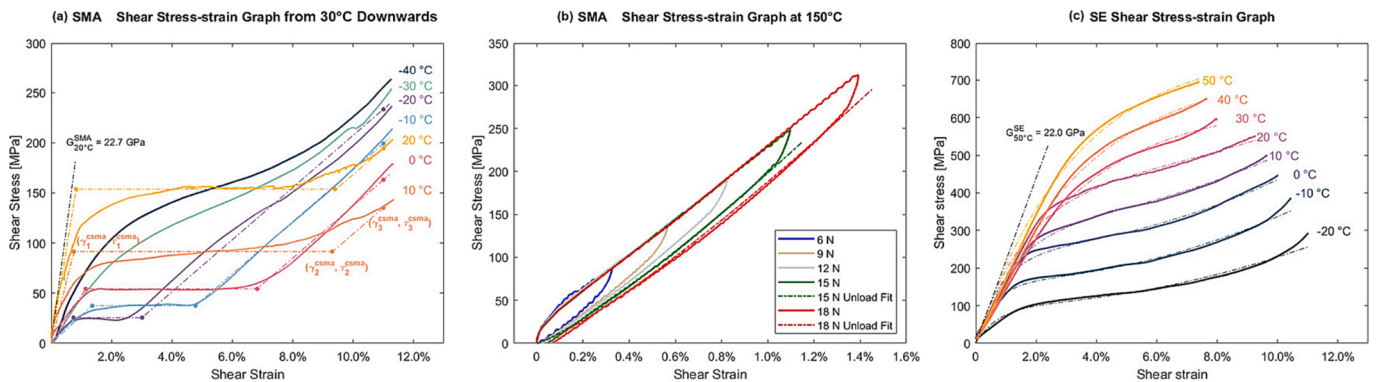
Fig. 4. (a) SMA shear stress–strain curves from 30 °C downwards. The coloured dash-dotted lines and colour points ( \gamma_i^{SMA} , \tau_i^{SMA} ) are used for modelling in section 5.2.1. (b) SMA shear stress–strain curves at the heated state (150 °C). The coloured dash-dotted curves are also used for modelling in section 5.2.2. (c) SE shear stress–strain loading curves at different temperatures. The coloured dash-dotted curves are used for modelling in section 5.3.1. The dash-dotted black line corresponds to the shear modulus obtained from the dynamic measurements of Fig. 3(c).
