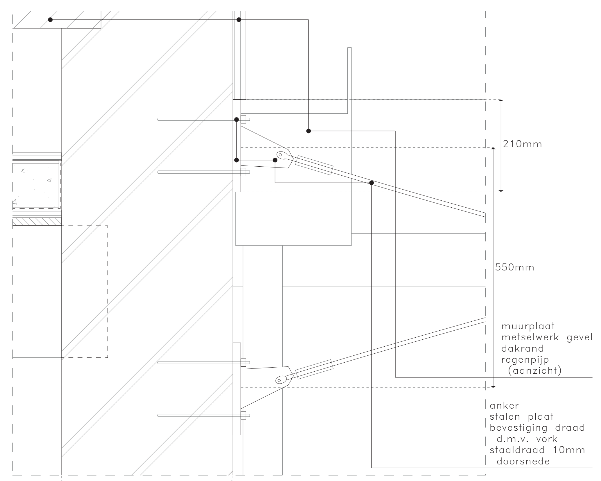
4. GLASS ROOF - FACADE 1:5
