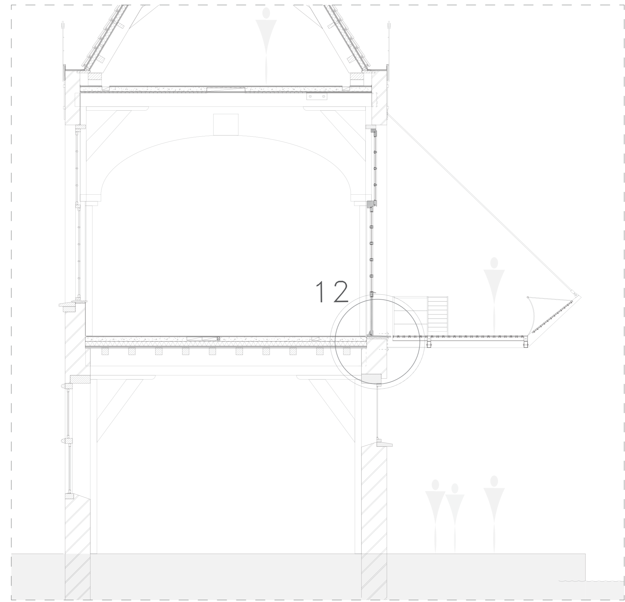
4. CROSS SECTION: SCALE 1:50 GIRDERS PERPENDICULAR TO WALL > OPENING
