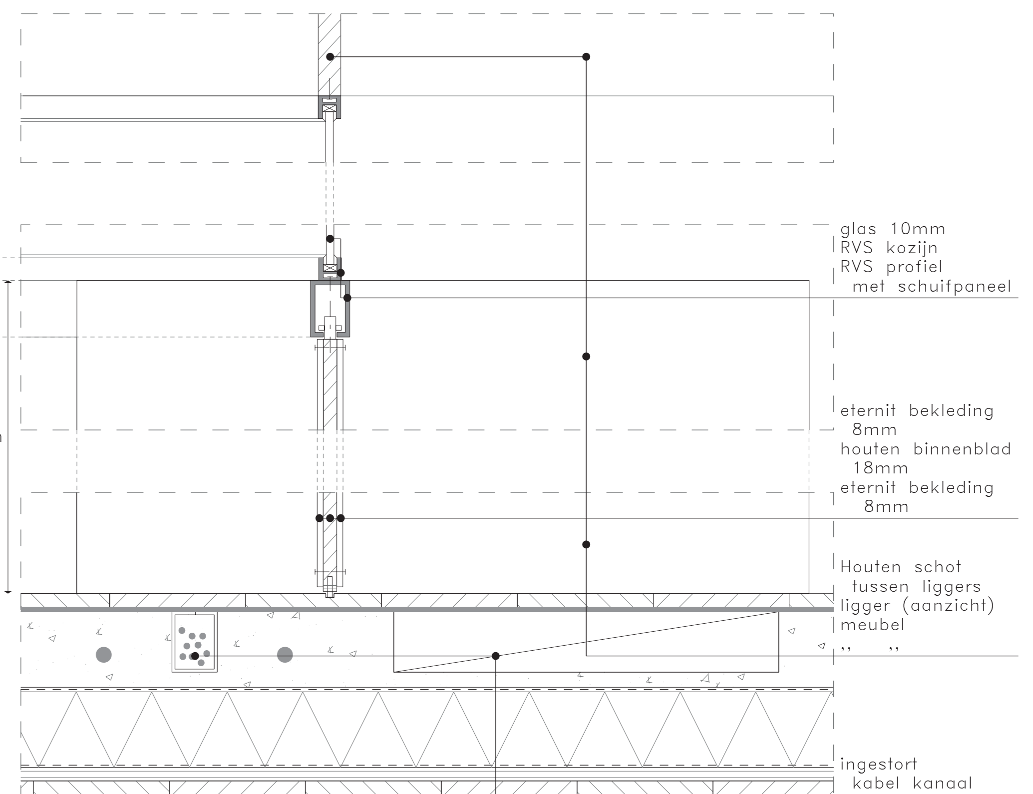
8. FURNITURE 1692 1:5
