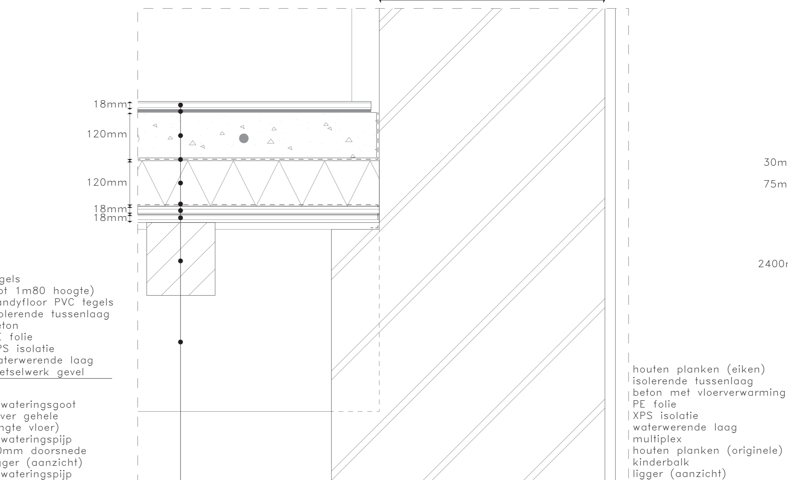
7. FLOOR - FACADE 1:5
