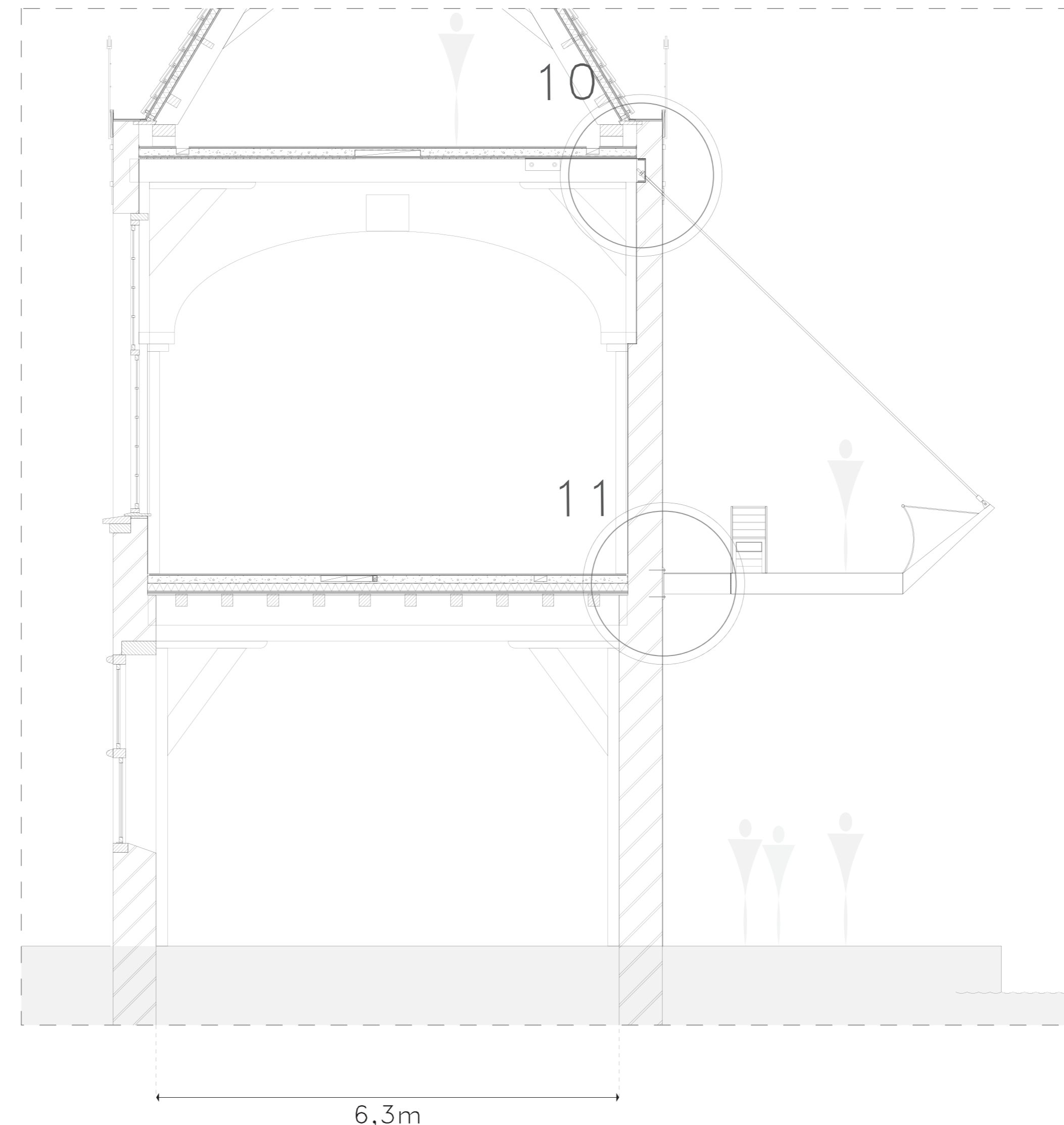
3. CROSS SECTION: SCALE 1:50 GIRDERS PERPENDICULAR TO WALL
