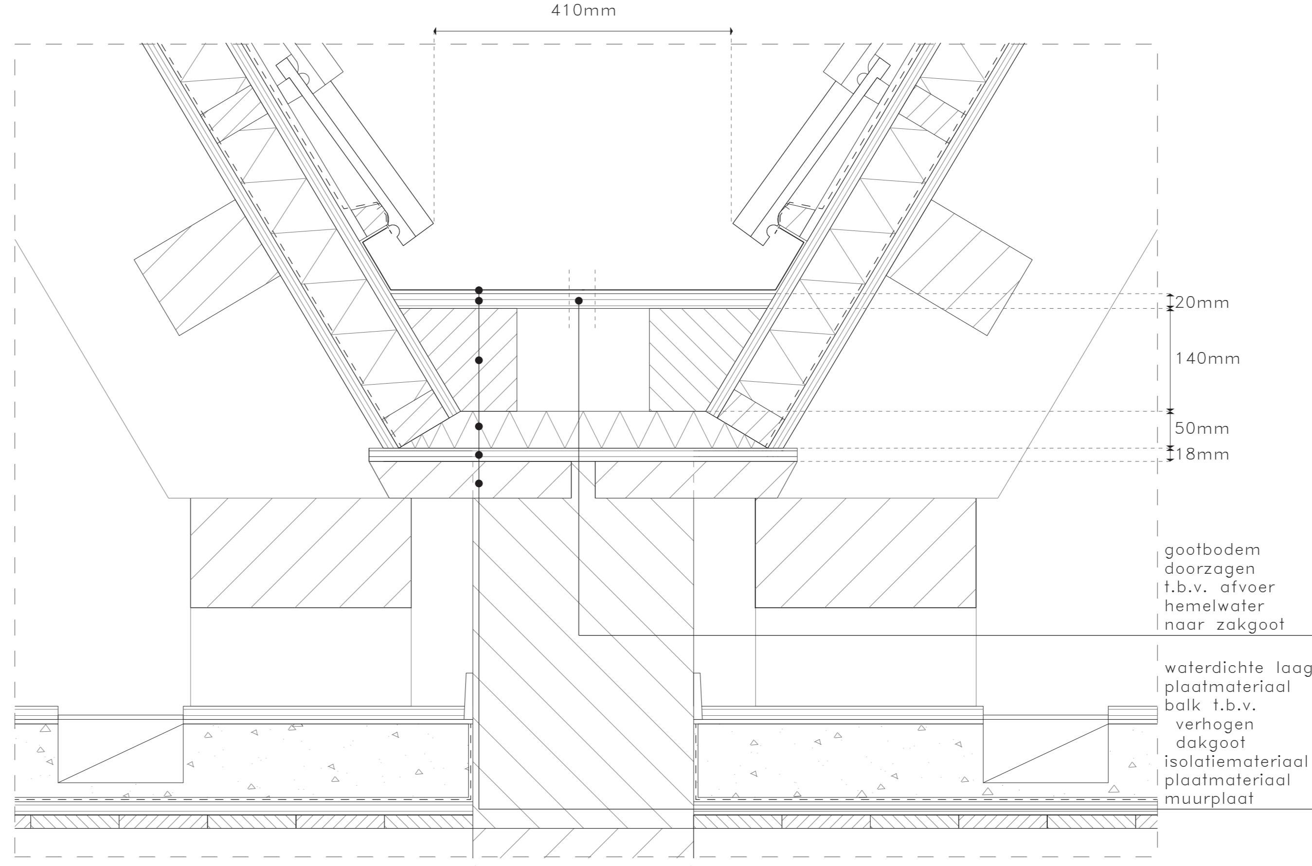
3. GUTTER BETWEEN ROOF SLOPES 1:5
