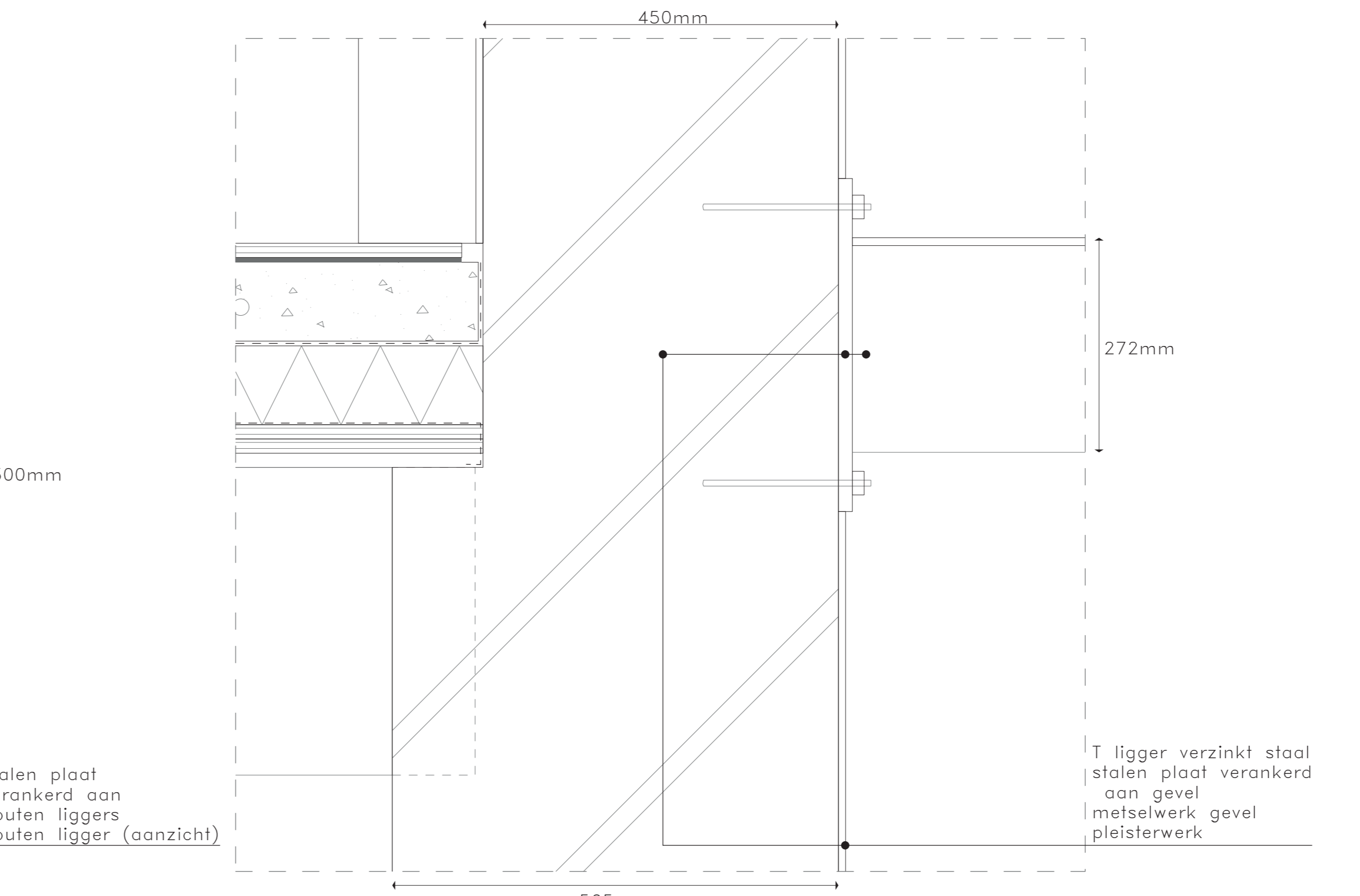
11. STREET - FACADE 1:5
