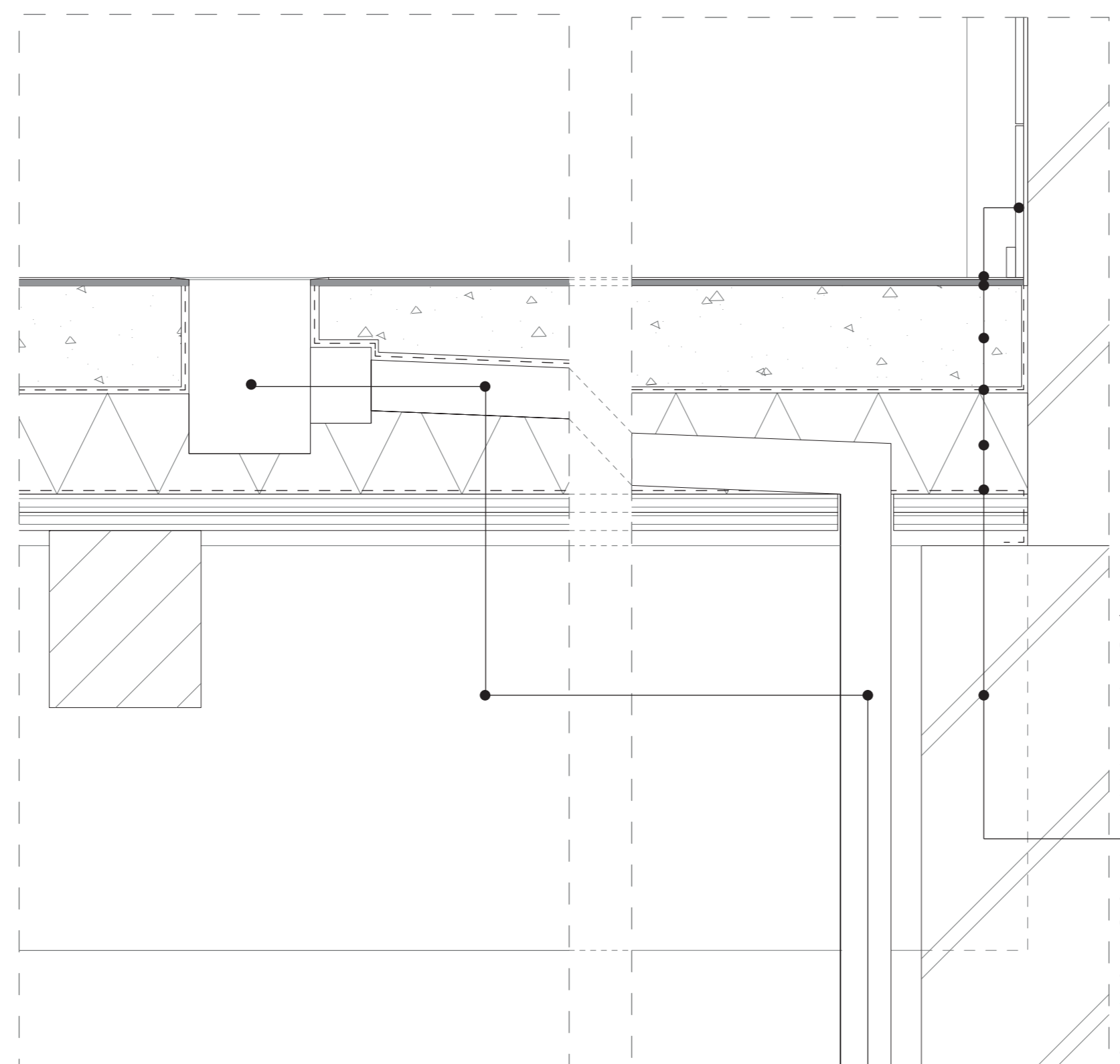
6. DRAIN KITCHEN 1:5
