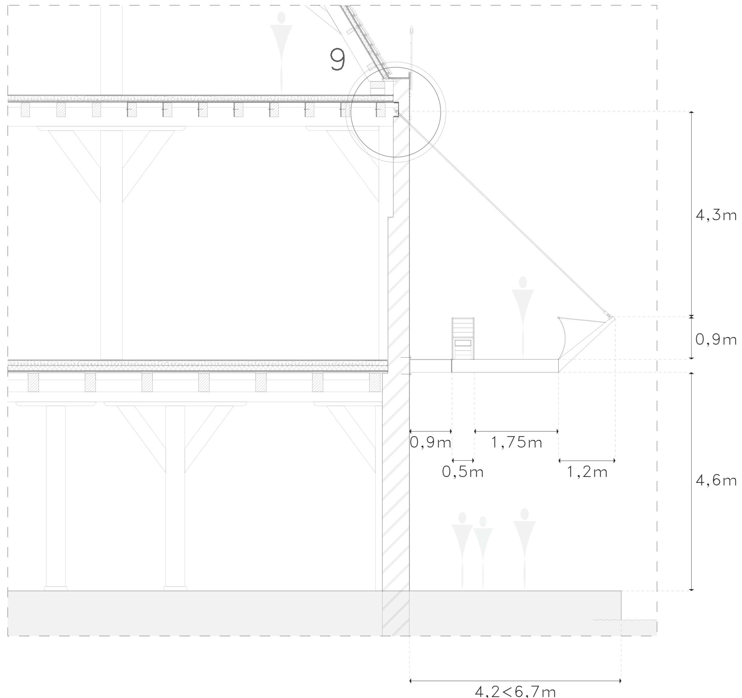
2. CROSS SECTION: SCALE 1:50 GIRDERS PARALLEL TO WALL
