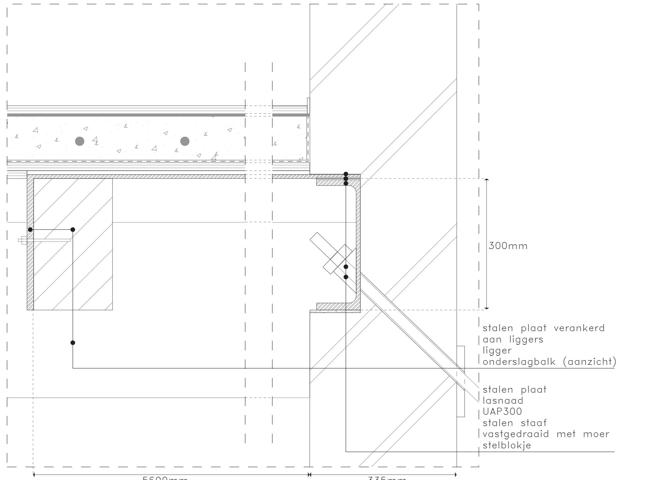
9. STREET - GIRDERS 1:5
