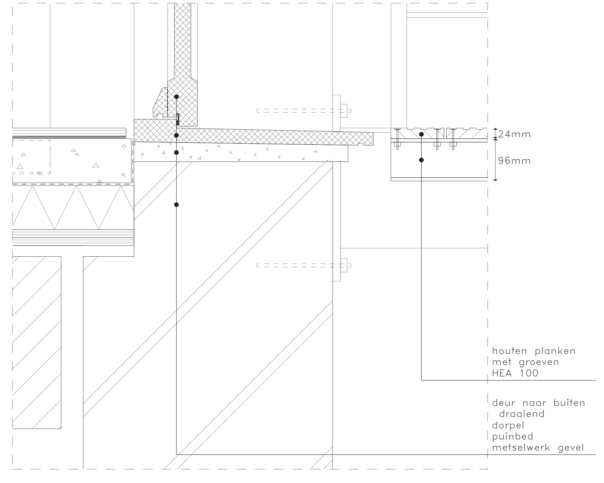
12. STREET - ENTRANCE 1:5
