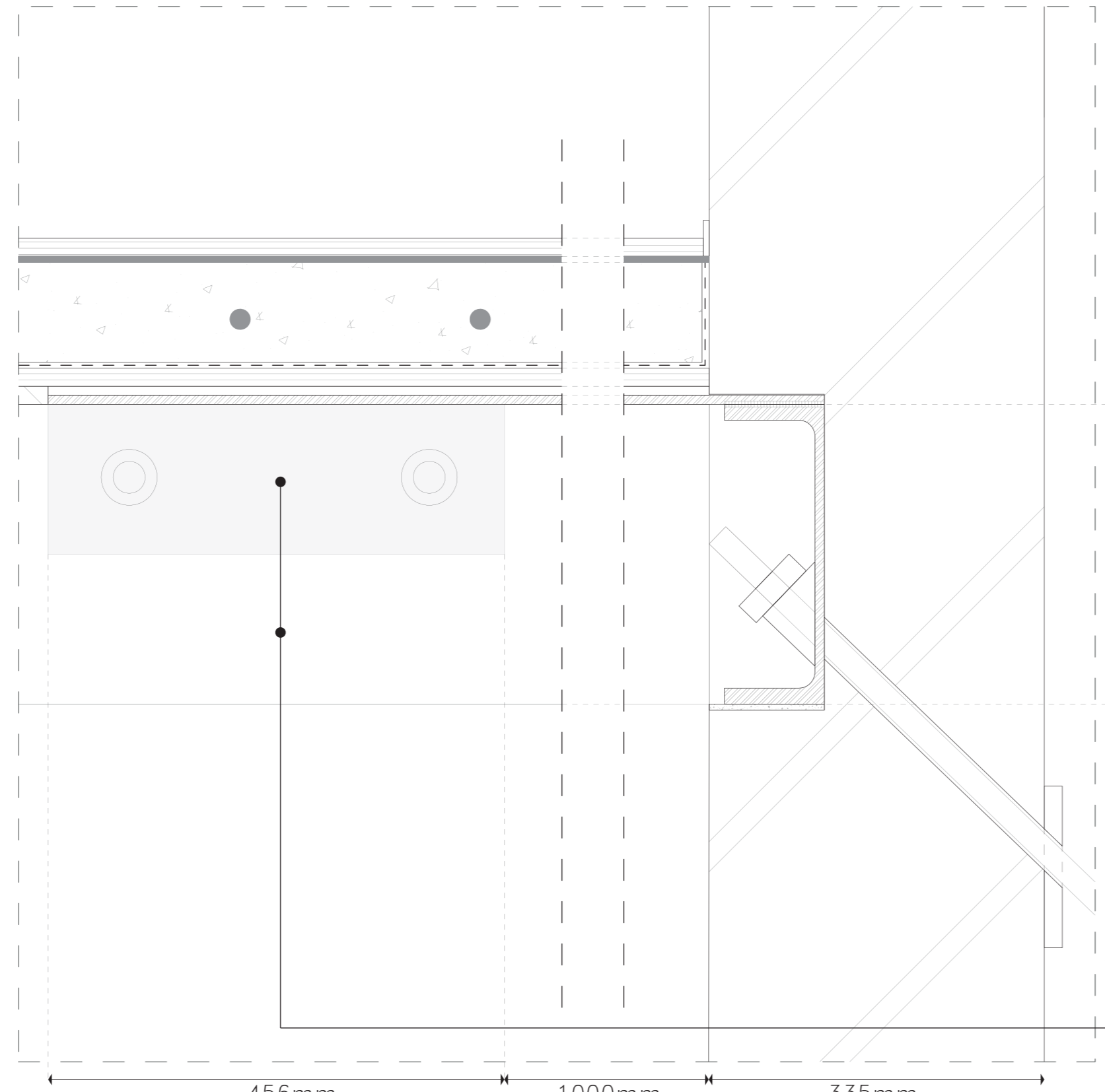
10. STREET - GIRDERS 1:5
