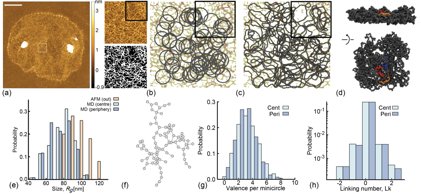
FIG. 6. (a) Figure showing a kDNA image (the scale bar is 2\ \mu\text{m} ) and an enlarged 1\ \mu\text{m}^2 region with the corresponding thresholded image (black and white). (b) Starting configuration of the AFM steered MD: 90 rings are placed randomly in a quasi-two-dimensional simulation box. Phantom beads (yellow, orange, and red in the figure) are static and act as Gaussian attracting basins. (c) At the end of the MD simulation, we obtain ensembles of conformations that capture the correct length and size of minicircles, display no ambiguous crossings with other rings, and are compatible with the underlying AFM image. (d) Snapshot of the resulting network after having removed the slab confinement. (e) Distributions of R_g of the minicircles from AFM (picked from outside the kDNA) and of the simulated ones (both from the center and periphery). (f) Network representation of (d), where each node is a minicircle and an edge between nodes represents that they are linked. Our simulated networks typically have all the nodes in one large connected component. (g) Distribution of valence, showing that the central minicircles are on average more connected than the peripheral ones. (h) Distribution of linking number, showing that the most linked pairs are singly linked, and about 10% of them are doubly linked.
