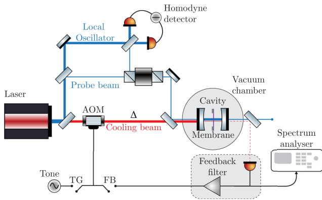
FIG. 1. A 1064 nm laser generates two beams. The probe beam, indicated by blue lines, is used to lock the laser frequency to the cavity resonance. Its phase, in which the membrane mechanical motion is encoded, is monitored with a homodyne scheme. The cooling beam, represented by red lines, provides the optomechanical interaction and is enclosed within a feedback loop. After being transmitted by the cavity, its amplitude is detected and the resulting signal is electronically processed and used to modulate the amplitude of the input field. In this way both the noise properties of light and the cavity susceptibility are modified.
