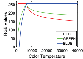
Figure 3: RGB values in different color temperature [6].
