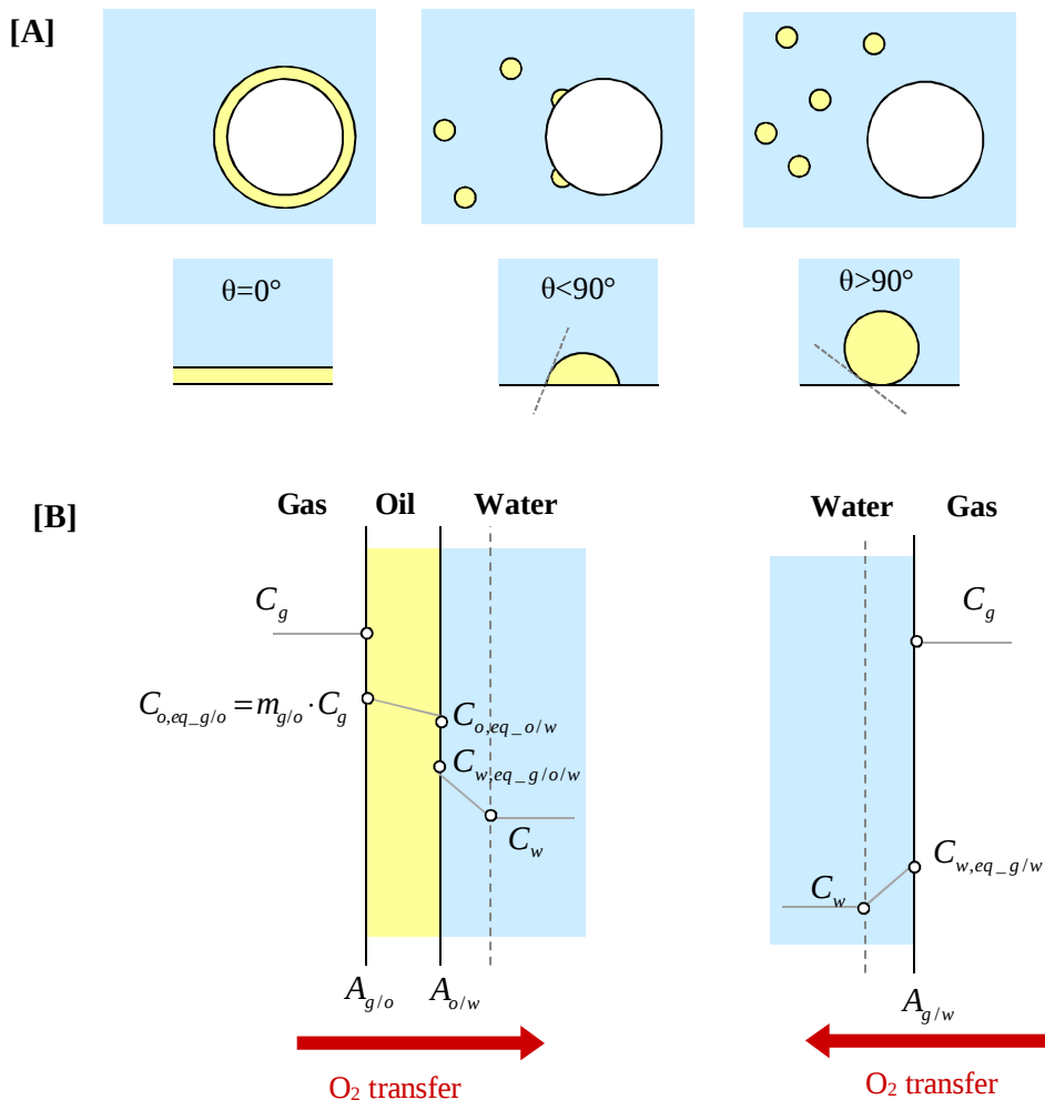
Figure 1 [A] three different scenarios for interactions between gas-oil-water (g/o/w) phases. Depending on the g/o contact angle ( \theta ), oil droplets can spread on the bubble surface forming a thin layer \theta=0^\circ , partially spread on the bubble surface forming beads \theta<90^\circ ; mostly remain dispersed in the aqueous medium \theta>90^\circ . [B] Depending on the interaction, oxygen can be transferred from the bubble to the aqueous medium via oil phase (left) or directly across the bubble surface (right). Due to the higher solubility of oxygen in hydrocarbons, the solubility of oxygen in water can be increased in the presence of oil.
