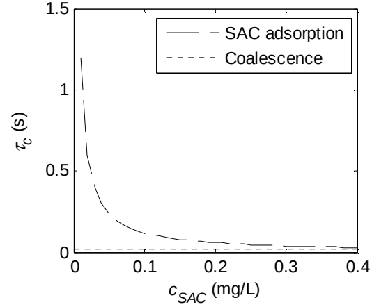
Figure 7. Characteristic times ( \tau_c ) of SAC adsorption and coalescence for d_{max} as a function of SAC concentration ( V_r = 1 \text{ m}^3 , H/D = 4 , v_{gs} = 5 \text{ cm s}^{-1} , \phi_{oil} = 0.1 ).
