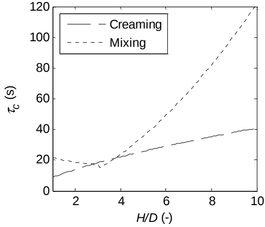
Figure 10. Characteristic times ( \tau_c ) of creaming and mixing for d_{\max} as function of aspect ratio ( V_r = 1\text{m}^3 , v_{gs} = 5\text{ cm s}^{-1} ).
