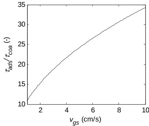
Figure 8. Coalescence is an order of magnitude faster than droplet stabilization ( V_r = 1 \text{ m}^3 , H/D = 4 , c_{SAC} = 0.1 \text{ mg L}^{-1} , \phi_{oil} = 0.4 ).
