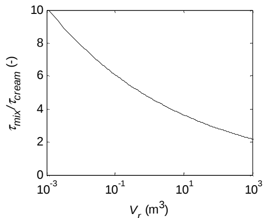
Figure 12. Ratio characteristic times of mixing and creaming for d_{max} ( v_{gs} = 5 \text{ cm s}^{-1} , H/D = 15 ).
