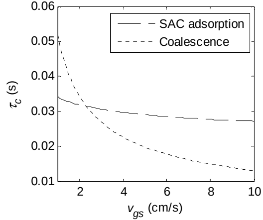
Figure 5. Characteristic times ( \tau_c ) of SAC adsorption and coalescence for d_{max} as a function of superficial gas velocity ( V_r = 1 \text{ m}^3 , H/D = 4 , c_{SAC} = 0.4 \text{ mg/L} , \phi_{oil} = 0.1 ).
