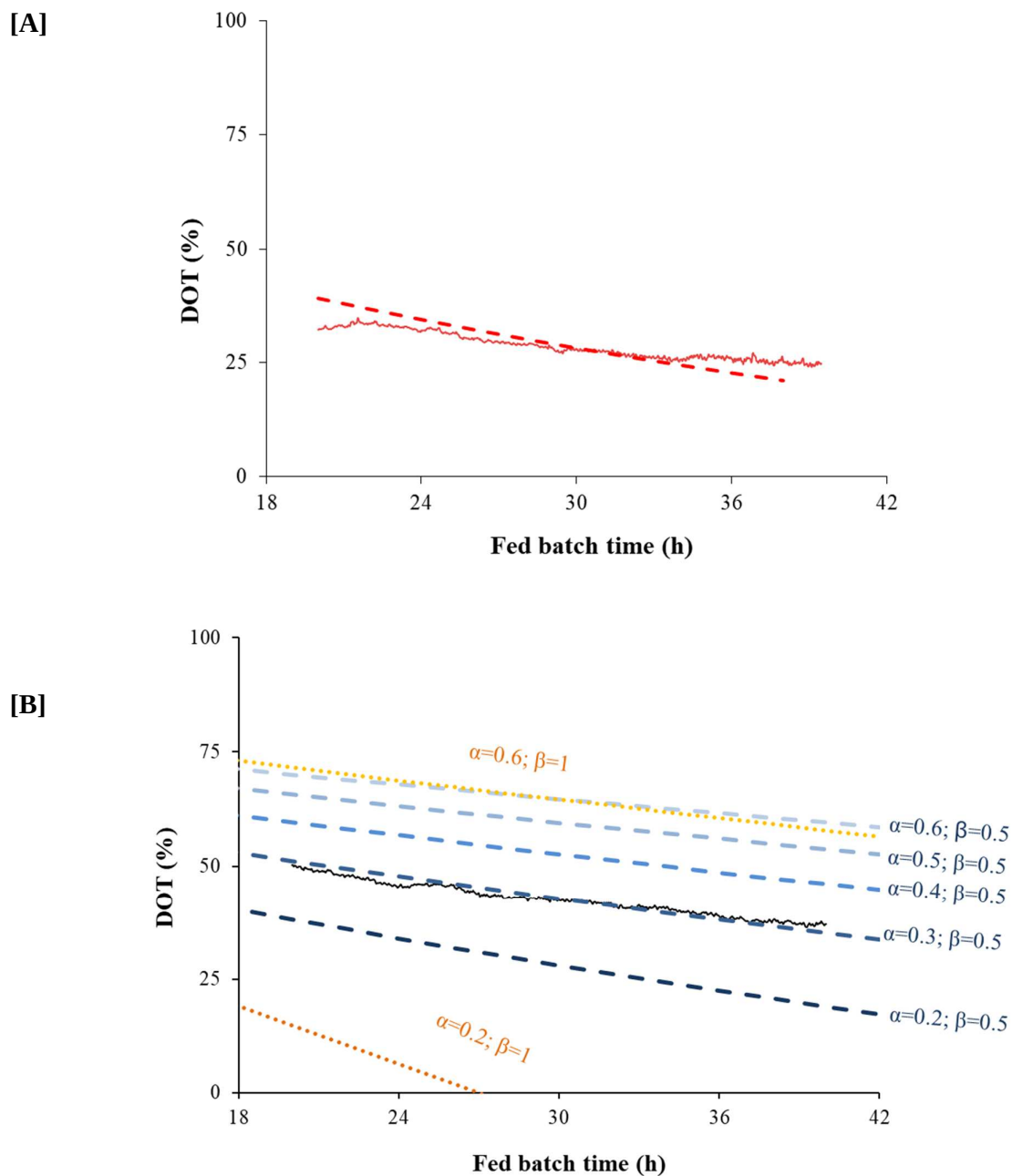
Figure 2. [A] Comparison of experimental DOT profile in F01 without oil to a modelled DOT profile ( \alpha=0 ; \beta=0 ; R^2=0.72 ). [B] Comparison of experimental DOT profile in F02 containing 7.5% v/v of hexadecane to model trends based on different oil enhancement ( \alpha ) and bubble coverage ( \beta ) values ( R^2=0.74 ).
