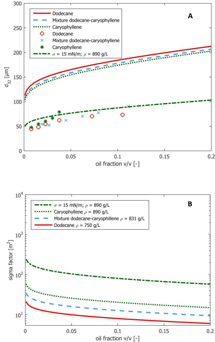
Figure 3: Theoretical values of droplet size (A) and required sigma factor (B) for recovering oil droplets in a disk stack centrifuge of 30% efficiency and 11 \text{ L s}^{-1} capacity as function of oil fraction estimated at a constant power input of 2.4 \text{ W kg}^{-1} (corresponding to 1.5 kg fermentor, stirring rate of 1000 rpm, and 1 vvm of gas flow) compared to experimental droplet size values (indicated as markers) at power input ranging from 2.2-2.7 \text{W kg}^{-1} (corresponding to 1.275 L of water and different amounts of caryophyllene and dodecane). Potential effect of lowering interfacial tension to 15 \text{ mN m}^{-1} by surface active components in a caryophyllene/water dispersion is also shown.
