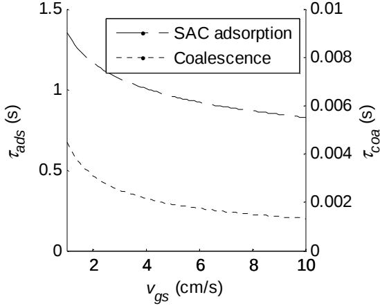
Figure 4. Characteristic times of SAC adsorption and coalescence for d_{min} as a function of superficial gas velocity ( V_r = 1 \text{ m}^3 , H/D = 4 , c_{SAC} = 0.4 \text{ mg/L} , \phi_{oil} = 0.1 ).
