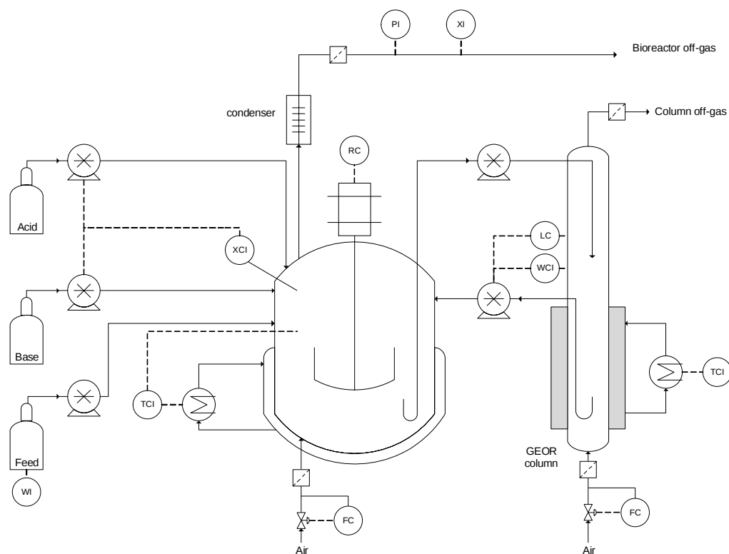
Figure 2. [A] Overview fermentation stages in the different experiments. [B] Schematic representation of the integrated system. P-pressure; X-composition; R-agitation speed; T-temperature; W-weight; F-mass flow; L-level; I-indicator; C-controller.
