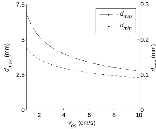
Figure 3. The minimum and maximum droplet diameters at varying superficial gas velocities ( V_r = 1\text{m}^3 , H / D = 4 , c_{SAC} = 0.4 \text{ mg L}^{-1} , \phi_{oil} = 0.1 ).
