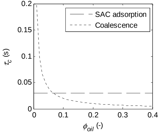
Figure 6. Characteristic times ( \tau_c ) of SAC adsorption and coalescence for d_{max} as a function of volumetric oil fraction ( V_r = 1 \text{ m}^3 , H/D = 4 , v_{gs} = 5 \text{ cm s}^{-1} , c_{SAC} = 0.4 \text{ mg L}^{-1} ).
