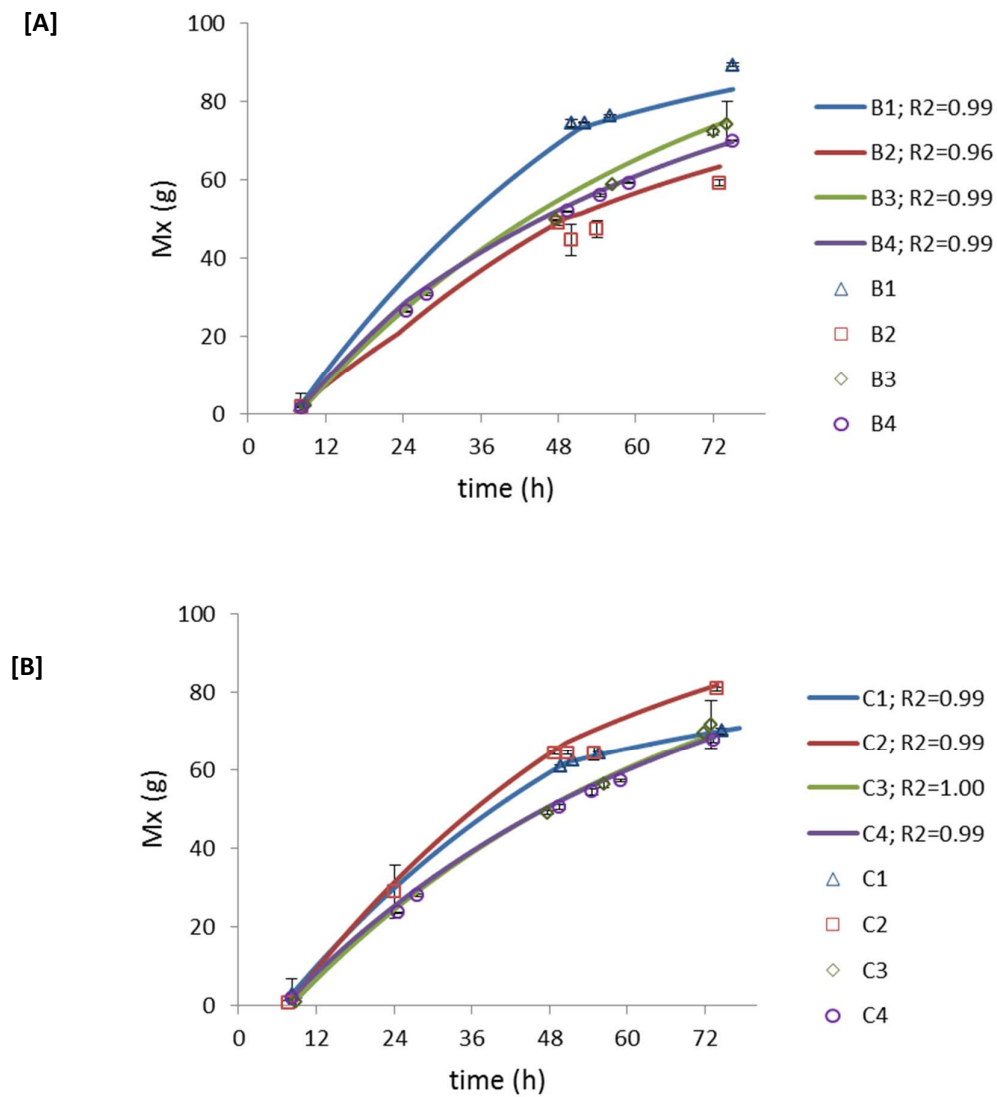
Figure 3. Total mass of cells in the reactor for base case fermentations [A] and circulation case fermentations [B]. Solid lines represent data obtained from the kinetic model. Markers represent experimental data obtained from cell dry weight measurements.
