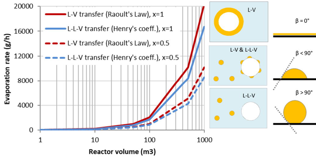
Figure 2: Maximum estimated evaporation rate at 1vvm gas flow and 35°C, as function of the fermentor working volume for two different routes: L-V modelled by Raoult's law, and L-L-V modelled by Henry's law. x=1 is the composition of an oil phase purely composed of sesquiterpene and x=0.5 represents a situation where 10%v/v of sesquiterpene is produced in a bioreactor containing 10% v/v of solvent. Distribution of oil phase on gas-water interface depends on the contact angle \beta : (i) When \beta=0^\circ oil phase is fully spread onto gas surface (ii) \beta<90^\circ oil beads with large contact area oil-gas are formed, and (iii) if \beta>90^\circ oil beads with low oil-gas contact area are formed.
