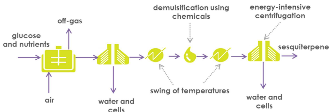
Figure 3. Block scheme of the (reported) process at large scale for the recovery of microbial sesquiterpene [36].
