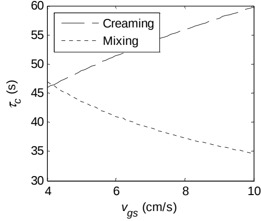
Figure 9. Characteristic times ( \tau_c ) of creaming and mixing for d_{\max} as function of superficial gas velocity in the heterogeneous regime ( V_r = 1 \text{ m}^3 , H / D = 4 , \phi_{oil} = 0.1 ).
