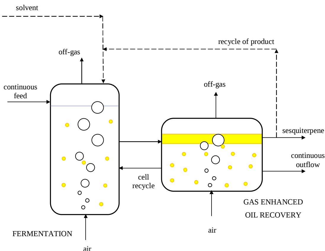
Figure 2. Schematic representation of an integrated process for continuous production and recovery of microbial sesquiterpene. In this system, the reactor would be a bubble column mixed by the power input provided by the gas bubbles. Solvents can be added to the system promoting oil coalescence and enhancing oxygen transfer. Alternatively, product could be recycled for the same purposes. Part of the fermentation broth is transferred to the gas enhanced recovery compartment where oil is separated from the aqueous phase. Broth with lower oil content is transferred back into the reactor, and the clear oil layer is removed from the top.
