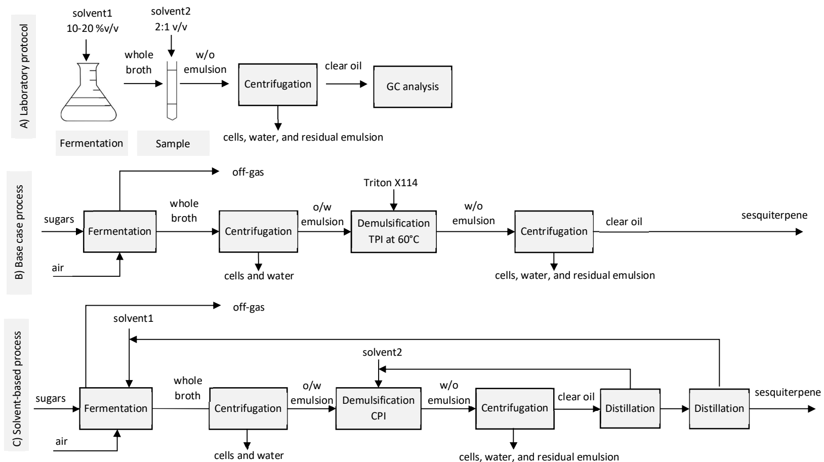
Figure 1: Process options for the production of sesquiterpenes. A) Lab scale protocol [8]; B) Base case [9]; C) Solvent-based process evaluated in this work.
