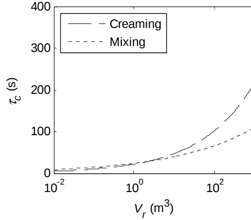
Figure 11. Characteristic times ( \tau_c ) of creaming and mixing for d_{\max} as function of reactor volume ( H/D = 4 , v_{gs} = 5\text{ cm s}^{-1} ).
