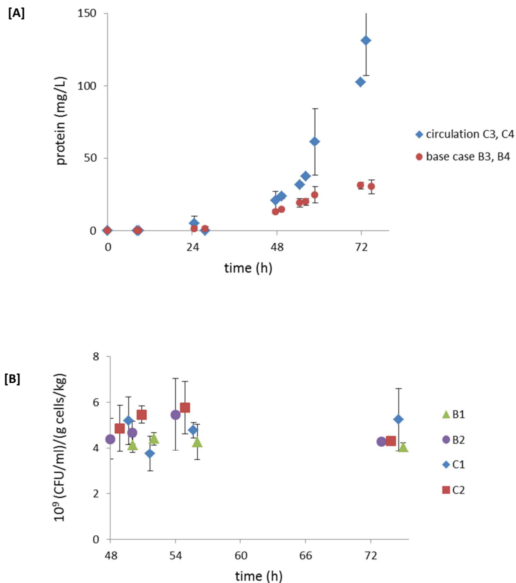
Figure 4. Comparison of base case (B1 to B4) and circulation case (C1 to C4) based on extracellular protein concentration [A] and cellular viability [B]. Error bars represent the standard deviation of the average.
