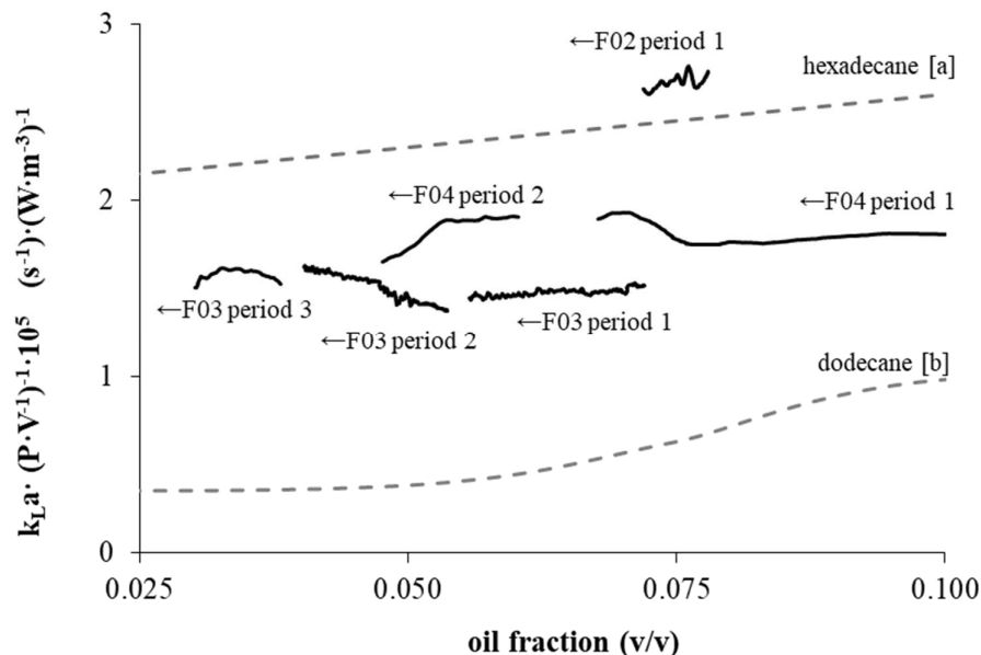
Figure 4. Experimental and literature k_La values corresponding to varying oil fractions. Continuous lines correspond to experimental data (Table 2). Dashed data correspond to literature values for (a) hexadecane in water [18] at 4000 \text{ (W} \cdot \text{m}^{-3}) and (b) dodecane in suspension of quiescent cells [15] at 963 \text{ (W} \cdot \text{m}^{-3}) . For comparison purposes, k_La values have been normalized to account for the effect of power input. Oil fraction in F02 to F04 changed due to dilution of medium during the fed batch period. Arrows indicate direction of change. While increasing values of k_La with oil fraction have been reported in literature (Pearson coefficient >0.95 ), experimental k_La \cdot (P \cdot V^{-1})^{-1} in this work was not significantly correlated to oil concentration (Pearson coefficients of F02 to F04 were +0.82, -0.64, -0.07 ).
