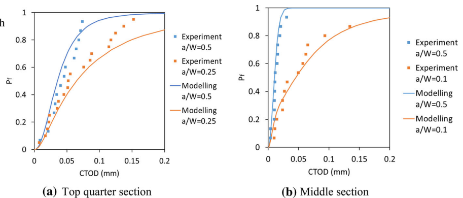
Fig. 14 P_t -CTOD curve of top quarter section in comparison with experimental data (dots are the experimental data and curves are the model predictions)
