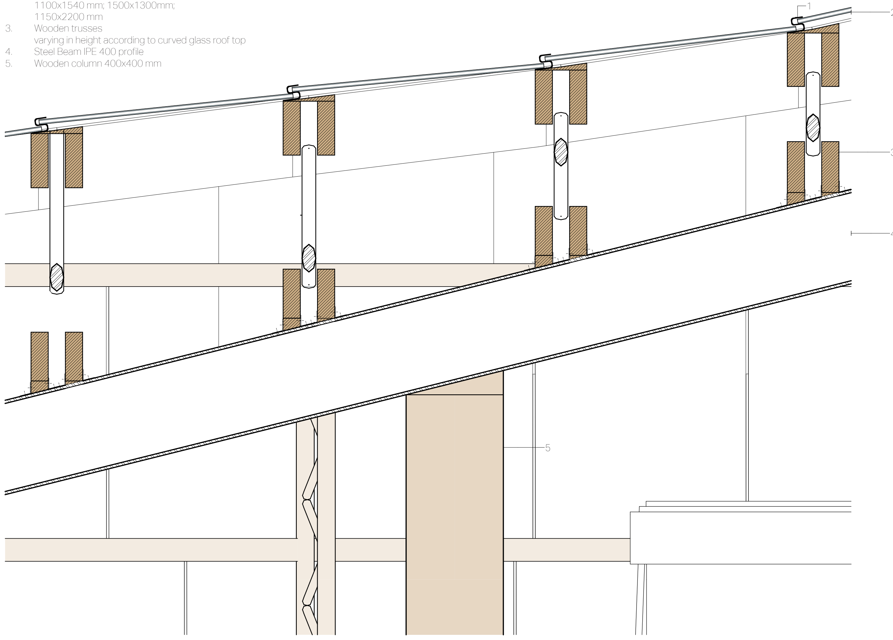
1:10 Detail Roof construction
