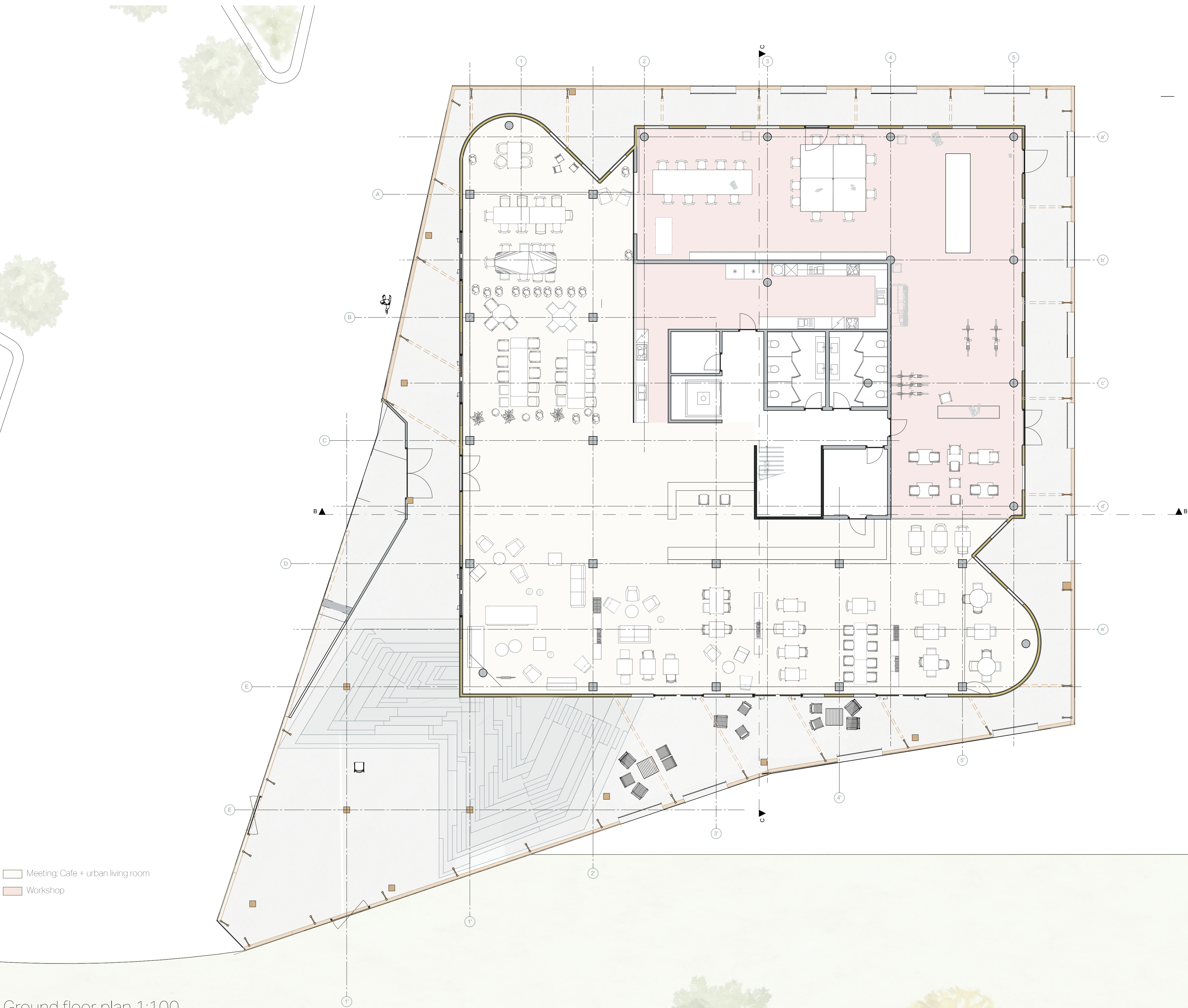
Ground floor plan 1:100
