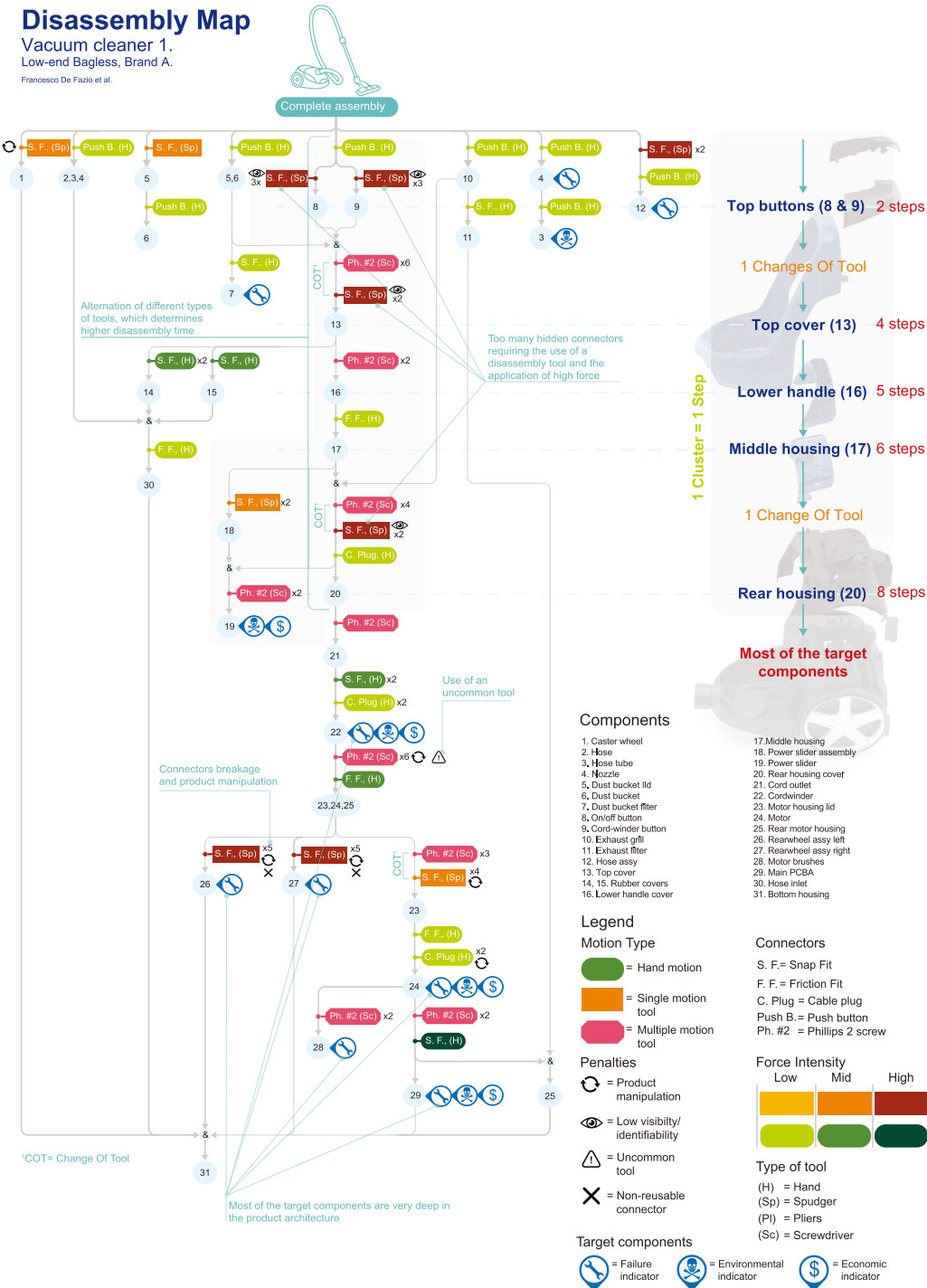
Fig. 9. Disassembly Map of the original architecture of vacuum cleaner #1.
