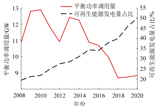
图1 德国电网平衡功率调用量及可再生能源占比 Fig. 1 Amount of balancing power called by the German Power Grid and the share of renewable energy
