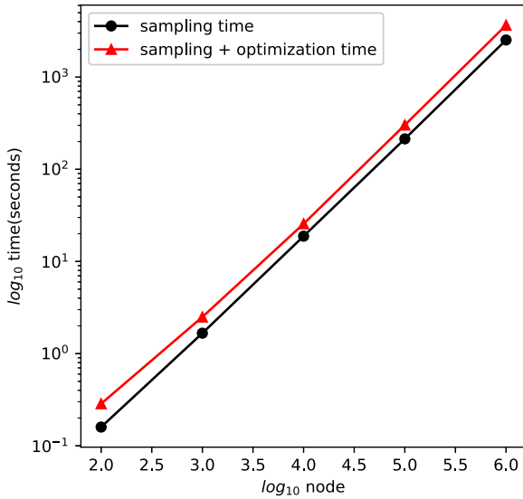
Fig. 9. Scalability of DiaRW on Barabási–Albert networks.
