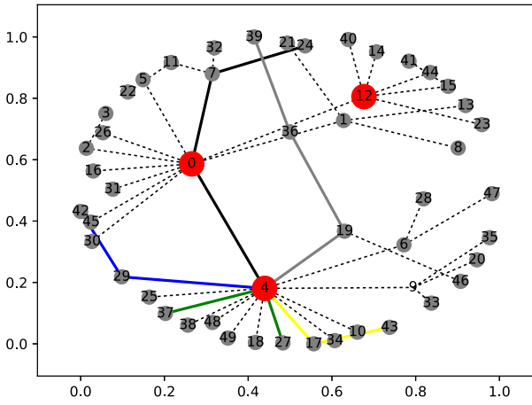
Fig. 3. An example of uniform random walk sampling on a scale-free network. It starts from hub node 4 with the number of walks 5 and walk length 4, generating node sequences (shown in solid line) like “4-29-42-29”(blue), “4-0-7-24”(black), “4-27-4-37”(green), “4-19-36-39”(gray) and “4-17-43-17”(yellow). (For interpretation of the references to color in this figure legend, the reader is referred to the web version of this article.)
