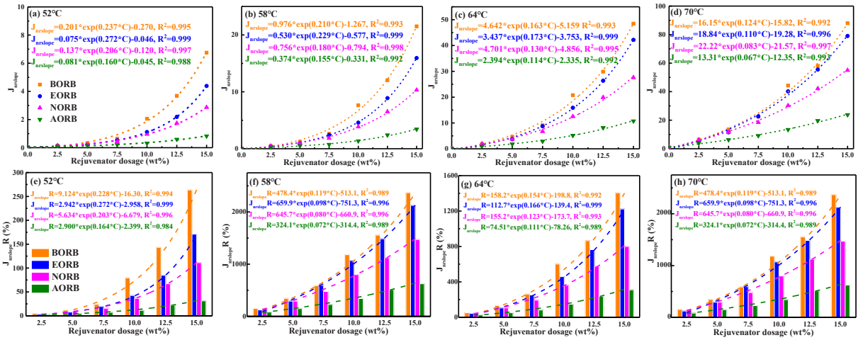
Fig. 20. The influence of rejuvenator dosage on the J_{nrslope} value at different temperatures.
