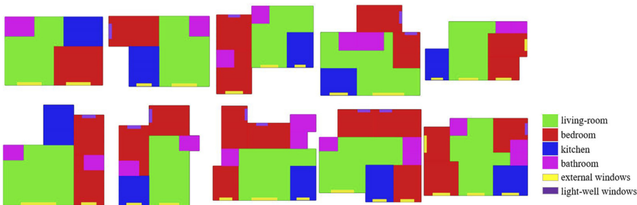
Figure 2. Floor plan alternatives assumed in generating data sets
