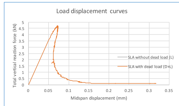
Figure 10: Dead load and point load are applied at the same position in the same direction. The curves are on top of each other.
