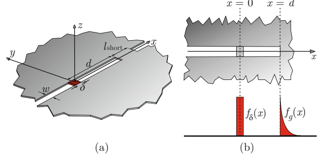
Fig. 1. (a) Interrupted infinite slot in free space. (b) Space domain basis functions with respect to their location along the semi-infinite slot.
