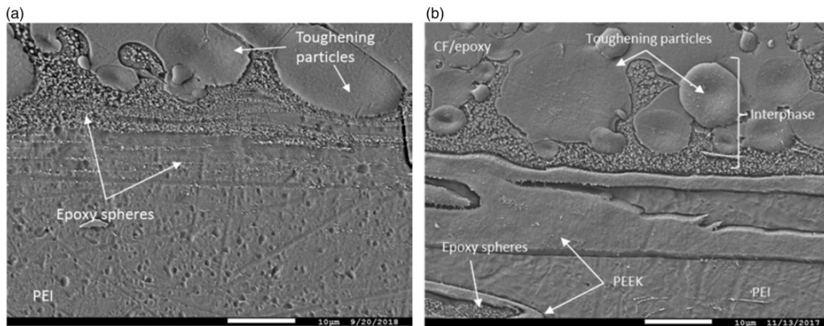
Figure 13. SEM micrographs of the cross-sections of (a) a hybrid PEI 60 sample and (b) a hybrid PEEK-60 sample. The interphase was affected by the welding process for both configurations. PEEK: polyetheretherketone; PEI: polyetherimide; SEM: scanning electron microscopy.
