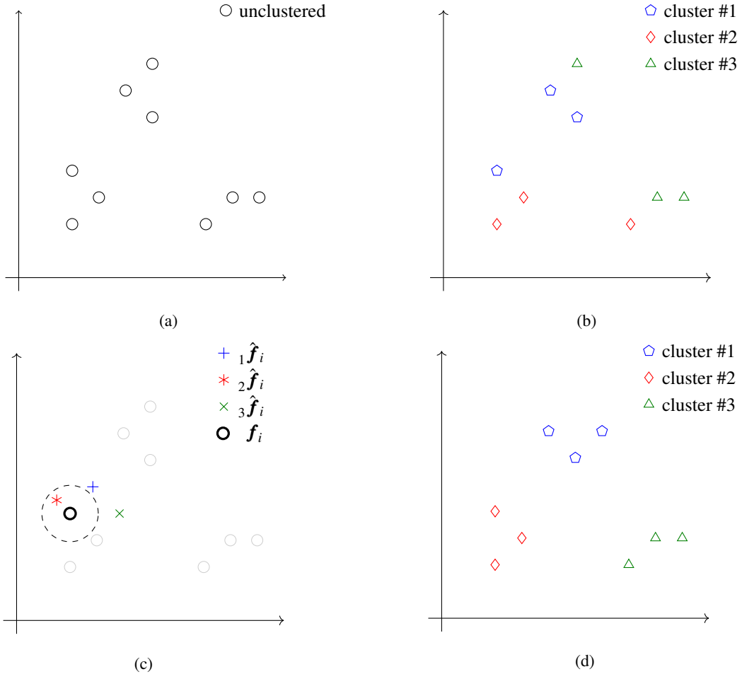
Figure 1: Modified k -means clustering algorithm: (a) unclustered samples; (b) initial clustering of samples; (c) distance between a sample \mathbf{f}_i and its DEIM approximation using {}_c\mathbf{A} and {}_c\mathbf{P} of all clusters, c = 1 \dots n_c . The sample \mathbf{f}_i belongs to the cluster that generates the closest {}_c\hat{\mathbf{f}}_i = {}_c\mathbf{A} {}_c\mathbf{P}^T \mathbf{f}_i in the sense of (28); (d) final form of clusters after convergence of the modified k -means clustering algorithm.
