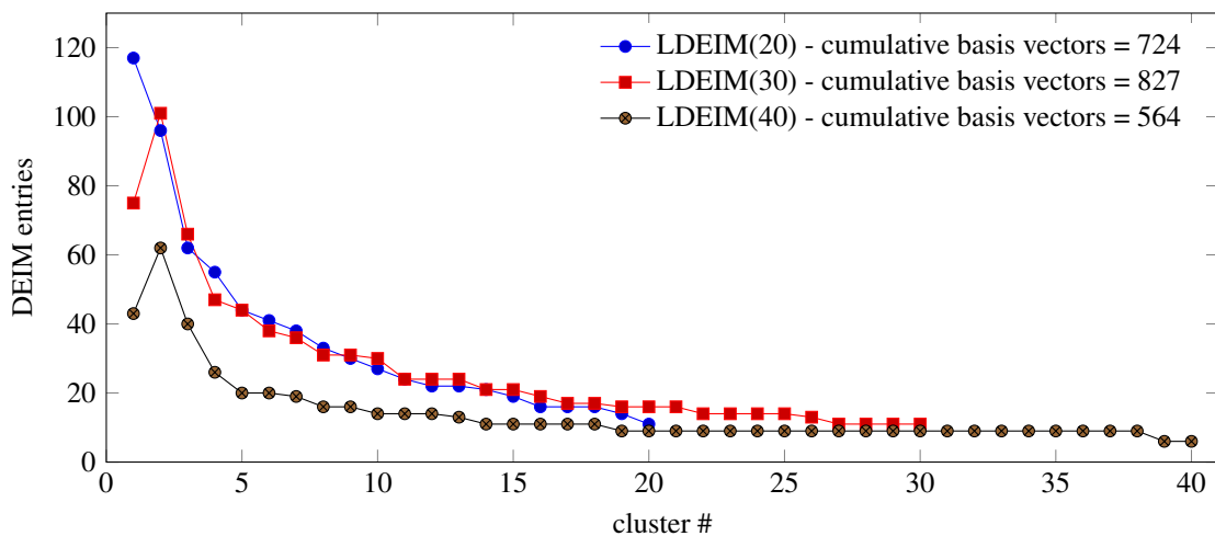
Figure 13: Footing: number of the DEIM entries in each cluster (reduced order model: 609 POD basis vectors associated with the displacement field).
