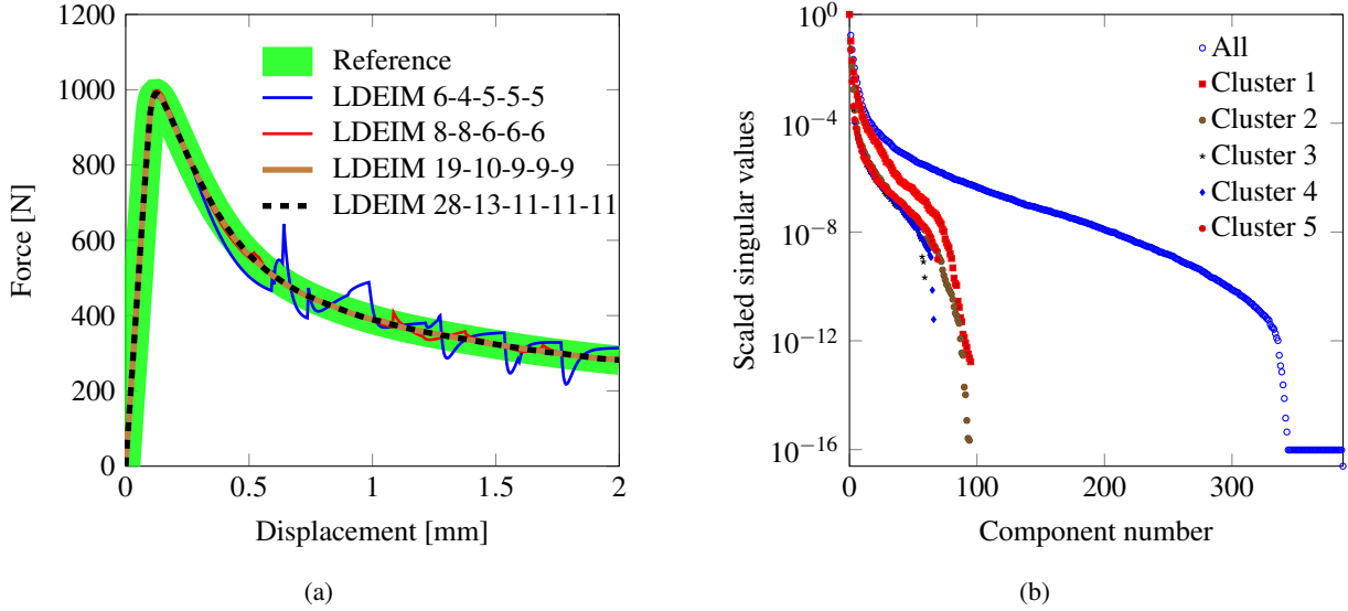
Figure 6: Performance of the LDEIM approximation in the two-dimensional strain localization problem: (a) basis addition study (reference solution: 1350 DOFs, 196 elements; reduced order model: 227 POD basis vectors associated with the displacement field); (b) singular values of the x component of the force vector samples using unclustered and clustered samples (those corresponding to the y and the z components follow the same trend).
