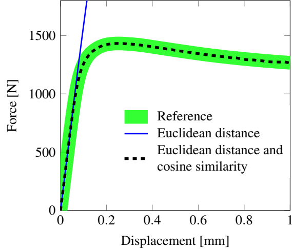
Figure 14: Footing: the effect of the distance definition on the load-displacement diagram (reference solution: 5184 DOFs, 1331 elements; reduced order model: 609 POD basis vectors associated with the displacement field, LDEIM with 40 clusters).
