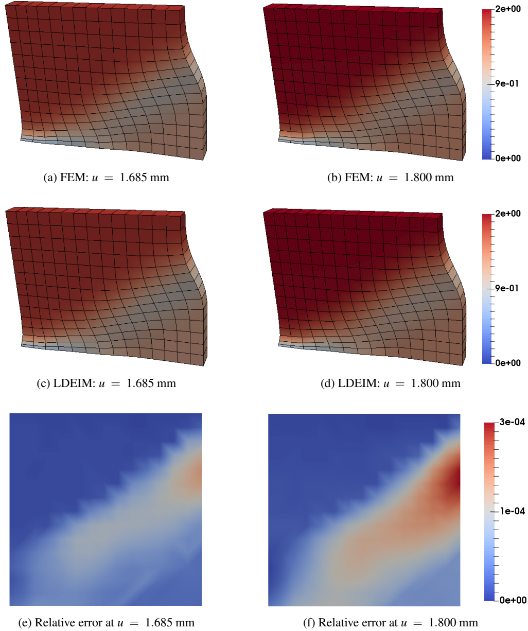
Figure 10: Two-dimensional strain localization problem: deformed configuration corresponding to the black curve depicted in Figure 9a at displacement levels corresponding to the 8th and 9th cluster changes indicated in Figure 9b. The reference FEM solution and reduced order model are depicted in the upper rows and the error between them is depicted in the bottom row.
