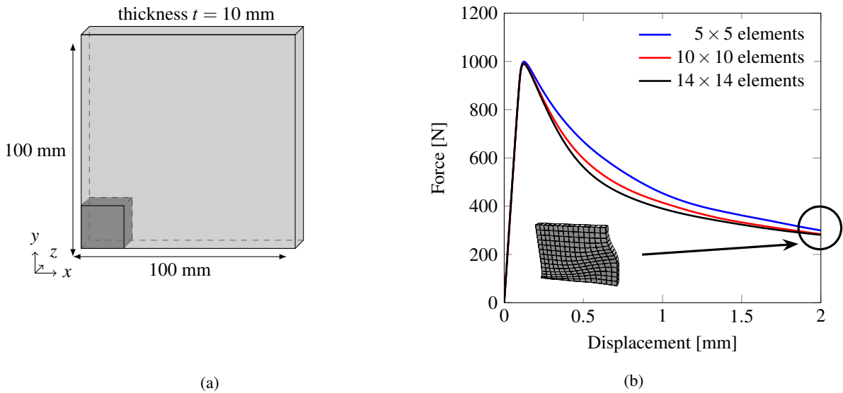
Figure 4: Two-dimensional strain localization problem: (a) geometry of the wall under compression with the dark shaded part indicating the weak region that localizes the initiation of plasticity and triggers a shear band; (b) the regularizing properties of viscoplasticity are reflected in the mesh refinement study in terms of the resultant of the force in the vertical direction on the lower edge against the value of the displacement of the upper edge; the inset shows the deformed wall with the shear band due to strain localization.
