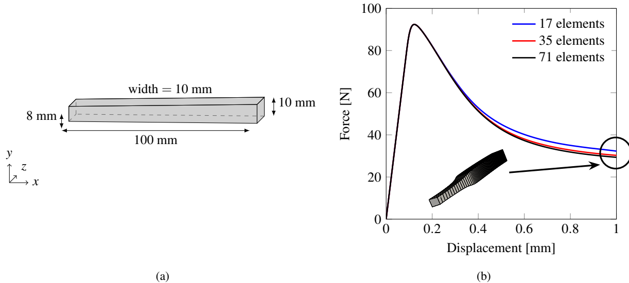
Figure 2: One-dimensional strain-localization problem: (a) the clamped end of the tapered bar has a smaller cross-section to trigger the initiation of plasticity and consequent strain localization; (b) the regularizing properties of viscoplasticity are reflected in the mesh refinement study in terms of the resultant force at the clamped end plotted against the displacement at the free end.
