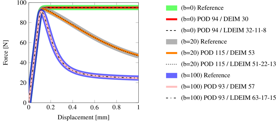
Figure 3: The MOR technique applied to the one-dimensional strain-localization problem. The reference curves are obtained with the 71 eight-node regular hexahedral element mesh (864 DOFs) using different values of the b parameter (8).
