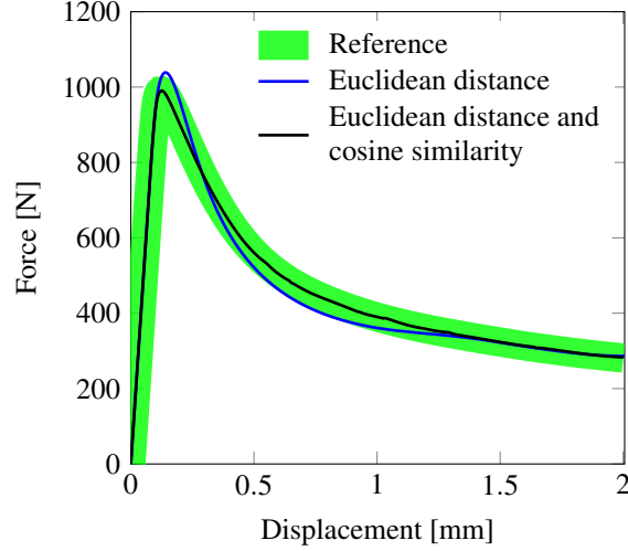
Figure 8: The effect of the distance metric on the load-displacement curves of the two-dimensional strain localization problem (reference solution: 1350 DOFs, 196 element; reduced order model: 227 POD basis vectors associated with the displacement field and LDEIM with 5 clusters and 19-10-9-9-9 DEIM entries in each cluster).
