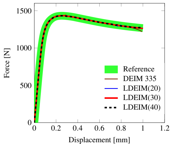
Figure 12: Footing: load-displacement curves associated with different number of clusters (reference solution: 5184 DOFs, 1331 elements; reduced order model: 609 POD basis vectors associated with the displacement field for DEIM and LDEIM).
