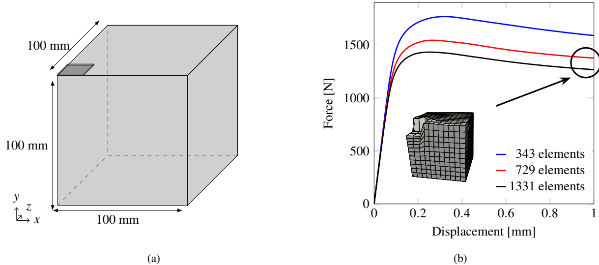
Figure 11: Footing: (a) geometry; (b) mesh refinement study.
