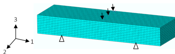
Figure 8. FE model of the short-beam specimen.
