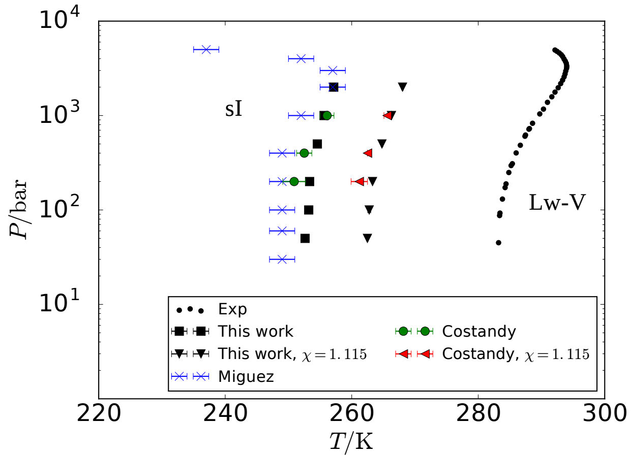
Figure 12: Three phase equilibrium points between sI hydrate (sI), liquid water (Lw) and gas vapor (V) for CO 2 hydrate, simulated using TraPPE CO 2 40 and TIP4P/2005 39 water, together with experimental results 3,4 , and direct coexistence simulations from Costandy et al. 18 and Miguez et al. 17
