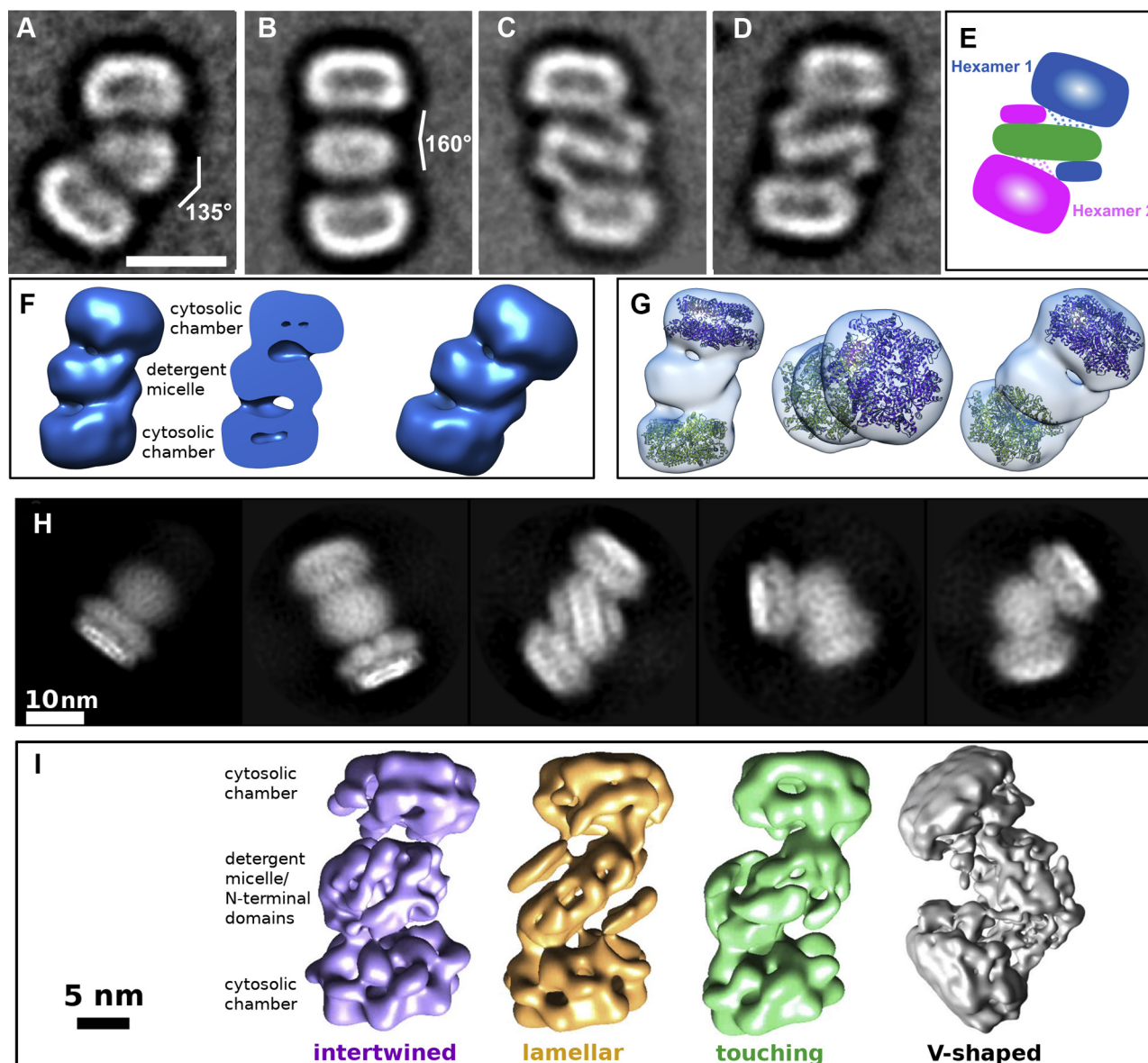
Figure 3. Class averages and 3D maps of FtsH dodecamers. A–D, class averages of the negatively stained specimen representing its typical side views. The scale bar represents 11 nm. E, schematic representation of the class averages highlighting with dashed lines six linking peptides present in the protein sequence. F, 3D maps and a cross section of different dodecameric conformations calculated from images of the negatively stained specimen. G, fitting of two cytosolic domains (PDB 4WW0) to the dodecamer map. H, cryo-EM class averages of the AaFtsH dodecameric specimen. Left to right: a hexamer side view, followed by four typical side views of a dodecamer. I, left to right: S-shaped FtsH dodecamers with variably intertwined N-terminal domains at resolutions of 17 Å (intertwined type), 19.5 Å (lamellar type), and 20.5 Å (touching type), respectively, and a V-shaped dodecamer at 12.3 Å.
