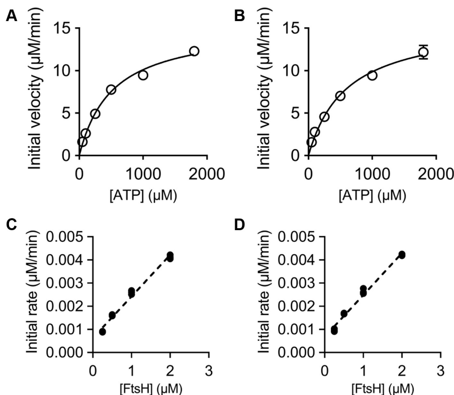
Figure 4. ATPase and protease activity assays. A–B, steady-state velocities for the ATP hydrolysis by 0.25 μM AaFtsH hexamers (A) and dodecamers (B). The average and SD of three replicas for each reaction are plotted (SD bars are not visible for some points owing to their small sizes). C–D, initial velocities of proteolysis of 50 μM resorufin-labeled casein by AaFtsH hexamers (C) and dodecamers (D) as a function of AaFtsH concentration. All the reactions were measured three times and all points are plotted.
