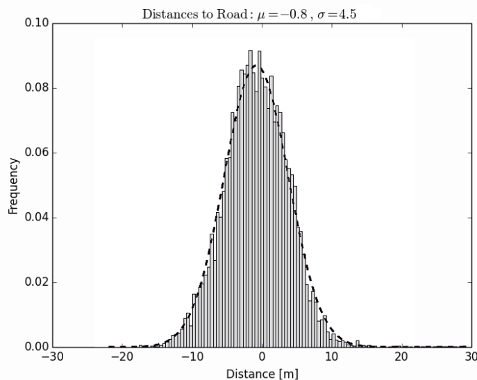
Figure 4: Histogram showing the distances from GPS points to the center line of the road including the fitted normal distribution.
