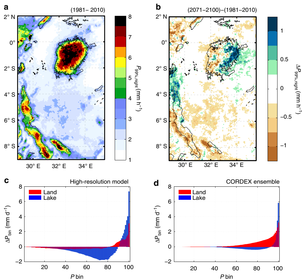
Figure 2 | Projected end-of-century changes in extreme precipitation over Lake Victoria. (a) Night-time 99th percentile precipitation ( P_{99\%,night} , 00:00 to 9:00 UTC) and (b) its projected future change from the high-resolution COSMO-CLM 2 model. (c,d) 24 h Lake (blue bars) and surrounding land (red bars) binned precipitation change ( P_{bin} ) from COSMO-CLM 2 and the ensemble mean of nine CORDEX-Africa members, respectively. The red rectangle in Supplementary Fig. 1 includes the land pixels considered as surrounding land. All changes are between time periods 1981–2010 and 2071–2100 under RCP8.5.
