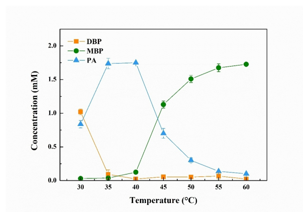
Figure 2. Selectivity of the DBP hydrolysis into MBP and PA at different temperatures. Reaction conditions: total reaction volume: 1 mL (10 mM phosphate buffer, pH 7); [DBP]_0 = 2 mM (40 \mu L of a 50 mM stock solution in DMSO), [EstJ6] = 1 \mu M, [P8219] = 2 \mu M, t = 3 h, 500 rpm. Negative controls that did not contain enzymes were carried out and no MBP or PA was detected.
