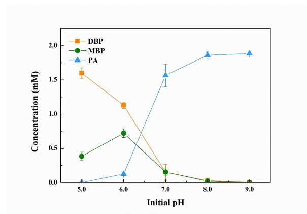
Figure 3. Effect of initial pH on the cascade reaction. Reaction conditions: total reaction volume: 1 mL (10 mM phosphate buffer); [DBP]_0 = 2 mM (40 \mu L of a 50 mM stock solution in DMSO), [EstJ6] = 1 \mu M, [P8219] = 2 \mu M, T = 40^\circ\text{C} , t = 3 h, 500 rpm. Negative controls that did not contain enzymes were carried out and no MBP or PA was detected.
