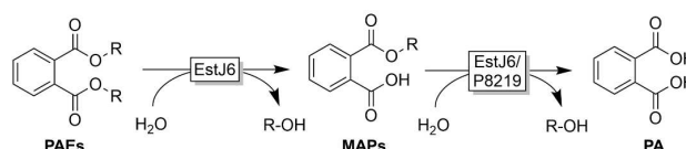
Scheme 1. Proposed biezymatic cascade for the complete hydrolysis of phthalic acid esters (PAEs) to phthalic acid (PA) via the monoalkyl phthalates (MAPs) catalyzed by the hydrolases EstJ6 and P8219.
