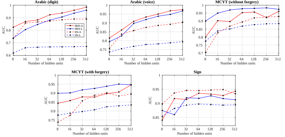
Figure 5.2: Area under the receiving-operator curve curve (AUC) of our two variants of Siamese Recurrent Networks (SRN-A and SRN-L) on five datasets as a function of the number of hidden units (higher is better). For reference, the performance of SRNs without recurrent connections (SNs) is also shown. All results were obtained by averaging over five repetitions. The standard deviation of the results is typically smaller than 0.01.
