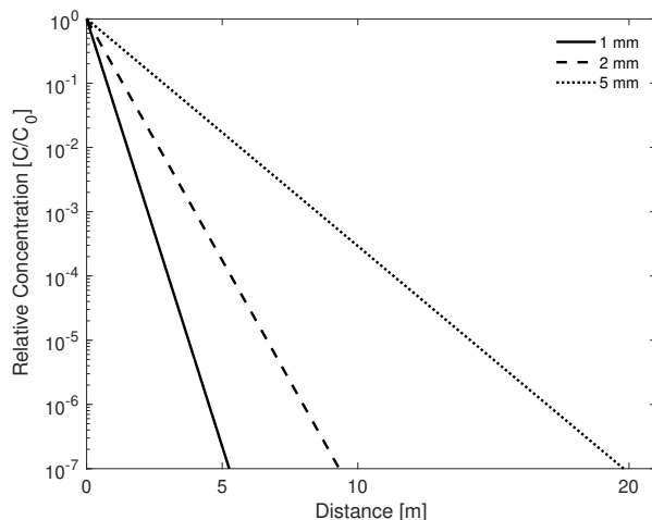
Figure 2.2.: Hypothetical case of DNACol for various collector grain sizes (Darcy velocity = 300 \text{ m y}^{-1} ; sticking efficiency = 0.59; other parameter values: see a print-out of the calculation in the Appendix A.3.
