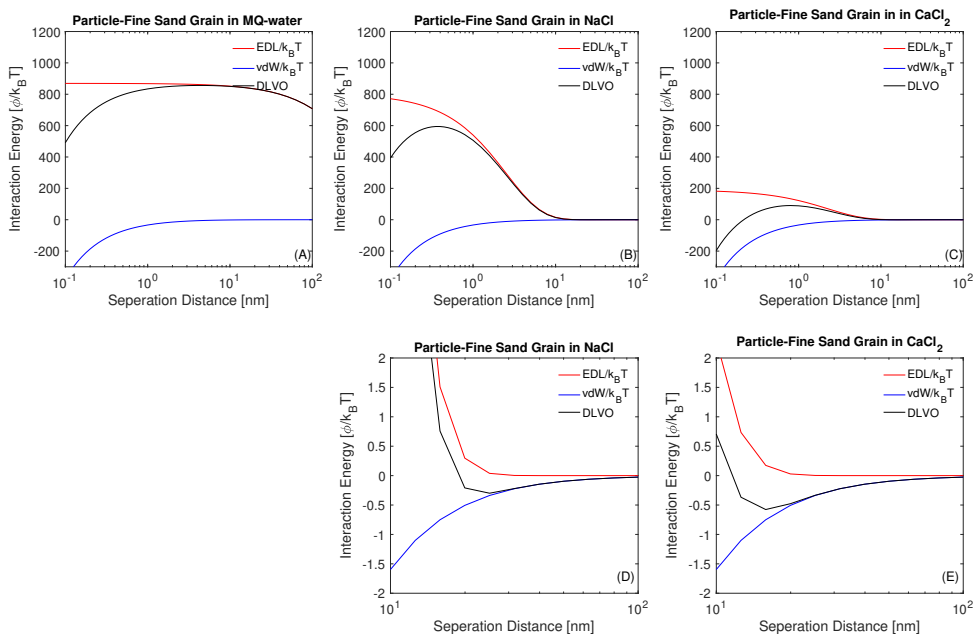
Figure A.4.: Calculated DLVO interaction energy profiles for the DNA-silica particle and fine sand grain system in Milli-Q water (A), NaCl solution (B), and in \text{CaCl}_2 solution (C). Bottom panels (D), and (E) show parts of panels (B), and (C), respectively, zoomed-in on the secondary minimum.
