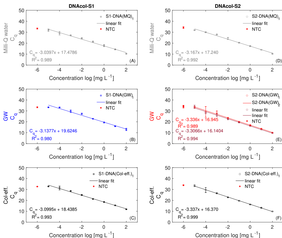
Figure C.2.: Calibration curves (DNACol) in various solutions, along with linear-regression fits (lines). The negative control values (NTC= No Template Control) of samples are presented by red symbols. Error bars indicate the standard deviation of triplicate qPCR samples. The background solutions of DNACol (S1) experiments are: (A) Milli-Q water, (B) Tulip groundwater, (C) Column effluent. The background solutions of DNACol (S2) experiments are: (D) Milli-Q water, (E) Tulip groundwater, (F) Column effluent.
