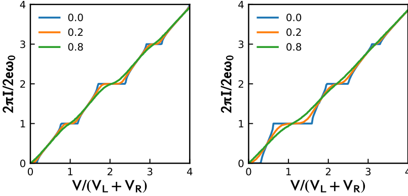
Figure 5.12: Smoothing of current plateaux at finite temperature. I-V characteristics of symmetric setup under gate voltage modulation with \omega = \omega_0 at dimensionless temperatures \tilde{T} shown in the labels. Left: strong coupling regime, \tilde{C} = 0.2 , q_0 = \pi/2 , the induced charge modulation A = 6 . Left: weak coupling regime, \tilde{C} = 50 , the voltage gate modulation A = 100 with q_0 = \pi/2 . At the same temperature, the degree of smoothing is bigger for the plateaux of smaller width. The same degree of smoothing in the weak coupling regime occurs at twice smaller temperature as compared with the strong coupling regime.
