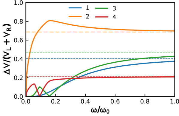
Figure 5.5: The frequency dependence of the plateau width for several integer plateaux (see the labels). Strong coupling regime \tilde{C} = 0.2 , q_0 = \pi/2 , symmetric setup, the gate charge amplitude A = 2\pi . The high-frequency limits (Eq. 5.18, 5.60) are given by dashed lines. The high-frequency approximation given (formula 5.18) is given by dashed lines. We see that the limit is achieved at \omega \approx \omega_0 for all plateaux. The width is the high-frequency approximation is valid for all steps. The width decreases to zero at lower frequencies, with some non-monotonous Bessel-like dependence.
