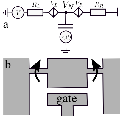
Figure 5.1: Two phase slip junctions in series in resistive environment coupled to a capacitor in between where the gate voltage is applied.
