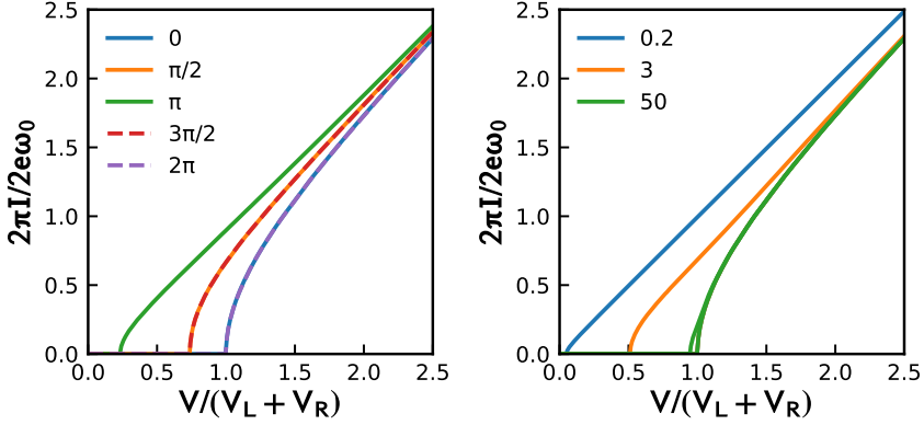
Figure 5.2: I-V characteristics in stationary regime. Symmetric setup, R_L = R_R , V_L = V_R . Left: Intermediate coupling, \bar{C} = 1 . The labels give the gate-induced charge q_0 . The Coulomb blockade threshold is modulated by q_0 , but does not vanish at q_0 = \pi owing to finite \bar{C} . Right: I-V characteristics for q_0 = 0, \pi and three different \bar{C} shown in the labels. The curves collapse at q_0 , which is the peculiarity of the symmetric setup. The minimum threshold approaches the maximum one upon increasing \bar{C} manifesting the weak coupling regime.
