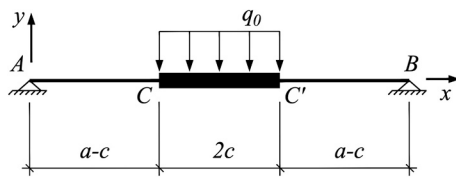
Fig. 6. Nonlinear beam strip model.
