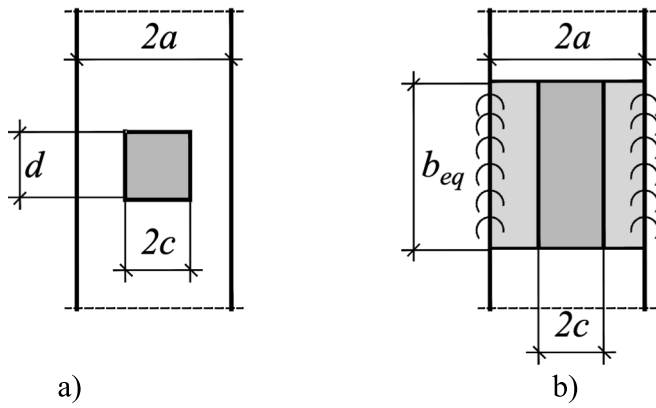
Fig. 5. Definition of the equivalent beam strip: a) real plate subject to patch loading; b) equivalent beam strip.
